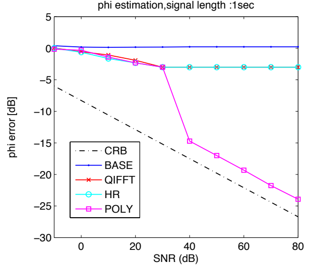
Figure 3.10: CRB : S_1 - \phi_0 - (1sec)
