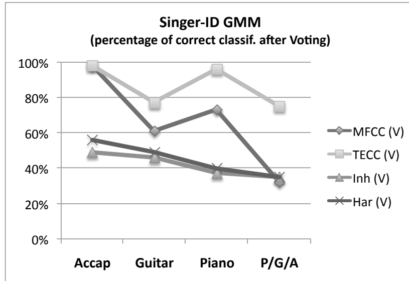
Figure 5.9: Classification accuracy for various accompaniment after majority voting
