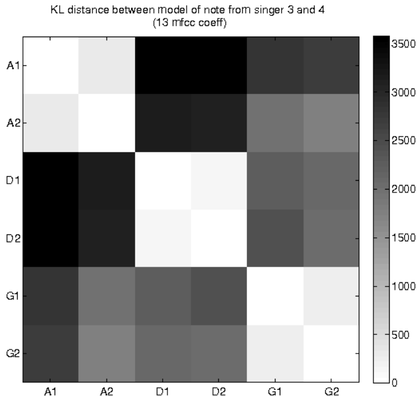
Figure 6.5: Distance between note-model for 2 singers with MFCC
