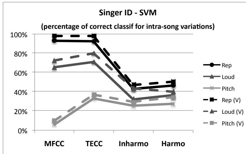
Figure 6.3: Classification accuracy for pitch and loudness variations for SVM. Results obtained after voting (V) are plotted with dashed lines
