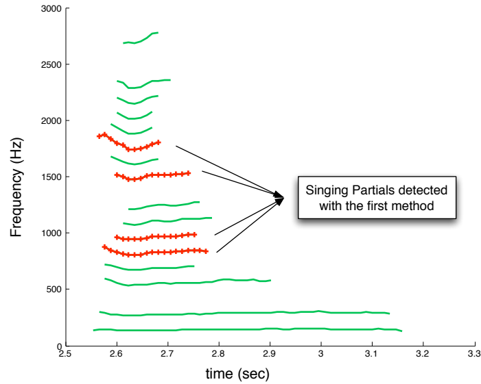
Figure 5.4: Comparison of the basic and improved method for vocal partial detection
