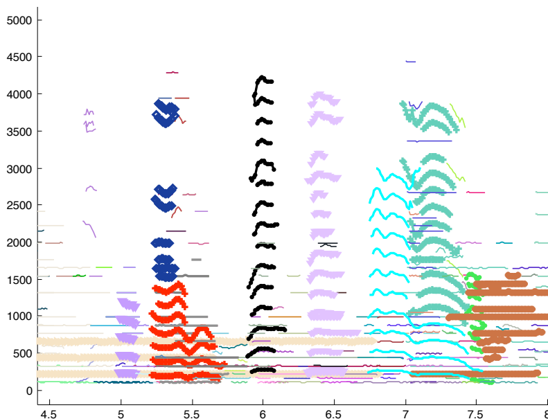
Figure 5.3: Example of partial clustering obtained on a real signal: voice + piano
