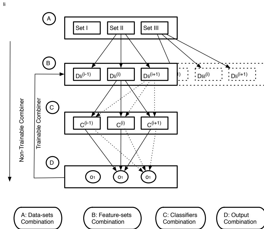
Figure 3.5: Level of combination
