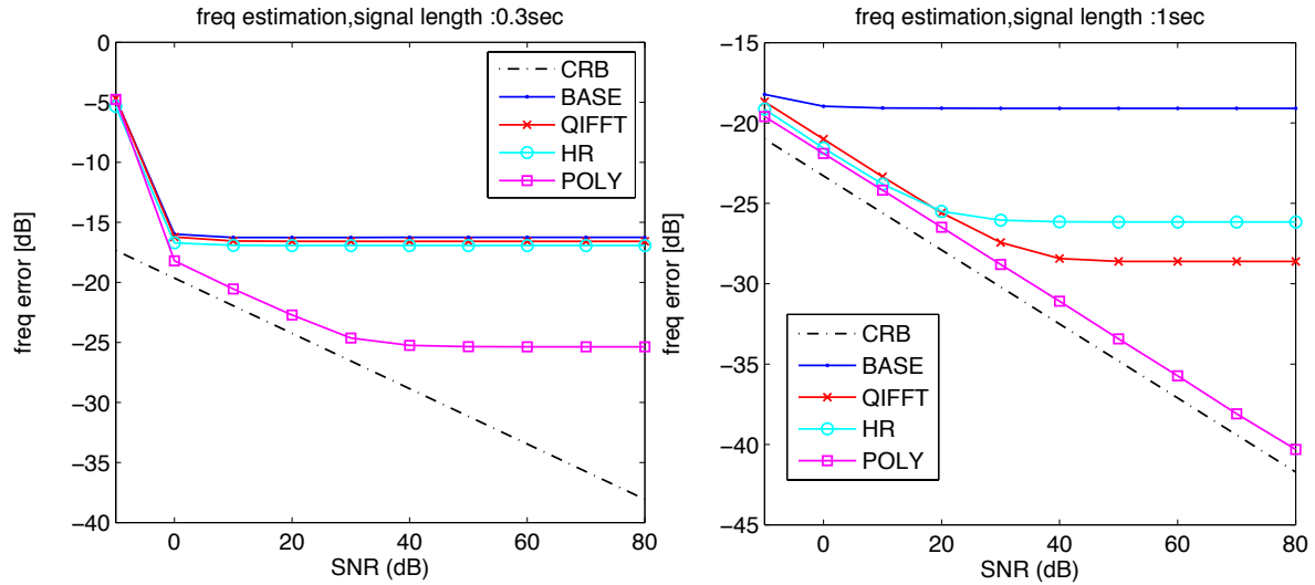
Figure 4.3: CRB : S1 - frequency - (0.3sec)
