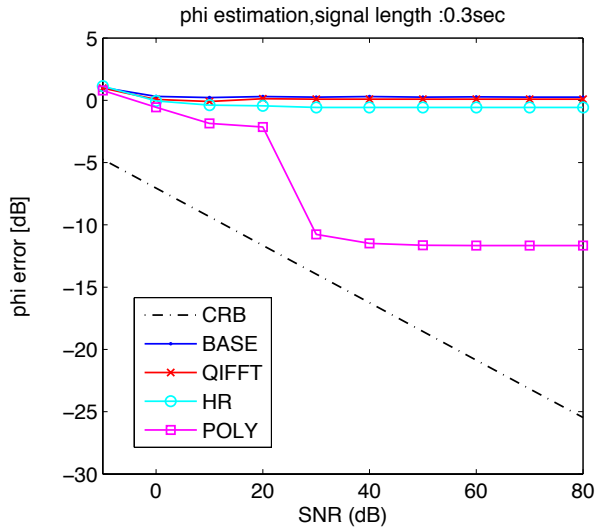
Figure 4.9: CRB : S_1 - \phi_0 - (0.3sec)
