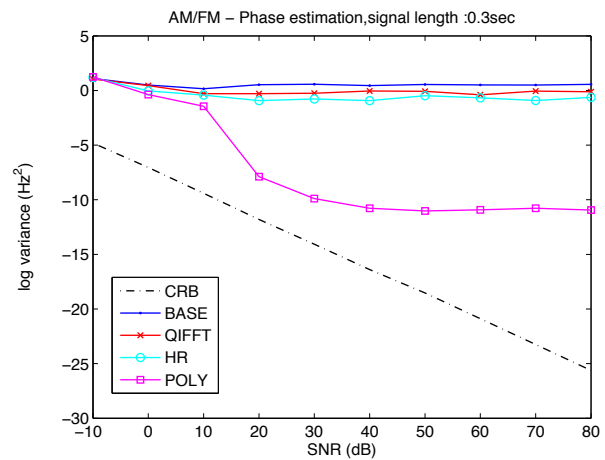
Figure 4.17: CRB - S2 - \phi_0 - (0.3sec)
