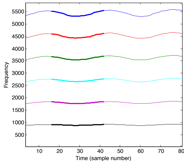
Figure 4.22: Frequency trajectories of the six first partials.
