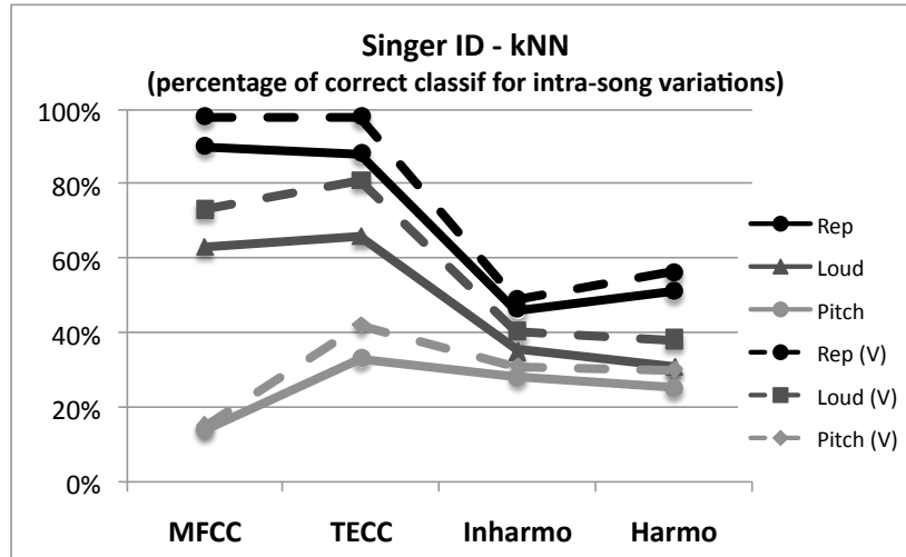
Figure 6.4: Classification accuracy for pitch and loudness variations for kNN. Results obtained after voting (V) are plotted with dashed lines
