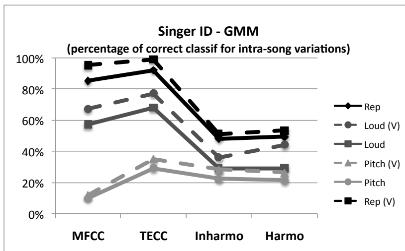
Figure 6.2: Classification accuracy for pitch and loudness variations for GMM. Results obtained after voting (V) are plotted with dashed lines
