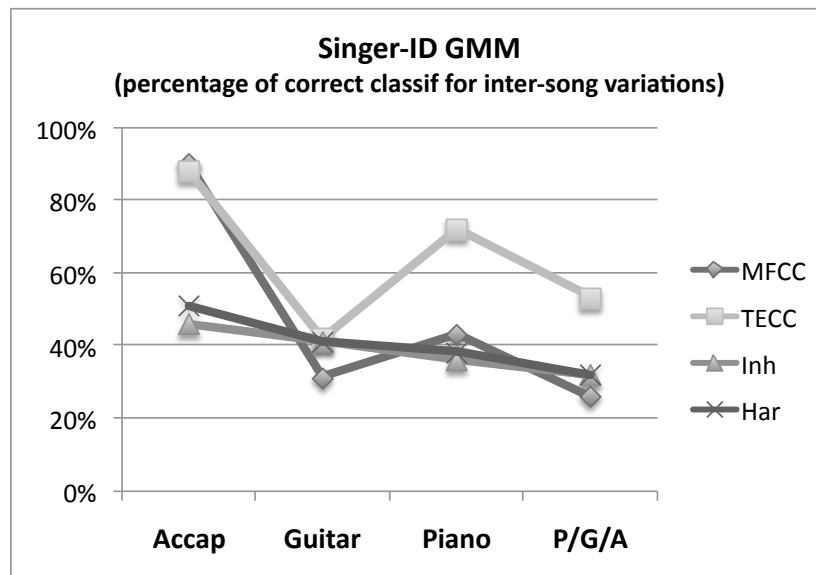
Figure 6.8: Classification accuracy for various accompaniment before majority voting
