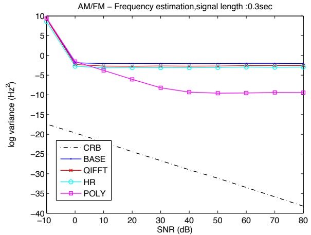
Figure 4.13: CRB - S2 - frequency - (0.3sec)
