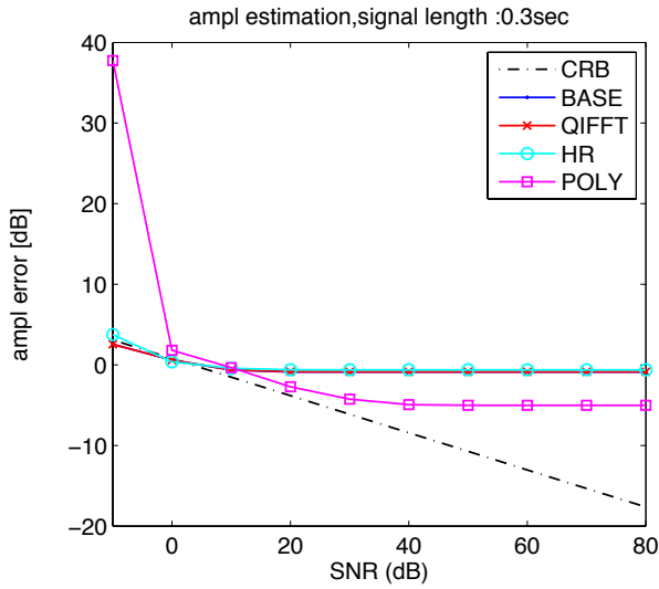
Figure 4.6: CRB : S1 - amplitude - (0.3sec)
