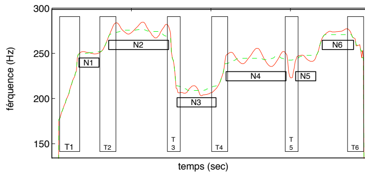
Figure 4.2: Fundamental frequency of a sung melody: Segmentation into sustained notes (N) and transitions (T)
