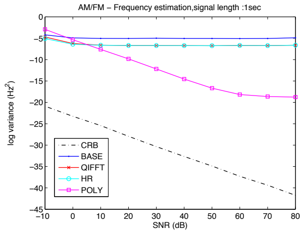
Figure 4.12: CRB - S2 - frequency - (1sec)
