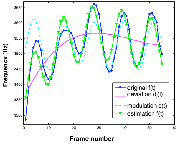
Figure 4.18: Estimation on a vibrated tone
