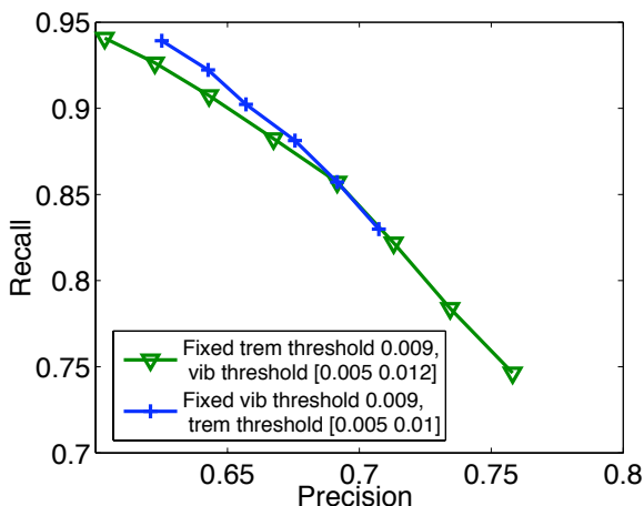
Figure 5.1: Examples of PR-curve obtained when varying one threshold
