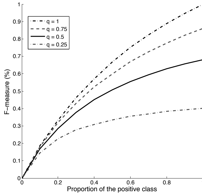
Figure 3.4: F_{measure} in function of the proportion of the positive class
