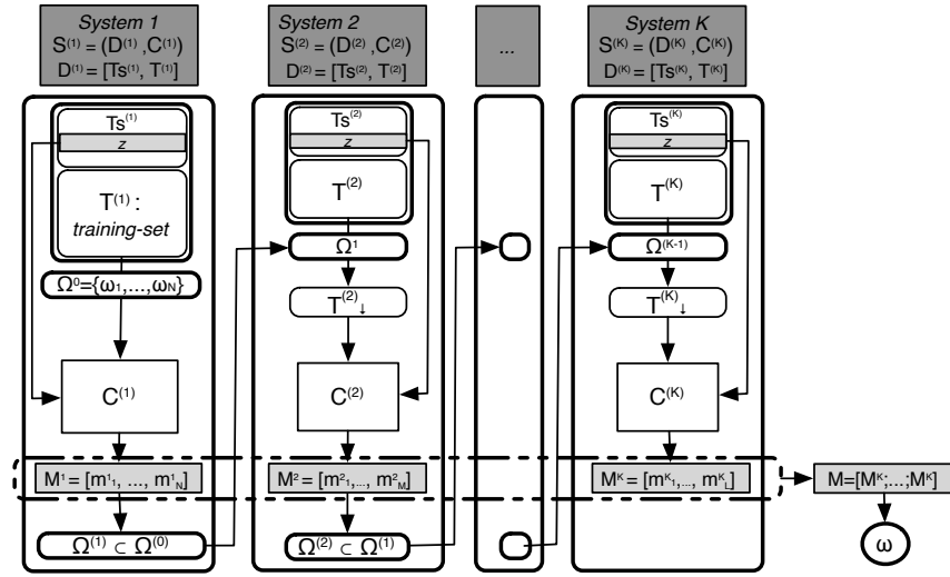
Figure 6.1: Scheme of the proposed method to combine K systems
