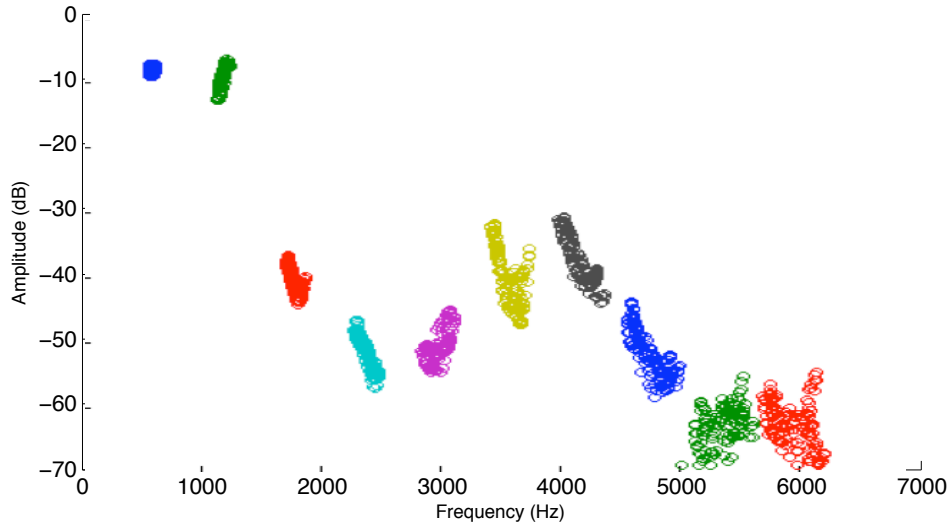
Figure 4.25: Samples of the vocal tract transfer function
