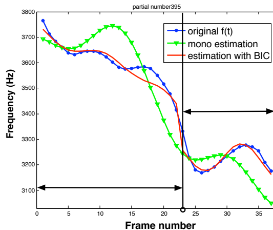
Figure 4.21: Vibrated notes linked + portamento
