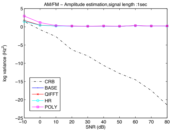
Figure 4.14: CRB - S2 - amplitude - (1sec)
