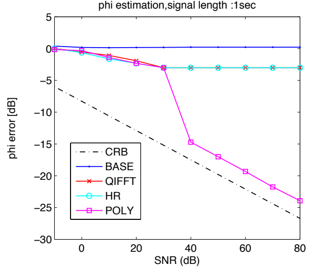
Figure 4.10: CRB : S_1 - \phi_0 - (1sec)
