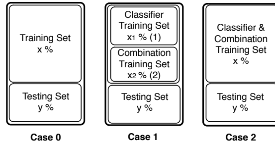
Figure 3.6: Possible data set reorganization to train class models and combination rules
