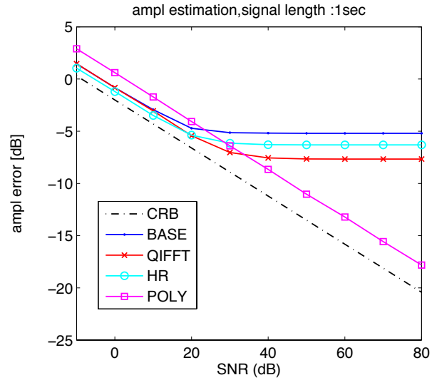
Figure 4.7: CRB : S1 - amplitude - (1sec)
