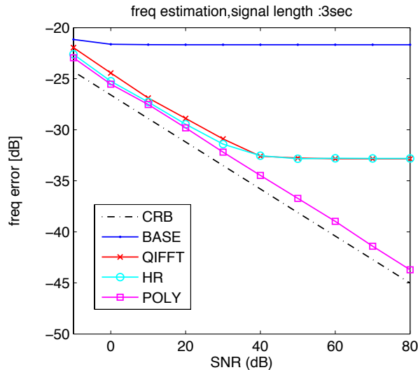
Figure 4.5: CRB : S1 - frequency - (3sec)
