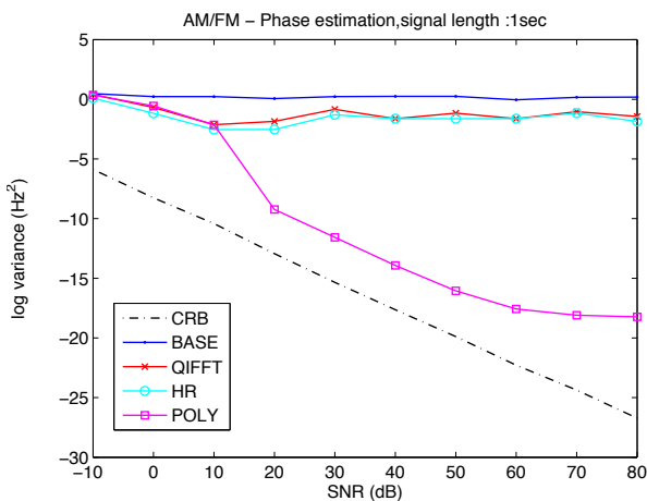
Figure 4.16: CRB - S2 - \phi_0 - (1sec)
