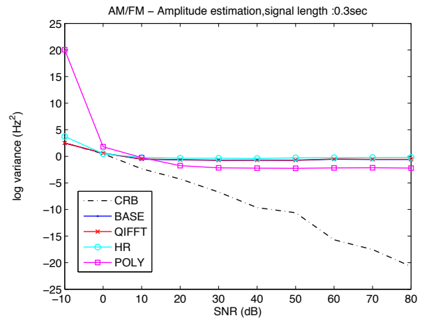
Figure 4.15: CRB - S2 - amplitude - (0.3sec)
