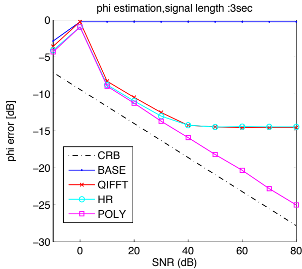
Figure 4.11: CRB : S_1 - \phi_0 - (3sec)
