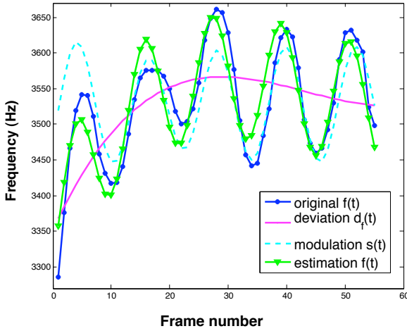
Figure 4.18: Estimation on a vibrated tone
