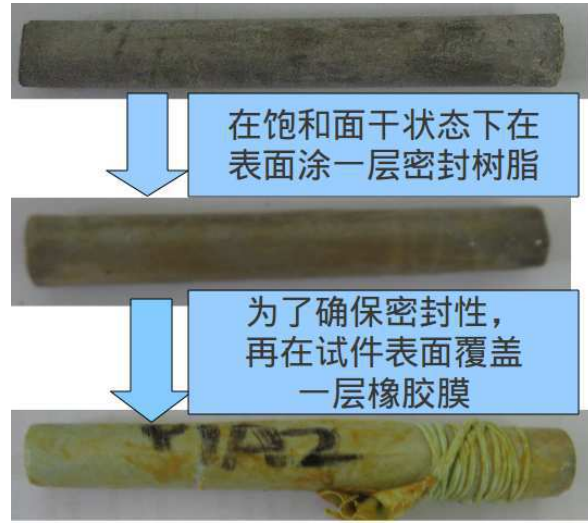
Figure 9.2: Preparation procedures of saturated cylindrical samples to obtain an undrained condition during freeze-thaw tests.
