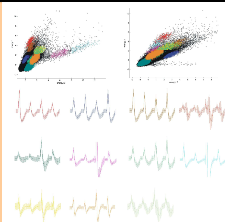
Figure 3.2.5: Example of spike sorting from one of our recorded tetrodes. The amplitude and waveform recorded on the four channels of a tetrode may be used to discriminate spikes from several cells. In this example, we recorded units from the pyramidal layer of CA1. In the top part of the figure, the amplitude of all spikes recorded on three of channels are plotted pairwise. The different colors refer to the putative single units (“clusters”) identified by the cluster discrimination program, and confirmed by the experimenter. This identification was based on PCA of these projection plots, as well as other projection plots involving the spike amplitude and other waveform parameters on the four channels. We identified 10 or 11 single cells from this recording (some uncertainty remains about two clusters (which ones?) with similar waveforms that may actually refer to the same cell). The bottom part of the figure shows the average waveforms on the four channels of the respective identified putative units.
