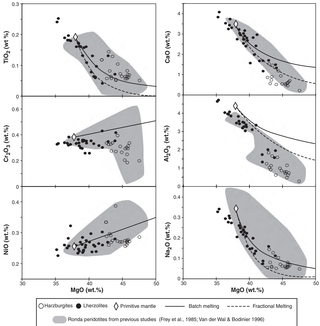
Fig. 8. Covariation diagrams for major (CaO, Al 2 O 3 ) and minor (Na 2 O, TiO 2 , Cr 2 O 3 , NiO) elements vs MgO (wt %) in the studied peridotites, compared with major- and minor-element compositions in the entire Ronda peridotite massif (Frey et al. , 1985; Van der Wal & Bodinier 1996) and with the evolution predicted by batch and fractional melting models (Gast, 1968; Shaw, 1970). Primitive upper mantle composition from McDonough & Sun (1995).
