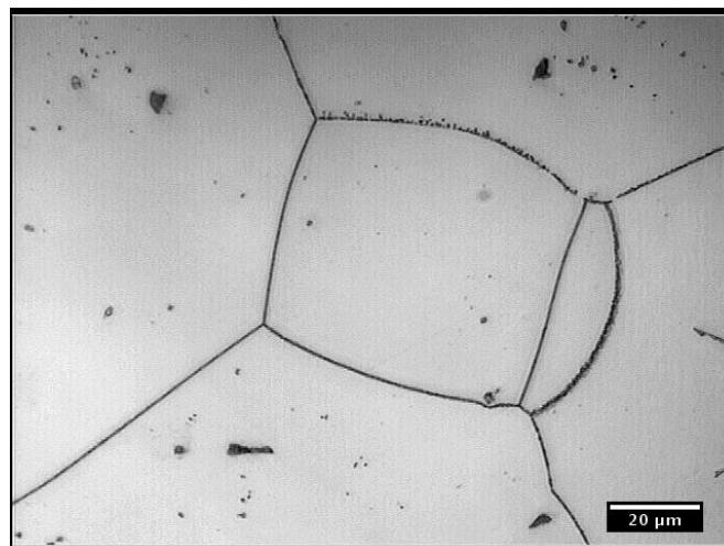
Figure 3.3: Light optical micrograph of a polished and etched cross-section through Beta21S after 1 hour at 790^\circ\text{C} . Layer-like \alpha precipitates are visible along the grain boundaries. The dark dots inside the grains are mostly inclusions.
