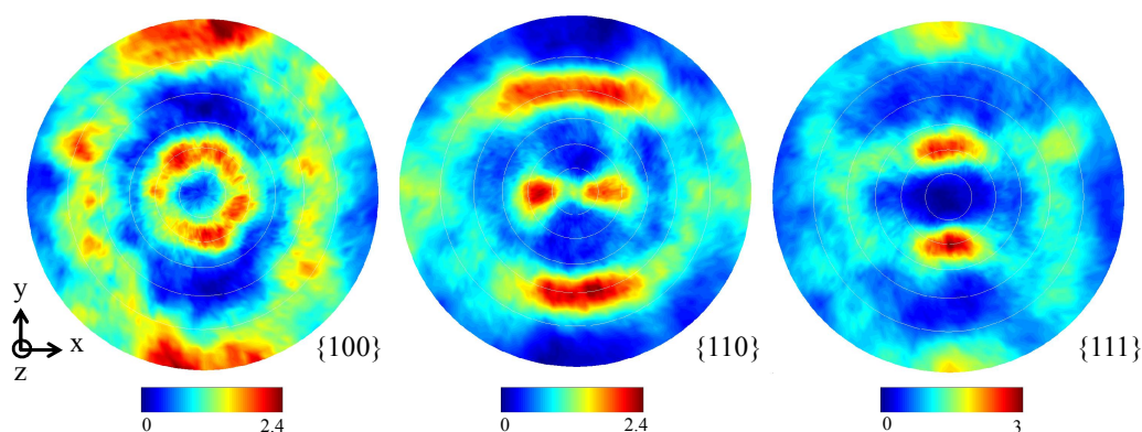
Figure 5.12: Pole figures showing micro texture of Beta21S [King et al., 2010].
