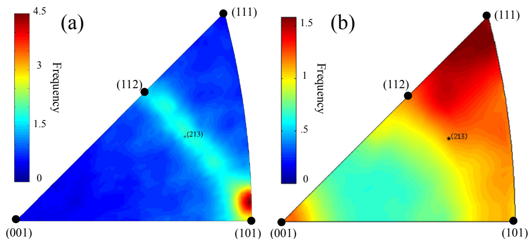
Figure 5.11: Crystallographic pole density distributions of the whole fracture surface in (a) VST5531 and (b) Beta21S.
