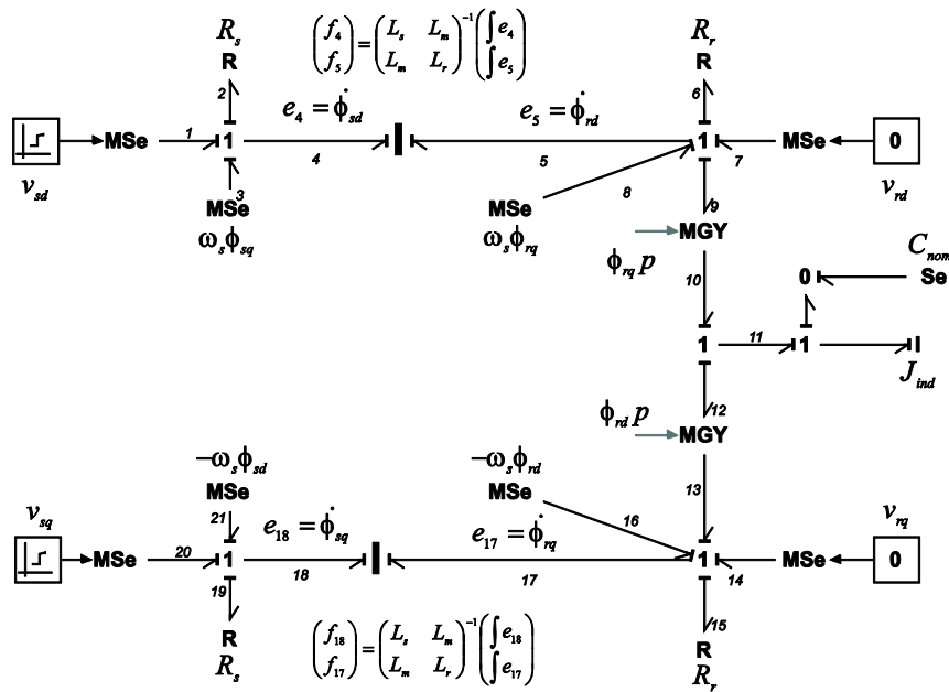
Figure 2.8 Bond graph de la machine asynchrone.
