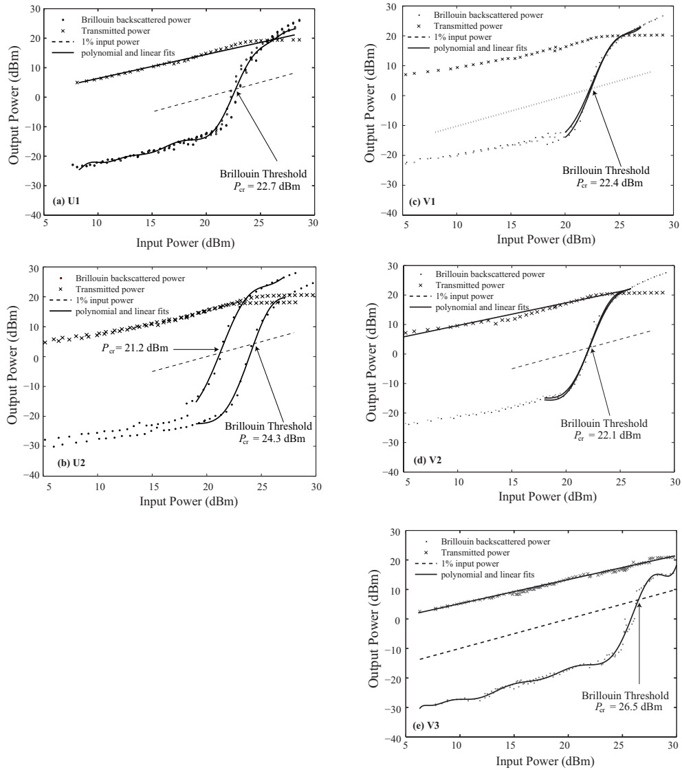
Figure 4.8: Experimental measurements of the Brillouin backscattered and transmitted powers through the periodically varying PCFs and the homogenous PCFs with similar micro-structure but without varying structure size. The Brillouin thresholds of the five PCFs are indicated by arrows for 1% fraction of the input power.
