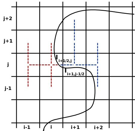
Figure 4.7: Decentered stencil: the discretization of the flux on point I_{i+1/2,j} involves grid point (i+1, j+2) instead of intersection point I_{i+1,j-1/2}
