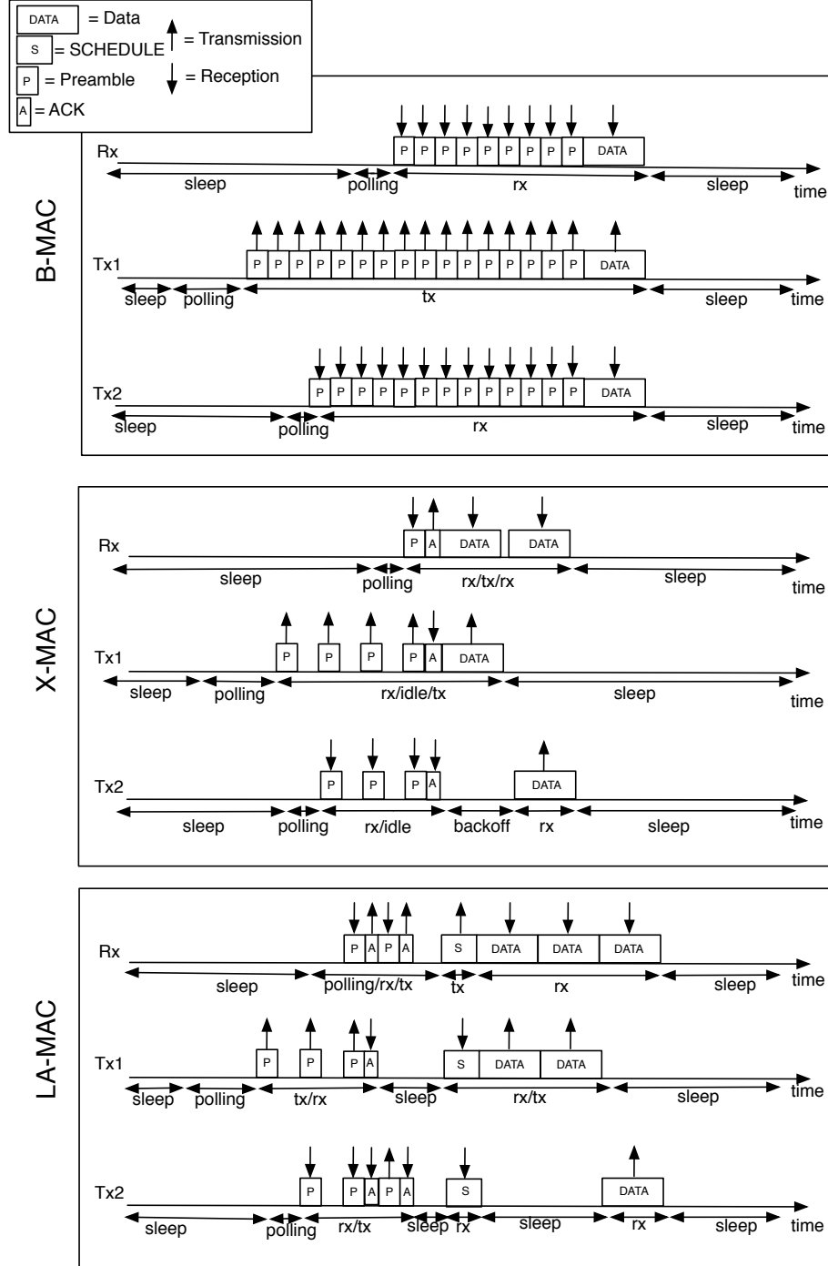
FIGURE 3.3 – Example of data frame transmissions with three preamble sampling MAC methods, B-MAC, X-MAC and LA-MAC.
