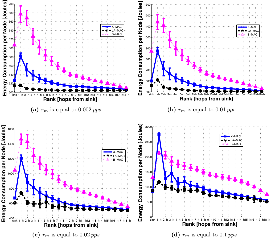
FIGURE 3.15 – Scenario 1, grid network with heterogeneous traffic. Energy consumption per node vs. the rank of nodes. There are 100 nodes are deployed in a regular 10x10 grid, alarm source has rank 10.
