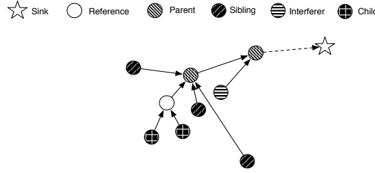
FIGURE 3.1 – Example of WSN showing the role of nodes.
