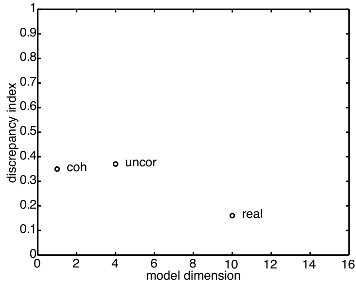
Figure 3.1 The discrepancy index vs. the model dimension for each noise model for the Rennes database.
