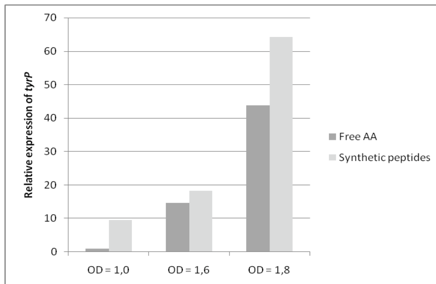
Figure 2: Relative expression of the tyramine transporter tyrP of L. plantarum IR BL0076 grown with free tyrosine or tyrosine containing peptides. Expression was measured at three different OD_{600nm} .
