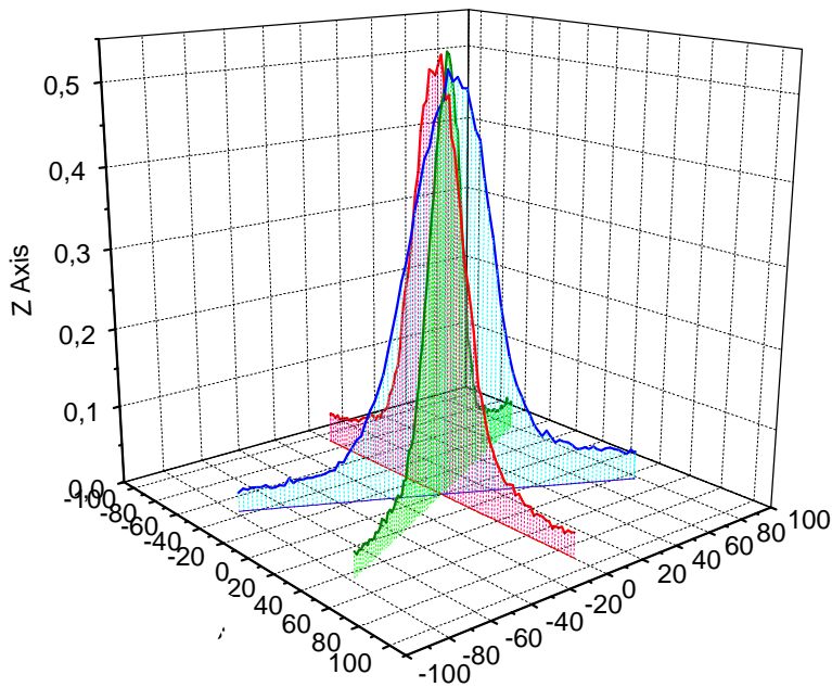
Figure II- 23 Angular diagram of a good SNOM tip
