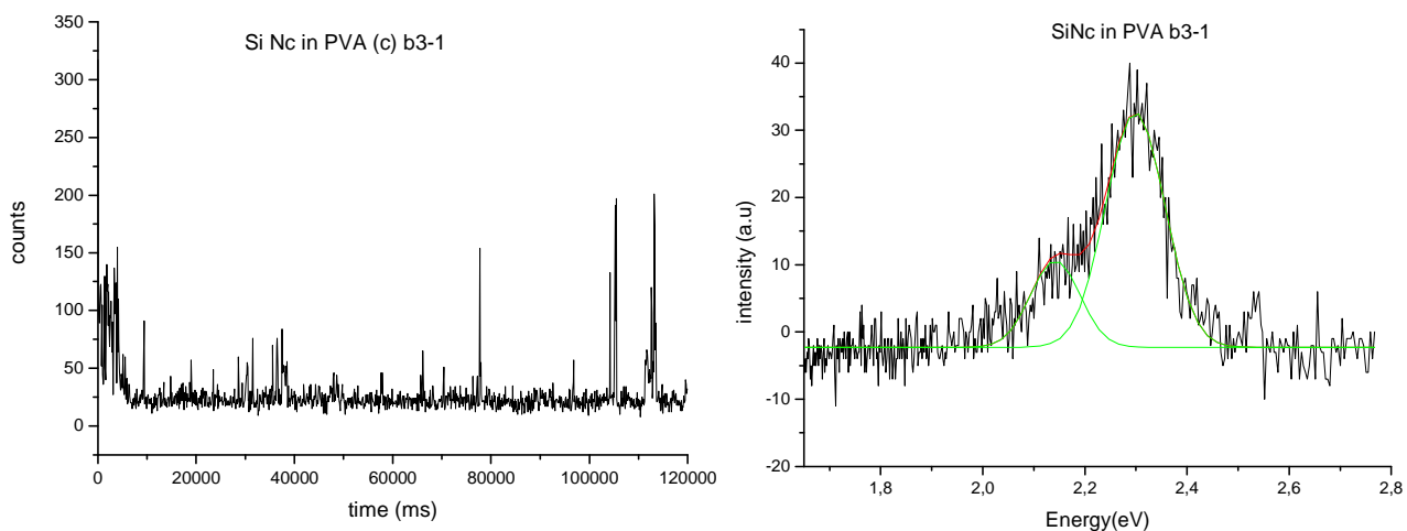
Figure IV- 22 Si nanocrystal in PVA sharped line time trace and corresponding emission spectrum.
