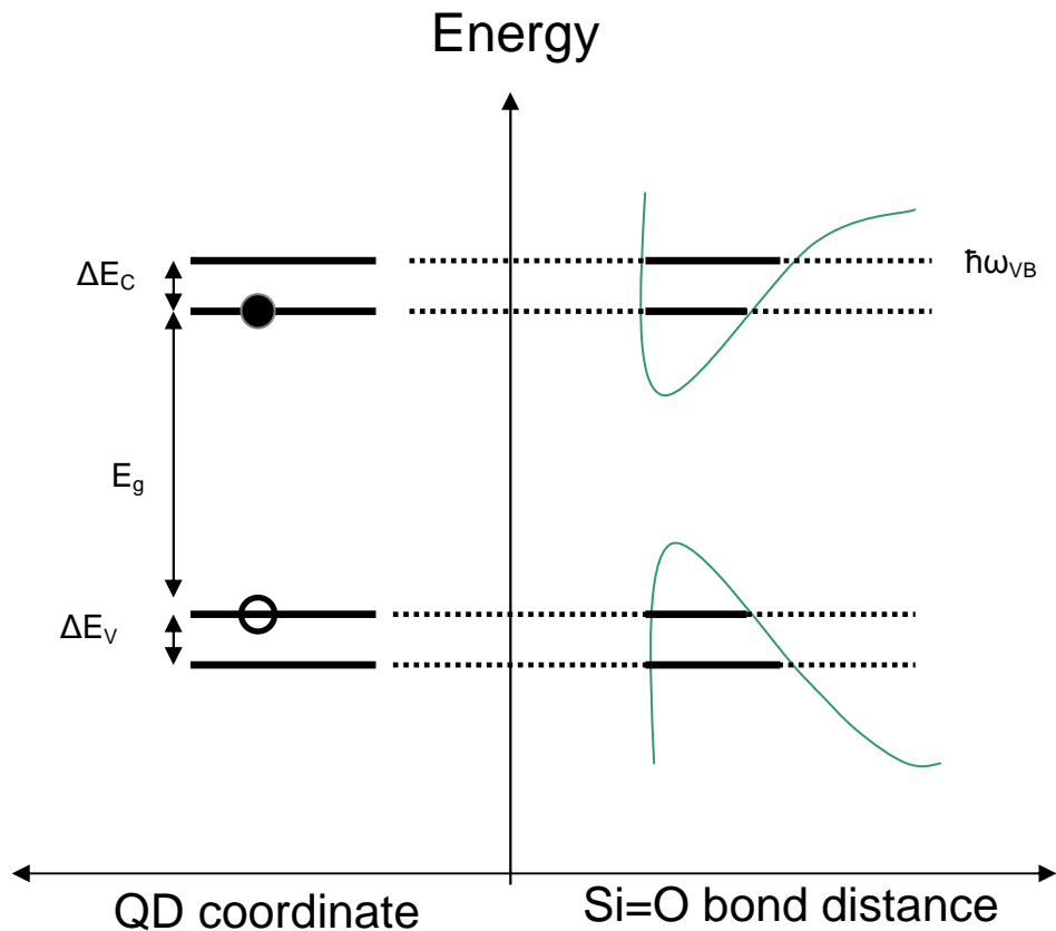
Figure IV- 18 quantized electronic levels of Si Nanocrystals and configuration space mode diagram for Si=O surface bonds. At left: \Delta E_c and \Delta E_v are the energy differences between lowest electronic sublevels of the conduction and valence bands. At right: Green lines represent the potential energy for surface vibrations (in the configuration space). The ground and first excited vibrational states are represented with the black lines. \hbar\omega_{VB} is the vibrational energy. When \hbar\omega_{VB} = \Delta E_c or \hbar\omega_{VB} = \Delta E_v , resonant coupling occurs.
