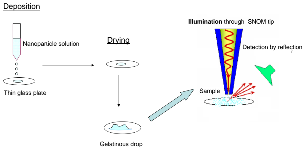
Figure III- 11 First sample preparation process for reflection mode SNOM imaging
