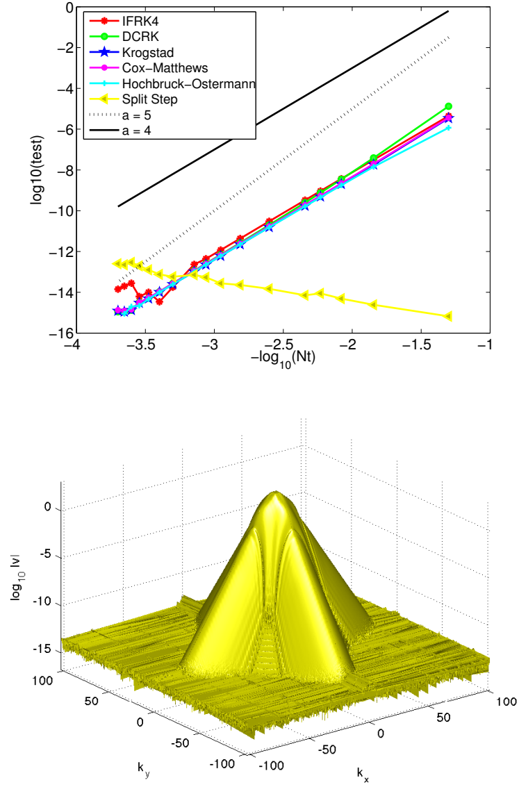
Figure 3.15: Non-conservation of the numerically computed L_2 -norm of the solution to the problem considered in Fig. 3.10 in dependence on the time step (top) and the Fourier coefficients for the final time (bottom).
