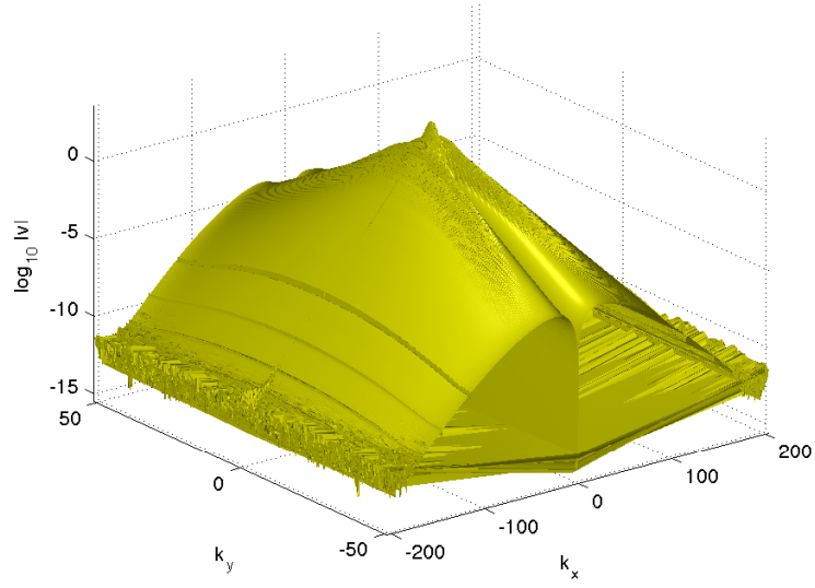
Figure 3.13: Non-conservation of the numerically computed L_2 -norm of the solution to the problem considered in Fig. 3.3 in dependence on the time step (top) and the Fourier coefficients for the final time (bottom).
