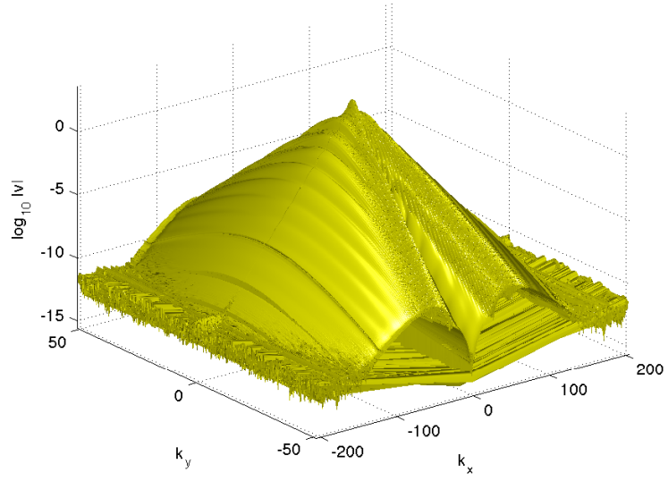
Figure 3.14: Non-conservation of the numerically computed L_2 -norm of the solution to the problem considered in Fig. 3.7 in dependence on the time step (top) and the Fourier coefficients for the final time (bottom).
