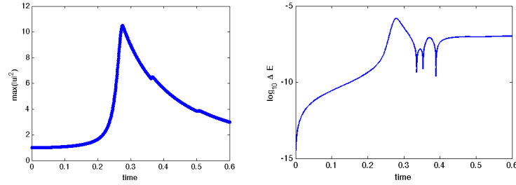
Figure 6.9: Time evolution of \max(|u|^2) and of the computed energy for an initial data of the form (6.2) with \eta = 0.1 .
