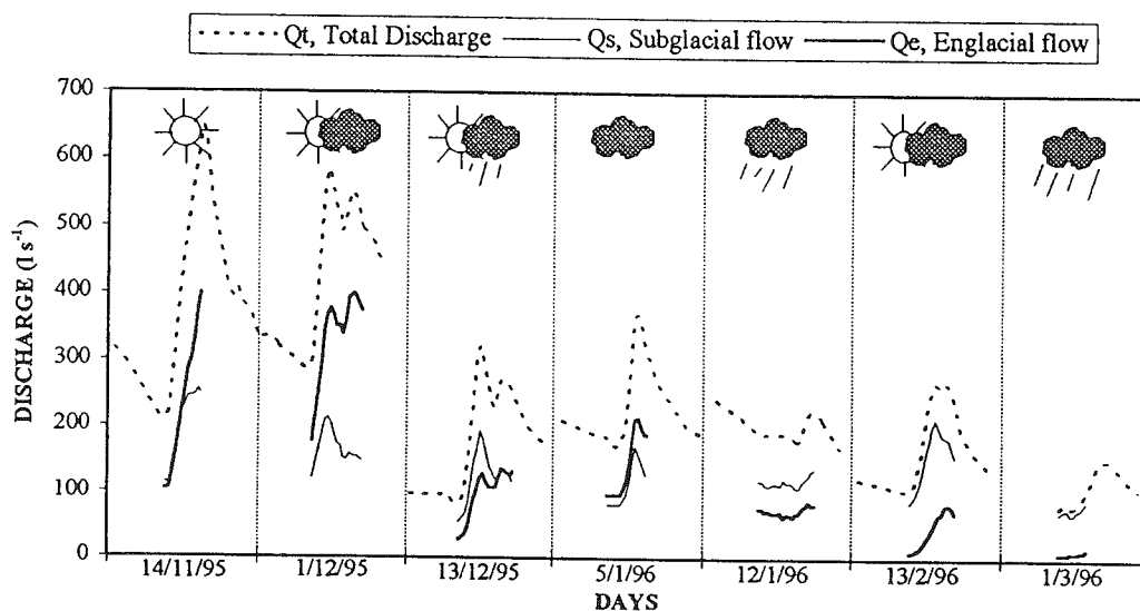
Figure 4. Total flow separation into englacial and subglacial components, at the limnometric station. Most of the water flowing in the proglacial stream comes from the englacial system, except during days of recession flow
