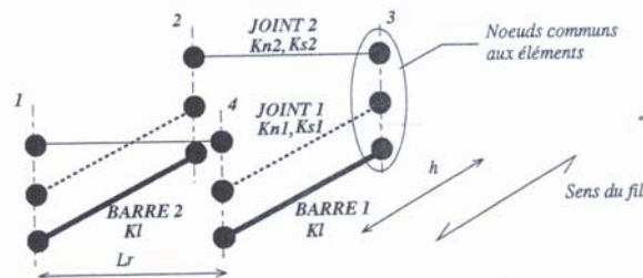
Figure B.5 : Ressorts élaborés [BOC 97]
