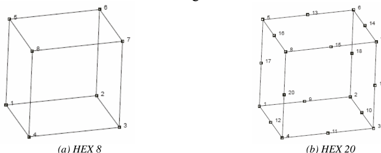
Figure B.16 : Éléments finis solides
