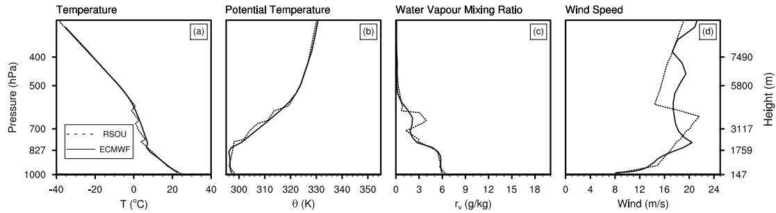
Figure 5.1: Comparison between the radiosonde data (dashed line) and the ECMWF analyses (solid line) for the Lançon-de-Provence 2005. The four graphics represent the vertical profile of: (a) temperature T ( ^{\circ}\text{C} ), (b) potential temperature \theta (K), (c) water vapour mixing ratio r_v (g/kg) and (d) wind speed (m/s).
