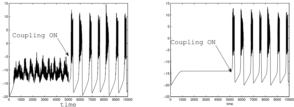
FIGURE 7.4: Mean membrane voltage of the active (left) and silent (right) population before and after the coupling between the two populations is switched on. After the coupling is activated, the system shows a global bursting oscillation even though no interconnections are present inside each neuronal population.
