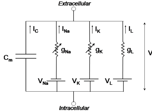
FIGURE 1.3: Electrical circuit equivalent to a model. C_m denotes the neuron membrane capacitance. V_{Na} and V_K are, respectively, the sodium and potassium equilibrium potential. The nonlinear conductances g_{Na} and g_K changes dynamically according to voltage changes. I_C = C_m dV/dt is the current at membrane capacitance. I_{Na} and I_K are the ionic currents generated by, respectively, sodium and potassium ions. The leak current I_L approximates passive properties of the cell. Adapted from (Skinner, 2006), with permission.
