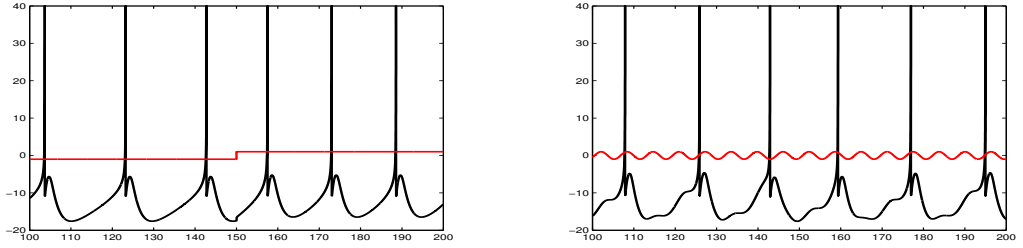
(b) Novel reduced model (6.15).
