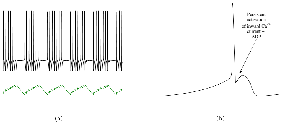
FIGURE 1.5: Bursting and ADP
