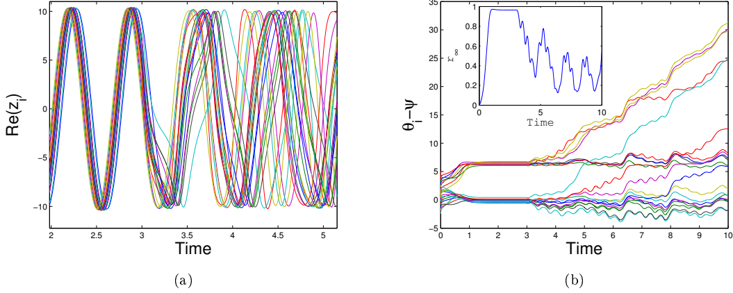
FIGURE 2.4: Large feedback gain and natural frequencies: full desynchronization.
