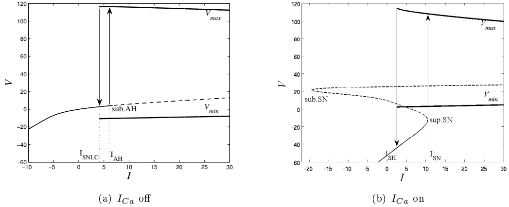
FIGURE 6.6: One parameter bifurcation diagram of the reduced Hodgkin-Huxley model with and without calcium current. Thin solid lines represents stable fixed points, while dashed lines unstable fixed points or saddle points. The thick lines labeled V_{min} and V_{max} represent, respectively, the minimum and the maximum voltage of limit cycles. (a): Hodgkin-Huxley model. (b): calcium-gated Hodgkin-Huxley model. I_x , with x = SNLC, AH, SH, SN , denotes the value of the input current for which the system undergoes the bifurcation x . See the text for more details.
