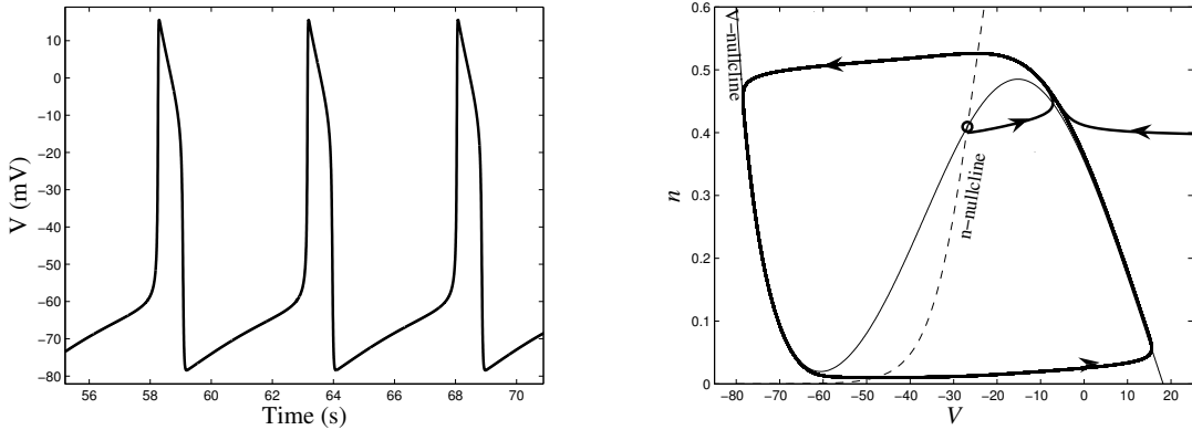
FIGURE 2.2: Periodic spiking and associated limit cycle in the I_{Na,p} + I_K model. Equations and parameters as in (Izhikevich, 2007, Figure 4.1)
