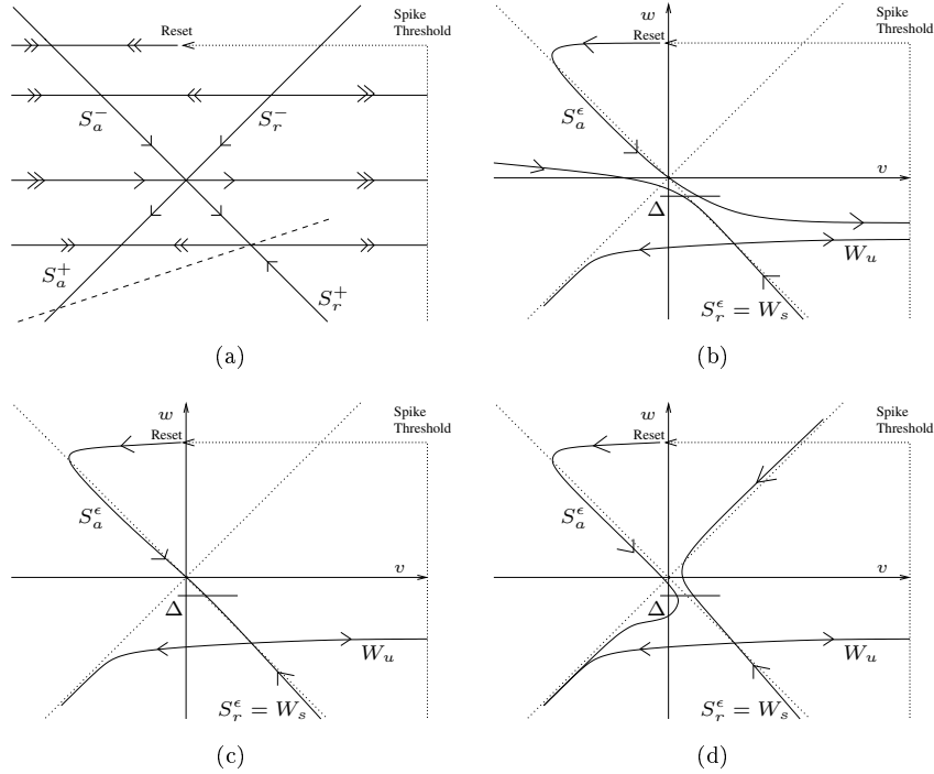
FIGURE 6.12: Phase-portrait of the hybrid dynamics (6.15) for different values of \epsilon and I . (a): Fast-slow dynamics for \epsilon = I = 0 . (b): Continuation of the slow manifolds for \epsilon > 0 and I > I_c(\sqrt{\epsilon}) , where I_c(\sqrt{\epsilon}) is defined as in Theorem 6.2. (c): Continuation of the slow manifolds for \epsilon > 0 and I = I_c(\sqrt{\epsilon}) . (d): Continuation of the slow manifolds for \epsilon > 0 and I < I_c(\sqrt{\epsilon}) .
