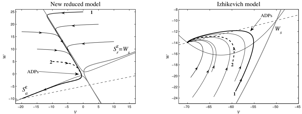
FIGURE 6.14: ADPs generation comparison in the proposed and in the Izhikevich hybrid models. Legend as in Figure 6.5. Parameters for the new reduced model (6.15) as in Figure 6.13, apart that here I = 1 . Equations and parameters for the Izhikevich model are provided at the end of the chapter
