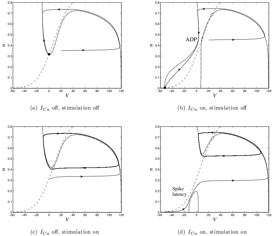
FIGURE 6.5: Phase portraits of the reduce Hodgkin-Huxley model with and without calcium current. The V -nullcline is drawn as a solid thin line, the n -nullcline as a dashed thin line. Trajectories are drawn as solid oriented lines. Black circles denote stable focus, black squares stable nodes, white circles unstable focus, and white square saddle points.
