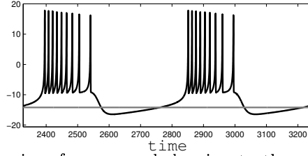
FIGURE 7.2: Typical behavior of a neuron belonging to the active population (black) and silent population (grey), before the diffusive coupling between the two populations is switched on.
