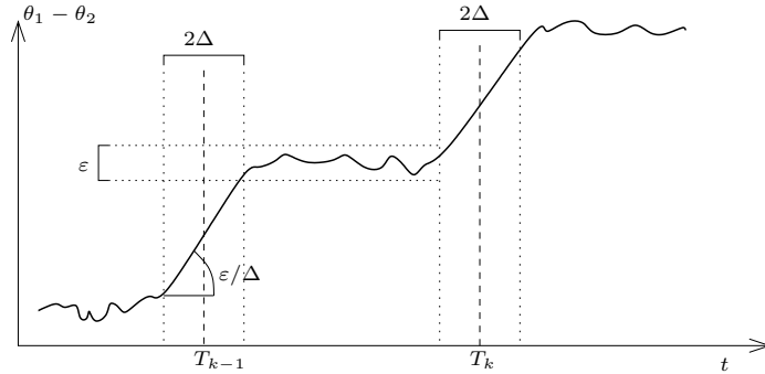
FIGURE 5.2: Time-course of the phase difference between two couple oscillators undergoing successive phase-slips on the intervals [T_k - \Delta, T_k + \Delta] . The constants \varepsilon, \Delta are defined in (5.11) below.
