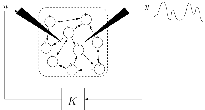
FIGURE 1.2: Proposed proportional mean-field feedback DBS control scheme. The mean electrical activity of a population of neurons, each modeled for simplicity as an oscillator, is recorder via a DBS electrode. This output is multiplied by a feedback gain and injected back in the neuronal population.
