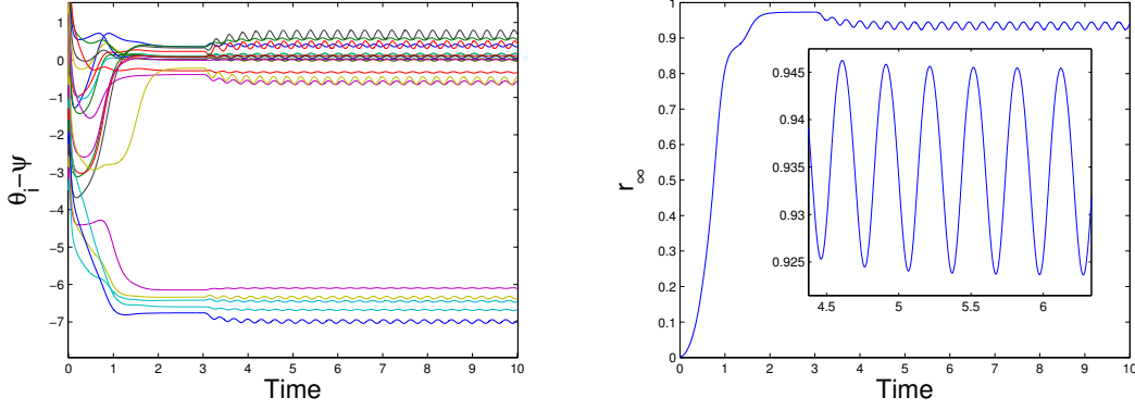
FIGURE 2.6: Small feedback gain: practical phase-locking.
