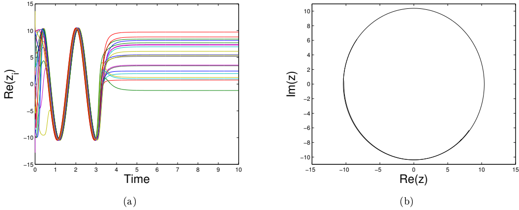
FIGURE 2.5: Large feedback gain and small natural frequencies: neuronal inhibition.
