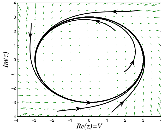
FIGURE 2.3: Limit cycle in the Landau-Stuart oscillator
