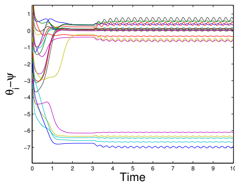
FIGURE 3.1: Practical phase-locking in Equation (2.3).
