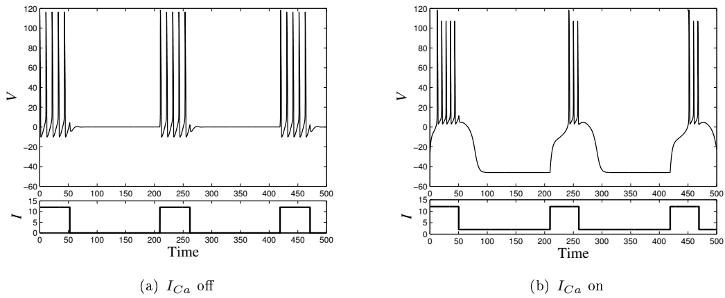
FIGURE 6.4: Exogenous bursting in the reduced Hodgkin-Huxley model with and without calcium current.
