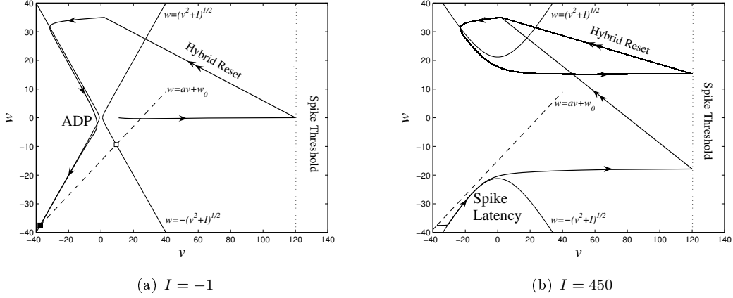
FIGURE 6.11: Simple model (6.15) with a = 0.6, c = 2, d = 35, w_0 = -15, v_{th} = 120 . exhibiting the same qualitative behavior of the calcium-gated Hodgkin-Huxley model. The legend for the phase-portrait is the same as Figure 6.5.
