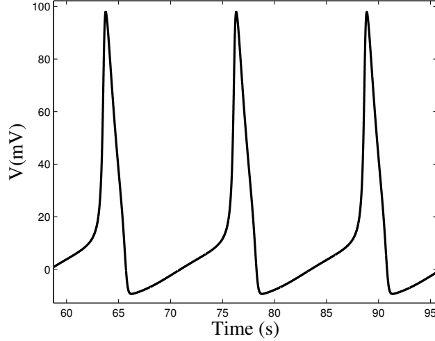
FIGURE 2.1: Periodic spiking in the Hodgkin-Huxley model. Equations and parameters as in (Hodgkin and Huxley, 1952).
