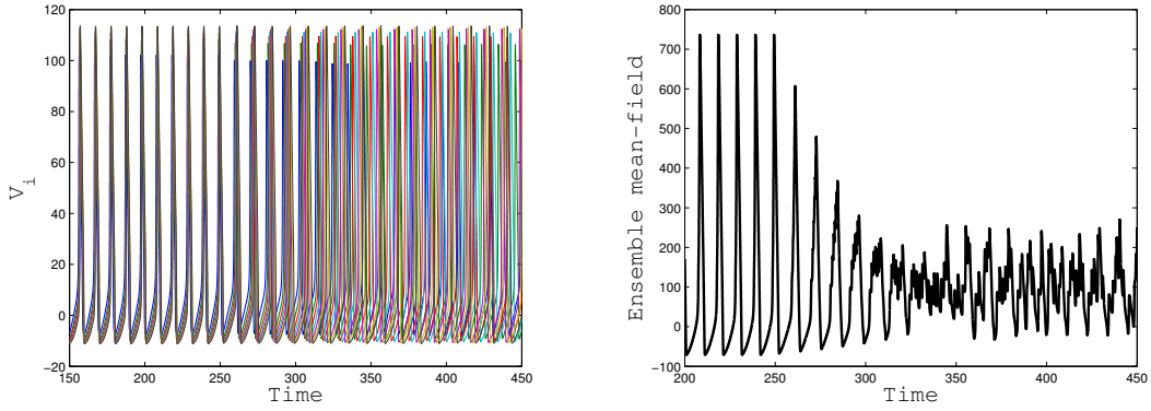
FIGURE A.4: Response of all-to-all coupled ( N = 7 ) Hodgkin-Huxley neuron model to proportional mean-field feedback. The feedback is switched on at t = 250 . Large natural frequencies: desynchronization. Left: voltages. Right: ensemble mean-field.
