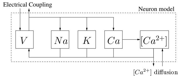
FIGURE 1.8: Input-output model of the neuron membrane. The membrane voltage interacts with the different ionic currents via parallel feedback loops. In turn, calcium currents change the intracellular Ca^{2+} concentration, providing a further slower feedback on the voltage dynamics (see Section 1.4.2, page 16). The interconnection with other neurons is due to electrical coupling and to the diffusion of Ca^{2+} ions in the extracellular medium. Other forms of internal and external interaction can similarly be modeled.
