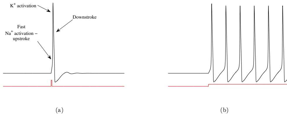
FIGURE 1.4: Neuronal excitability and periodic spiking
