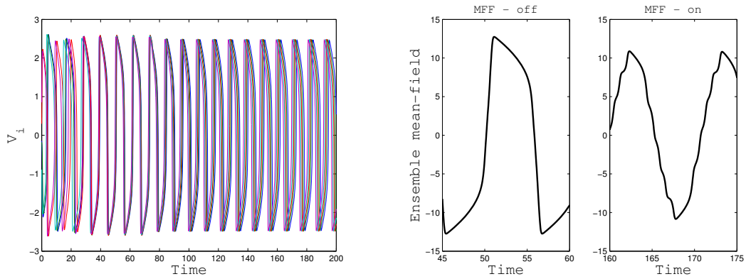
FIGURE A.2: Response of all-to-all coupled ( N = 5 ) Van der Pol oscillators to proportional mean-field feedback. The feedback is switched on at t = 50 . Small feedback gain: robust phase-locking. Left: voltages. Right: ensemble mean-field before and after the feedback is switched on.
