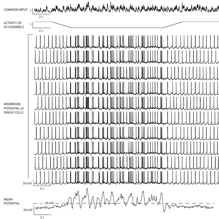
FIGURE 1.7: Response of an ensemble of heterogeneous dopaminergic neurons to a common noisy input. SK channels inhibit the calcium-regulated excitability, letting the neurons insensitive to the injected synaptic current and the ensemble desynchronized. When SK channels are downregulated, the ensemble is entrained by the exogenous current, resulting in a synchronous behavior. Adapted from (Drion et al., 2011b).
