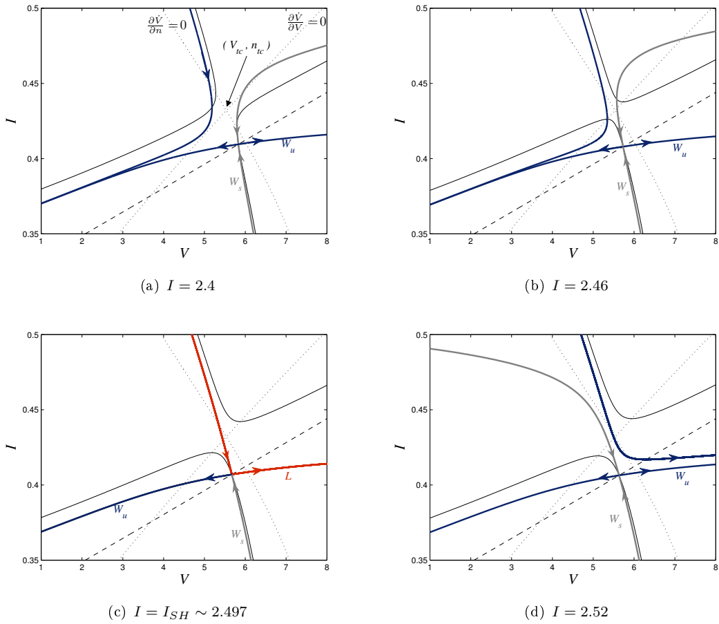
FIGURE 6.8: Phase portrait in the I_{C_a} -on configuration for different values of the input current. The V -nullcline is drawn as a solid thin line, the n -nullcline as a dashed thin line. W_s denotes the stable manifold of the saddle point, and W_u its unstable manifold. L denotes a saddle-homoclinic trajectory.
