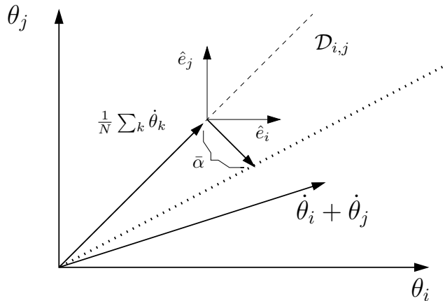
FIGURE 5.1: Geometric interpretation of desynchronization
