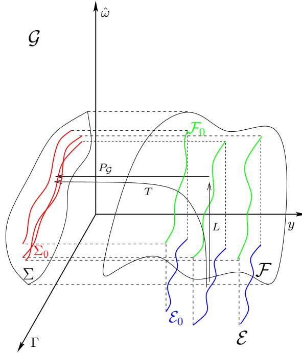
FIGURE 2.7: Construction of the smooth map T : \mathcal{E} \rightarrow \mathcal{G} .
