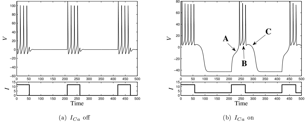
FIGURE 6.3: Exogenous bursting in the Hodgkin-Huxley model (6.4) with and without calcium current.
