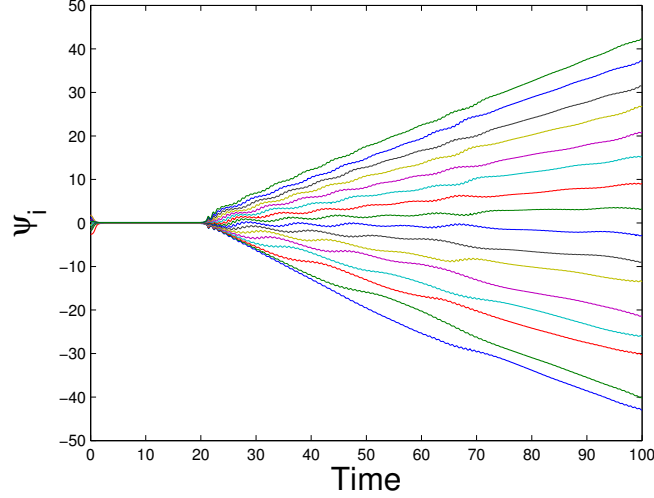
FIGURE 5.4: Evolution of the grounded dynamics of (5.18) for large natural frequencies when a proportional mean-field feedback with gain \gamma_0 = -k_0 is switched on at time t = 20
