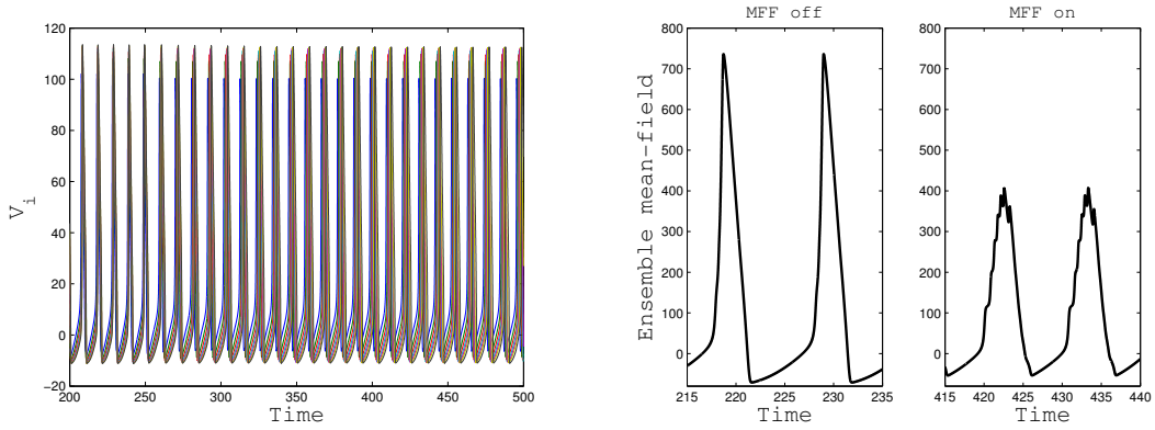
FIGURE A.5: Response of all-to-all coupled ( N = 7 ) Hodgkin-Huxley neuron model to proportional mean-field feedback. The feedback is switched on at t = 250 . Small feedback gain: robust phase-locking. Left: voltages. Right: ensemble mean-field before and after the feedback is switched on.
