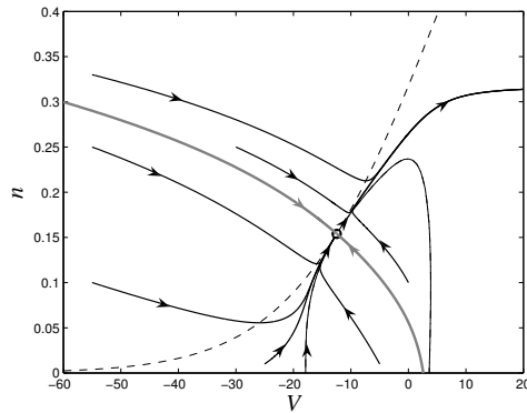
FIGURE 6.7: Saddle-node in the reduced Hodgkin-Huxley model with calcium current for I \sim I_{SN} . The gray thick trajectory depict the stable manifold of the saddle-node.
