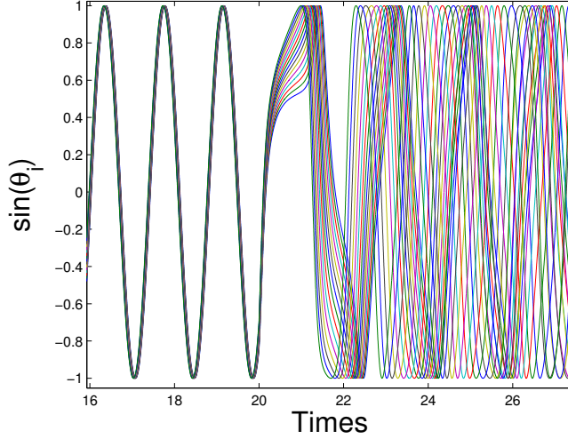
FIGURE 5.3: Evolution of the phases of (5.18) for large natural frequencies when a proportional mean-field feedback with gain \gamma_0 = -2k_0 is switched on at time t = 20 . The mean-field feedback induces desynchronization.
