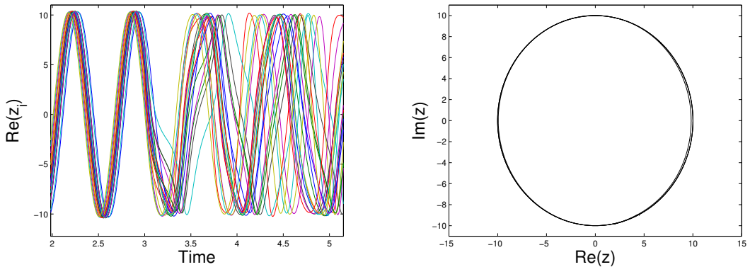
FIGURE 4.2: Large natural frequencies: desynchronization.
