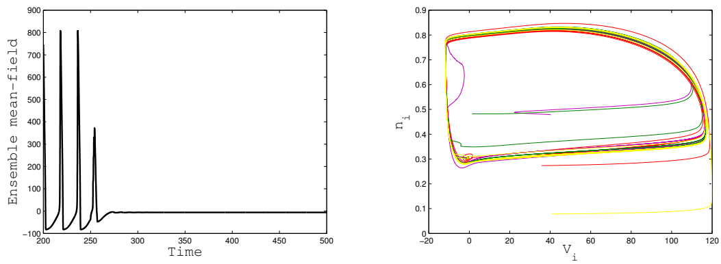
FIGURE A.6: Response of all-to-all coupled ( N = 7 ) Hodgkin-Huxley neuron model to proportional mean-field feedback. The feedback is switched on at t = 250 . Small natural frequencies: oscillation inhibition. Left: ensemble mean-field. Right: trajectory projection on the V_i, n_i planes.
