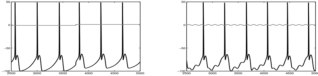
FIGURE 6.1: Robust pacemaking and afterdepolarization potentials in a detailed computational model of dopaminergic neurons. The gray trace depicts the injected stimulus.
