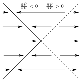
FIGURE 6.9: Sketch of the voltage dynamics of (6.5) for I = I_{tc} near the V -nullcline self-intersection in the singular limit \dot{n} = 0 . Thick lines are stable fixed points, dashed lines unstable. The dotted line is the locus \frac{\partial \dot{V}}{\partial V} = 0 . Arrows delineate the sign of \dot{V} in the different regions. The intersection point is a degenerate singular point of the voltage dynamics, corresponding to a transcritical bifurcation.
