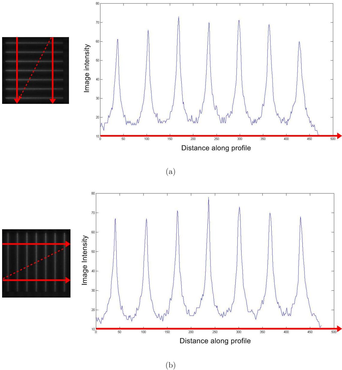
Figure 5.9: Profile analysis in an orthogonal direction to the axis of the pattern projection (a) horizontal pattern (b) vertical pattern
