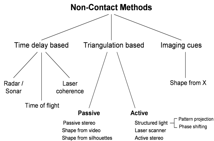
Figure 2.3: Hierarchy of non-contact 3D recovery approaches
