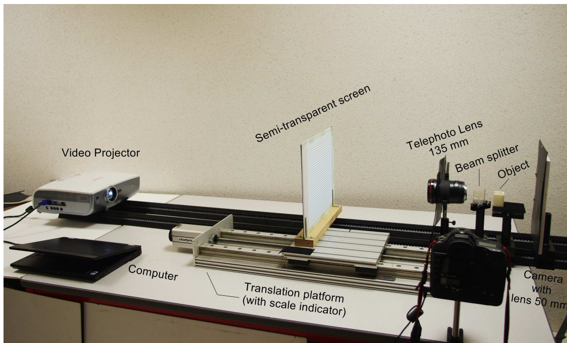
Figure 5.2: Experimental set-up
