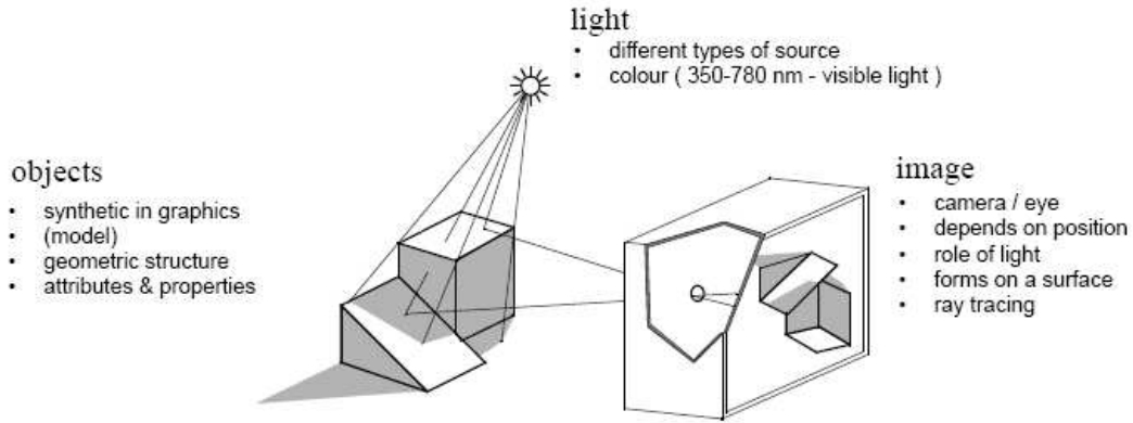
Figure 3.1: Pinhole Model
