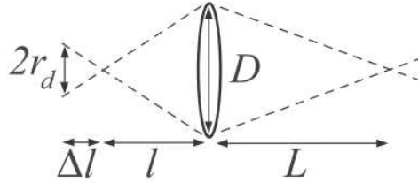
Figure 3.6: The defocus spot size
