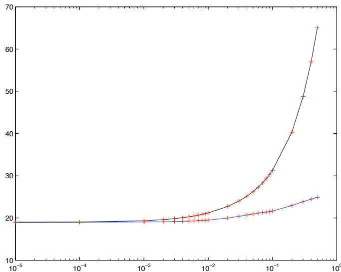
Figure 3.29: Value functions J(u_\varepsilon) in blue and J_\varepsilon(u_\varepsilon) in black, logarithmic barrier homotopy - second initialization, target L_2 , T_{\max} = 0.3N , computed points in red.
