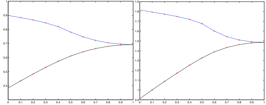
Figure 3.16: Value function for different \lambda , energy-consumption homotopy, target LO , T_{\max} = 10N left and T_{\max} = 5N right, J(u_\lambda) in blue and J_\lambda(u_\lambda) in black, computed points in red.
