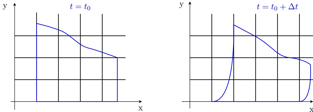
Figure 3.2: Eulerian mesh after a time increment. The two-dimensional mesh in black remains fixed, while the system represented with a blue line moves.
