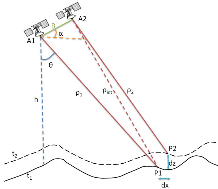
Figure A.4: InSAR geometry
