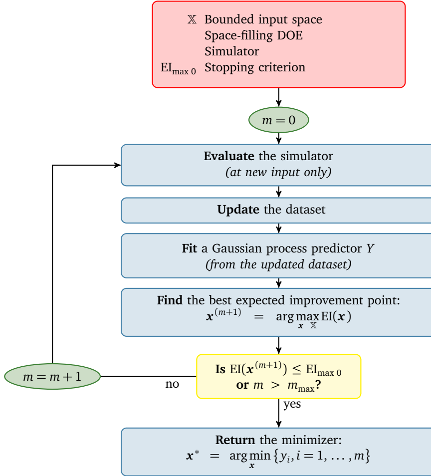
Algorithm 2.1 Efficient Global Optimizer
