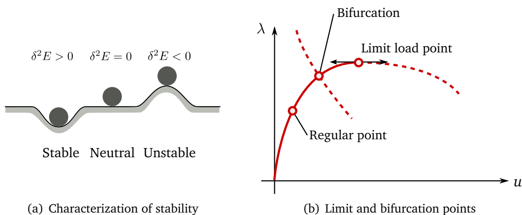
Figure 6.2: Equilibrium stability.
