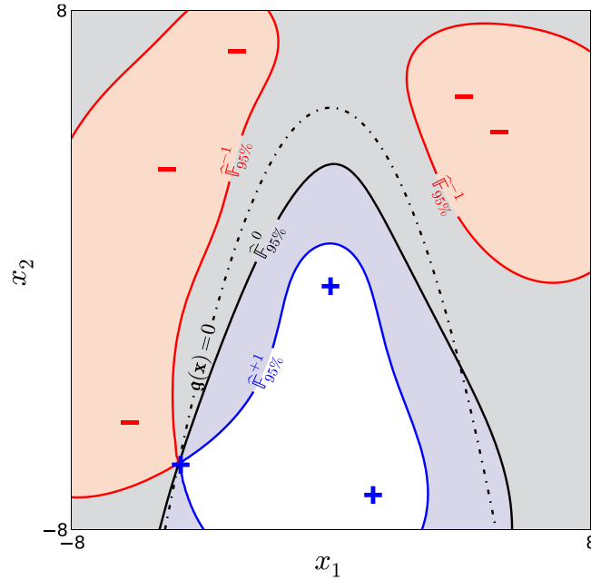
Figure 1.17: Approximate failure domains \mathbb{F}_{1-\alpha}^{-1} (red), \mathbb{F}_{1-\alpha}^0 (grey) and \mathbb{F}_{1-\alpha}^{+1} (blue) for the example from Section 1.5.3. The corresponding margin of uncertainty is defined as the relative complement of the red set in the blue set: \mathbb{M}_{95\%} = \mathbb{F}_{95\%}^{+1} \setminus \mathbb{F}_{95\%}^{-1} .
