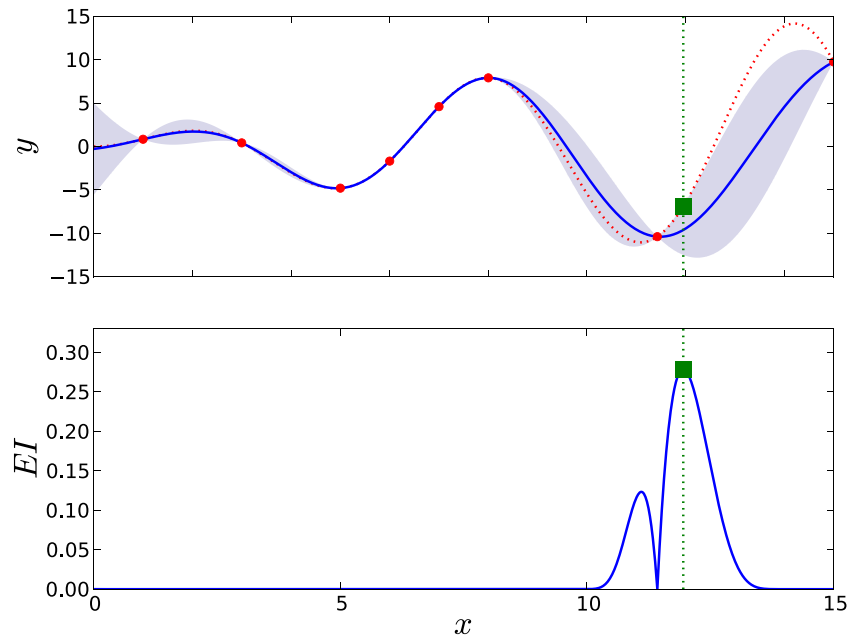
Figure 2.3: Implementation of the efficient global optimization technique for the minimization of f(x) = x \sin(x) on the interval \mathbb{X} = [0; 15] . The upper panel illustrates the original function (dotted line) together with its Gaussian process approximation (continuous line) built from the available dataset (red points). The lower panel illustrates the expected improvement and its maximizer which corresponds to the next evaluation required by EGO.
