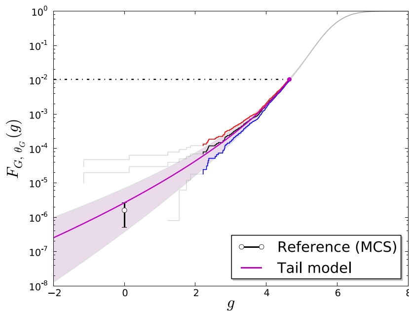
Figure 3.7: Inference of the tail of the distribution of the random performance G for the basic structural reliability problem defined in Section 3.2.4.
