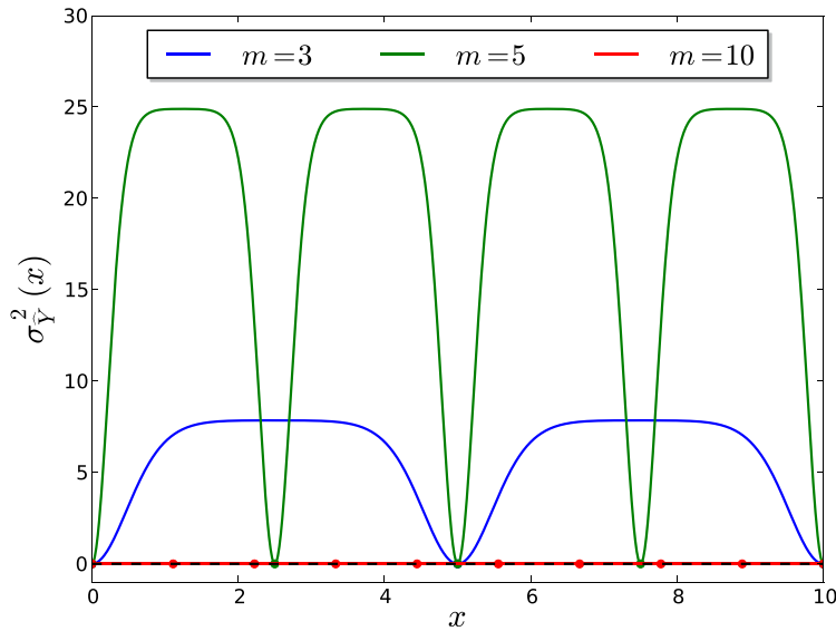
Figure 1.10: Asymptotic consistency of the best linear unbiased predictor for the one-dimensional function f(x) = x \sin(x) . The scale parameter \ell in the chosen squared exponential autocovariance model has been estimated by means of the maximum likelihood estimation technique (see Section 1.4.5.2) for each m .
