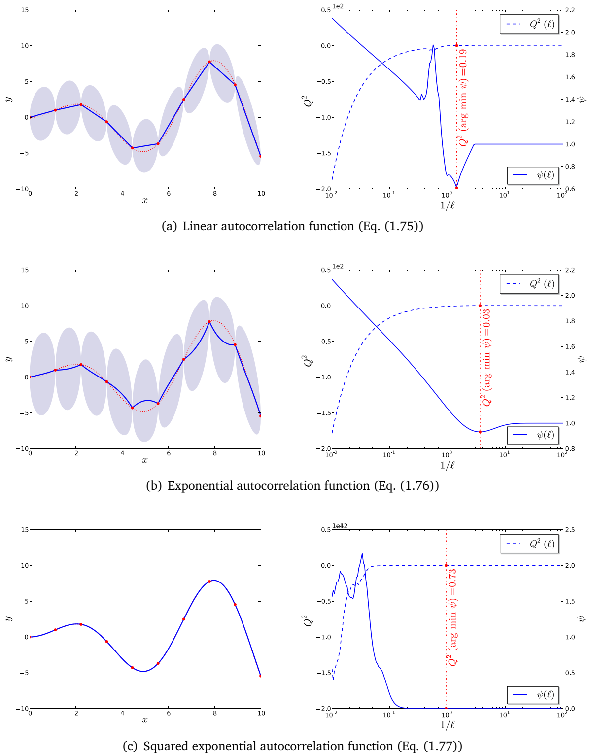
Figure 1.14: Universal Kriging models for (x) = x \sin(x) and various autocorrelation functions. The left-hand panels represent the observations and the probabilistic prediction as in Figure 1.11. The right-hand panels depict the reduced likelihood function \psi and the generalization score Q^2 as functions of the inverse scale parameter (1/\ell) .
