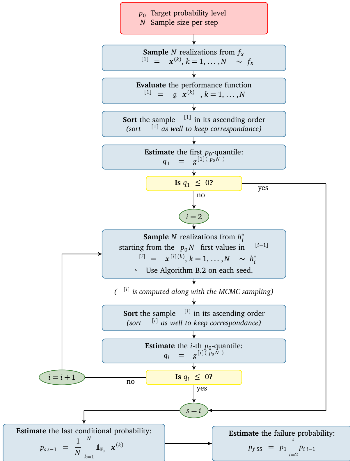
Algorithm 3.1 Adaptive splitting (or subset sampling)
