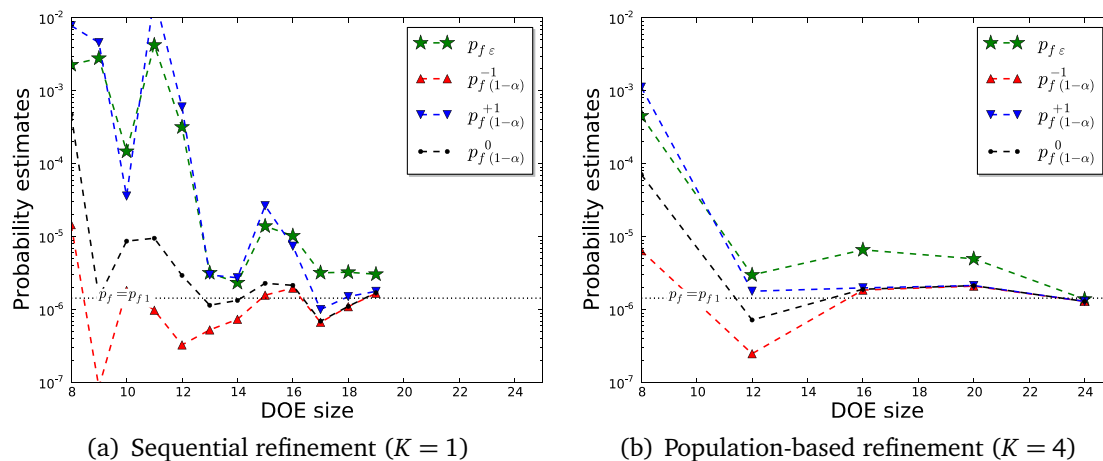
Figure 3.17: Convergence of various approximations of the failure probability for the basic structural reliability problem defined in Section 3.2.4.
