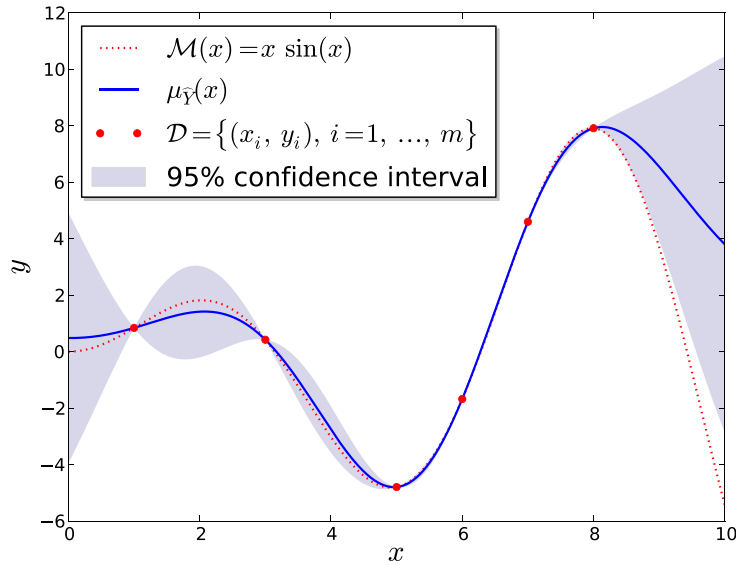
Figure 1.11: Gaussianity of the best linear unbiased predictor for the one-dimensional function (x) = x \sin(x) .
