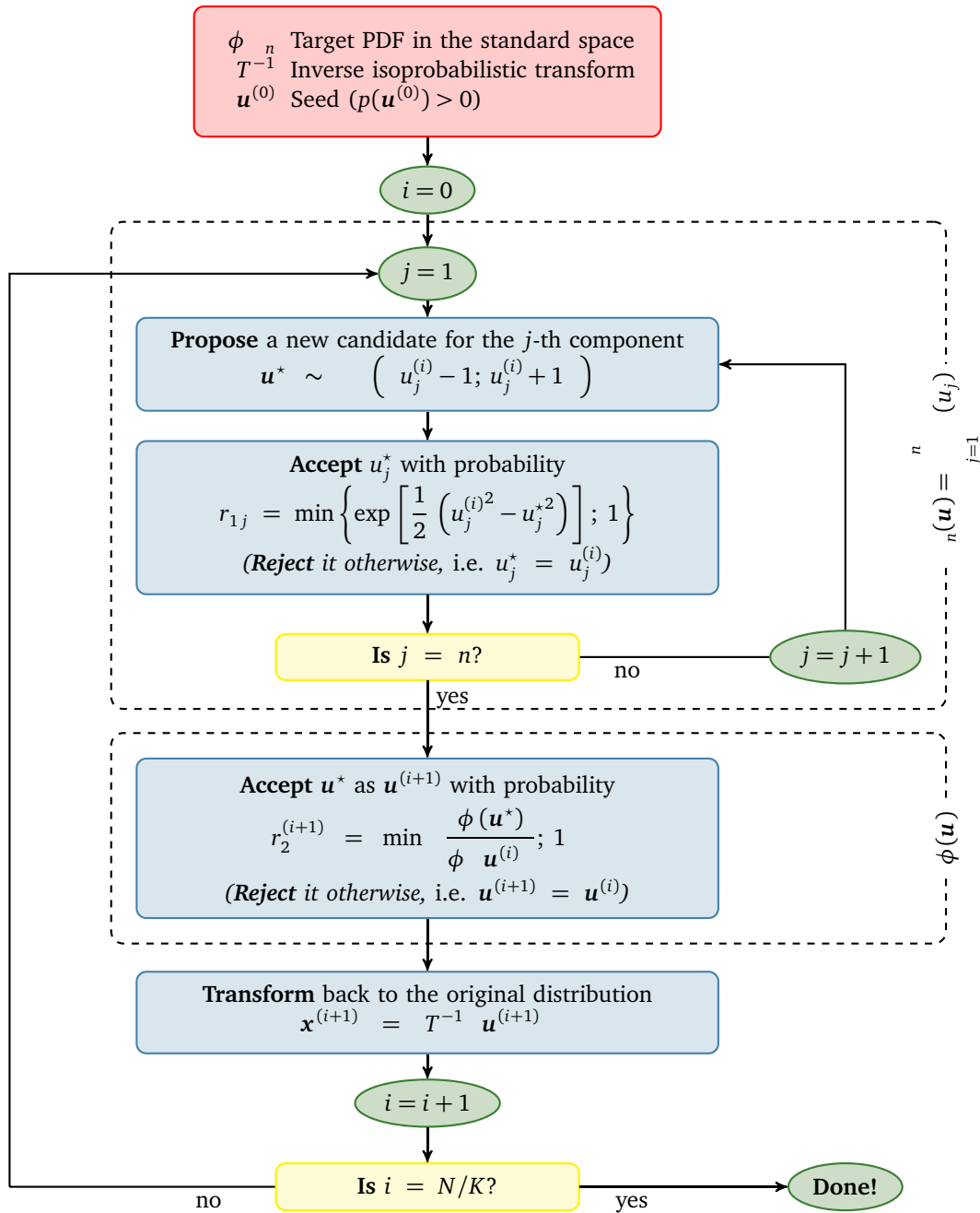
Algorithm B.2 Modified Metropolis-Hastings sampler
