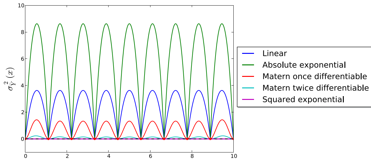
Figure 1.13: Prediction variance depending on the autocorrelation function for the approximation of the model \hat{y}(x) = x \sin(x) .
