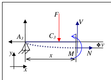
Figure 4-2 : Efforts internes
