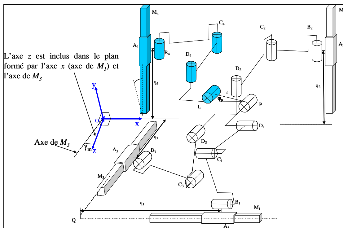
Figure 4-8: Isoglide4-T3R1 V2
