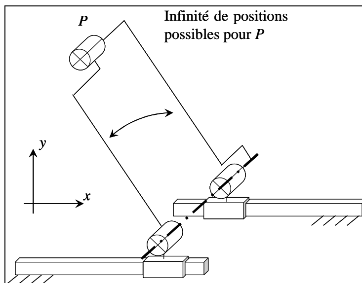
Figure 1-6 : Singularité architecturale
