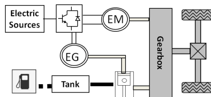
Figure 1.11: HEV series-parallel architecture
