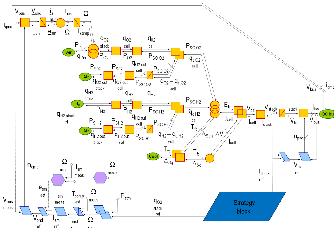
Figure 2.25: Fuel cell system practical control structure
