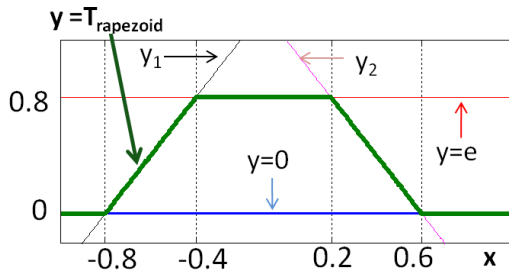
Figure 3.10: Trapezoidal MF example a = -0.8, b = -0.4, c = 0.2, d = 0.6, e = 0.8
