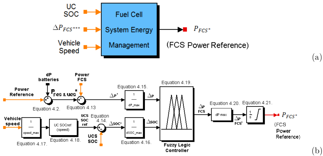
Figure 4.11: Fuel cell system local energy management strategy. (a) global view, (b) detail
