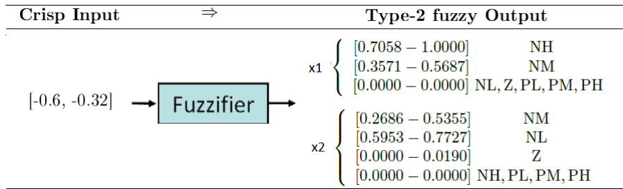
Figure 3.18: The fuzzifier: maps crisp inputs into type-2 fuzzy sets outputs
