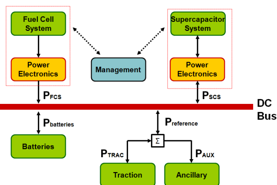
Figure 1. Energy configuration of the Vehicle
