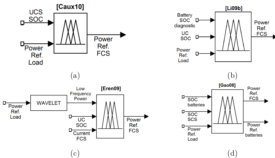
Figure 1.17: Fuzzy logic controllers used in hybrid electrical vehicles energy management (a) [Caux10], (b) [Li09b], (c) [Eren09], (d) [Gao08]
