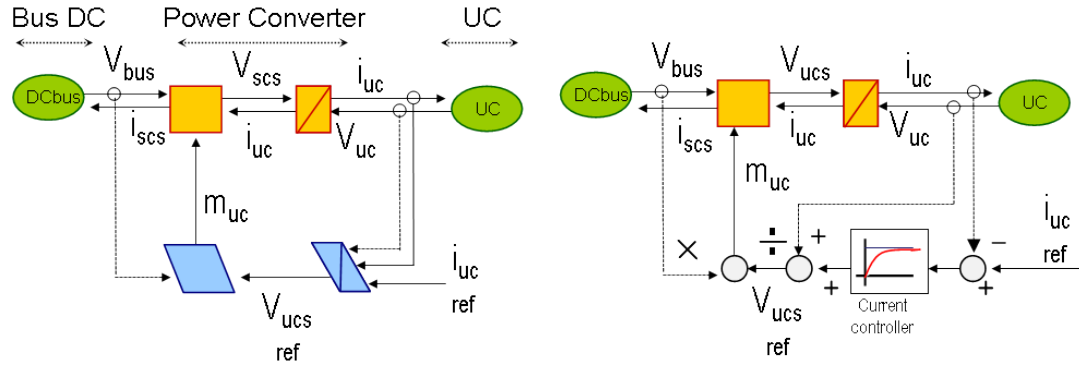
Figure 2.14: UCS EMR and control structure: MCS and PCS (left) detail (right)
