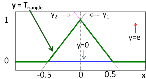
Figure 3.11: Triangular MF example a = -0.5, b = c = 0, d = 0.5, e = 1
