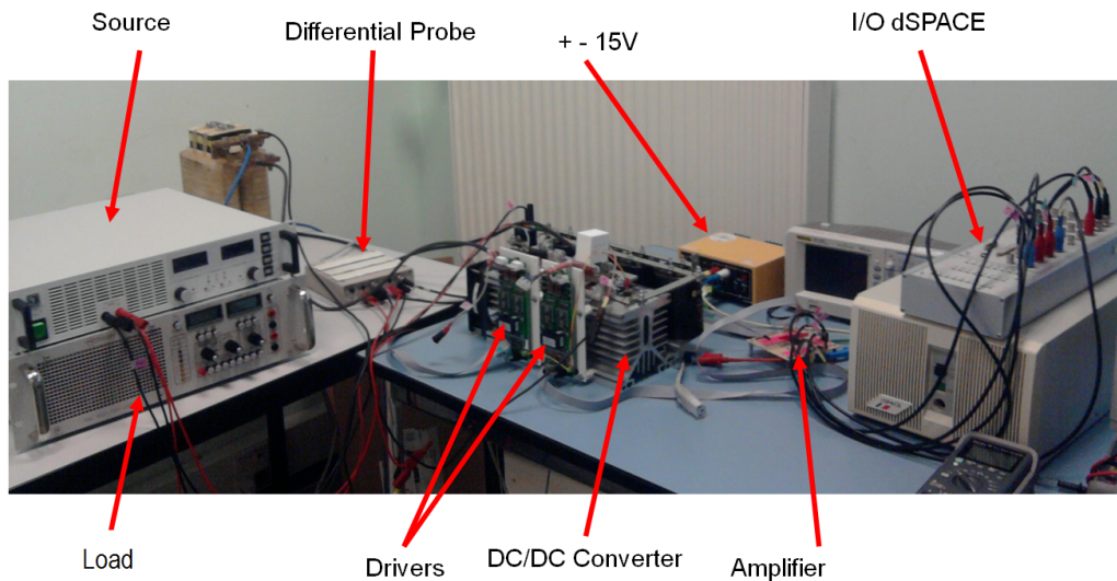
Figure 3.35: Experimental setup
