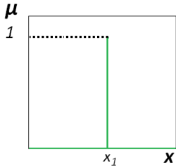
Figure 3.4: Singleton MF
