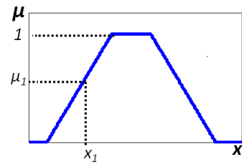
Figure 3.6: Type-1 MF
