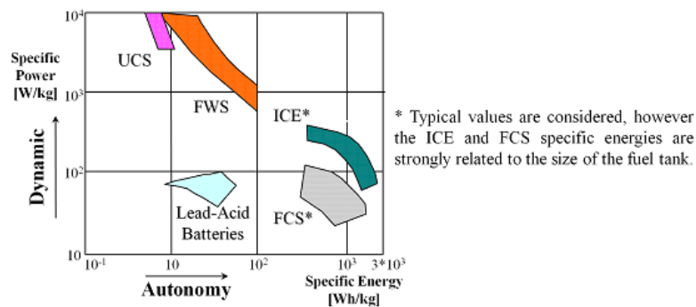
Figure 1.12: Ragone plot [Rago68] including ECCE hybrid electric vehicle energy sources
