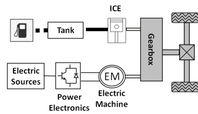
Figure 1.10: HEV parallel architecture
