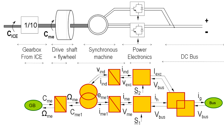
Figure 2.29: Flywheel system - Electrical part EMR
