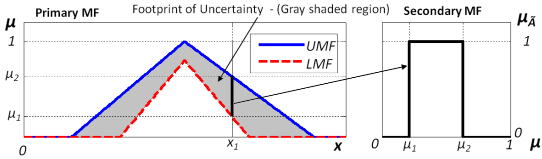
Figure 3.9: Interval type-2 fuzzy logic primary and secondary MFs
