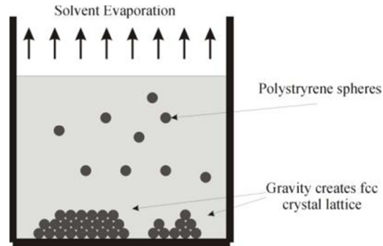
Figure III-3 Sedimentation method
