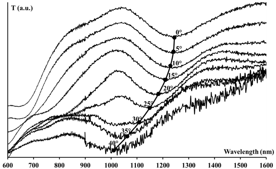
Figure IV-16: Transmittance spectrum with different incident beam angles ( 0^\circ - 40^\circ ). The inverse opal is made by 800 nm diameter size of PS template
