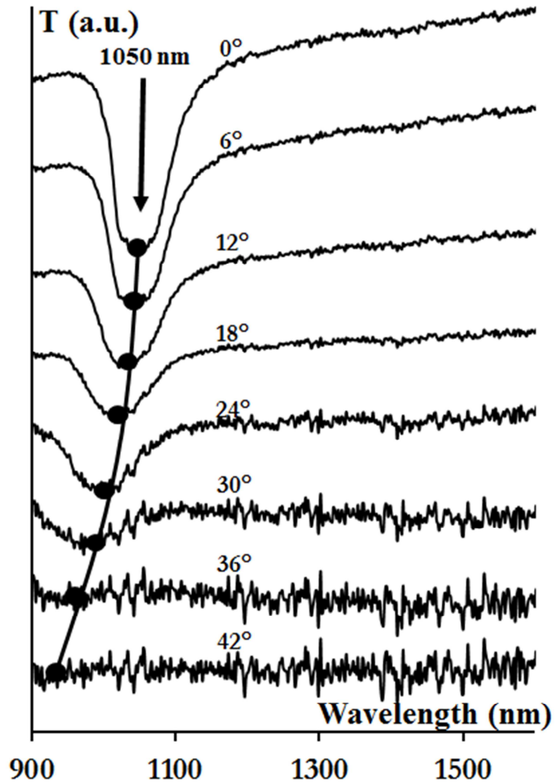
Figure IV-8: Transmittance of the direct opal as a function of the incident angle. The diameter of the polystyrene sphere is 453 nm and a focus is made on the first harmonic
