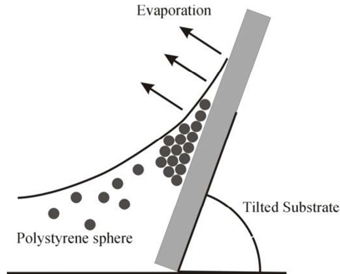
Figure III-4: Vertical deposition
