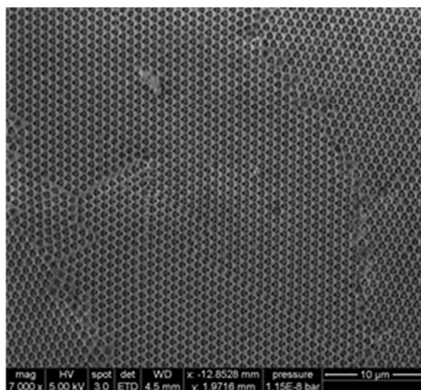
Figure IV-18: SEM image of non-magnetic inverse opal made by 903 nm direct opal with x7000 magnification
