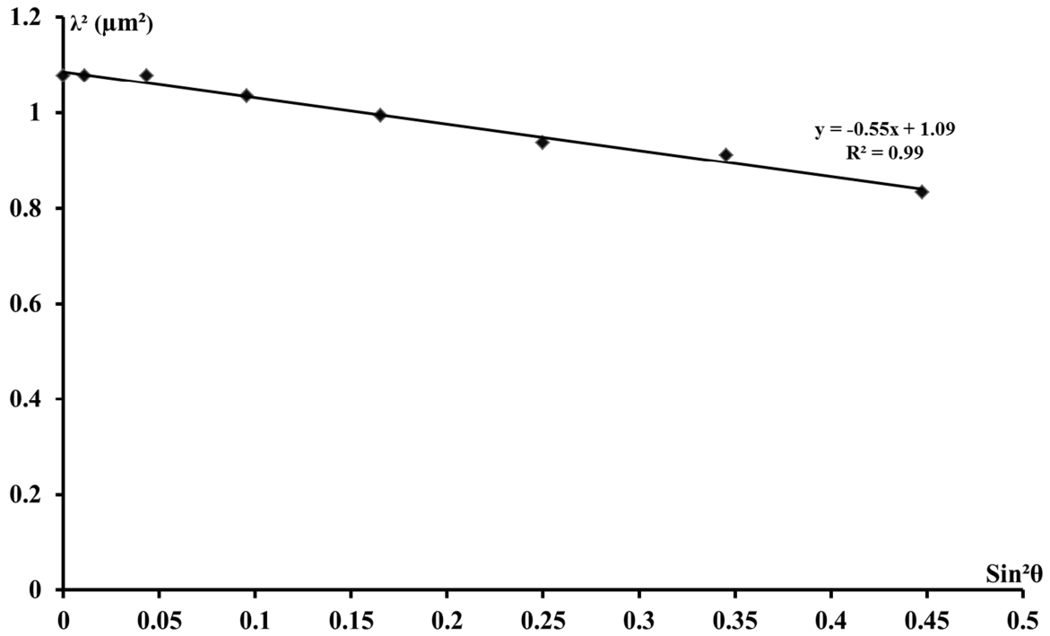
Figure IV-9: Center position of the first harmonic PBG on square plotted as a function of the \text{sin}^2\theta angle rotation
