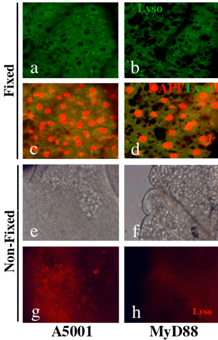
Figure 5.1: Autophagy and lipid droplets in starved wild type and MyD88 mutant flies.
