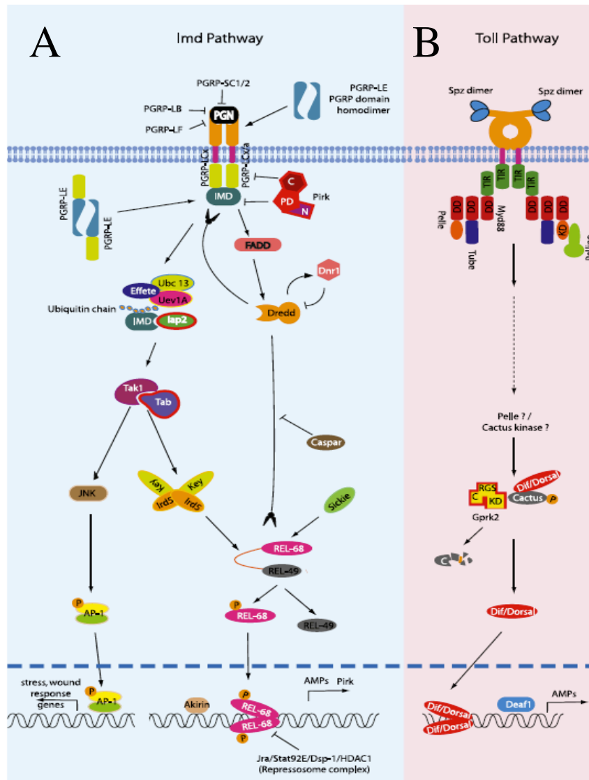
Figure 1.3: The IMD and Toll pathways
