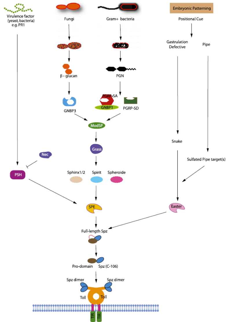
Figure 1.5: Cleavage of the SPZ cytokine which is required for Toll pathway activation
