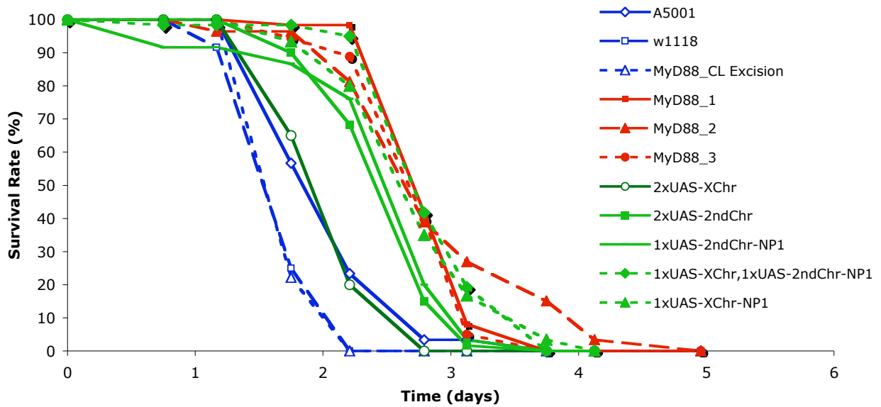
Fig. S8 : The insertion of the MyD88 + transgene on the X predicts a recessive suppressor of the MyD88 starvation phenotype
