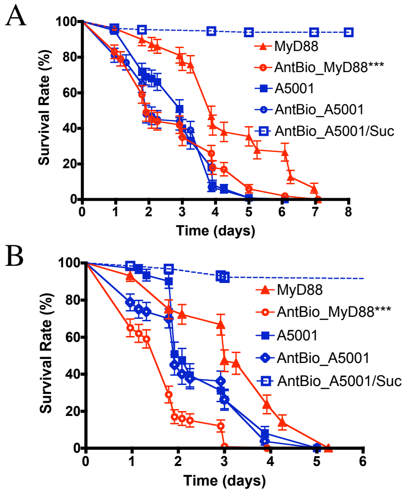
Figure 5.6: Starvation experiment using axenic flies.
