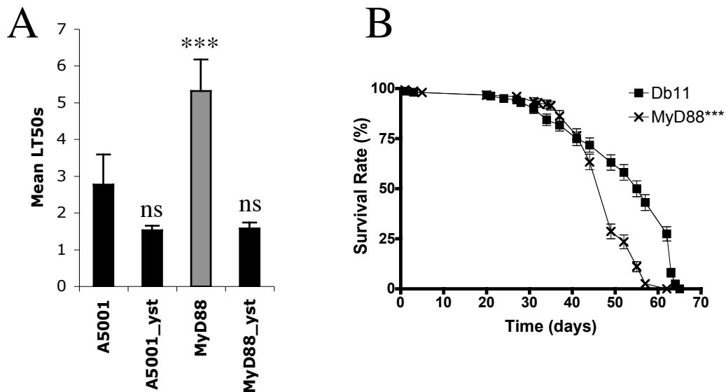
Figure 5.10: Additional source of yeast affects survival of MyD88 mutants
