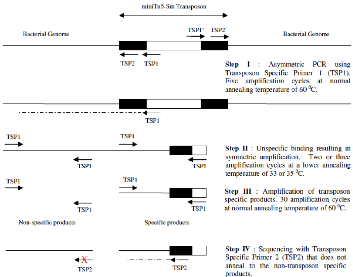
Figure 3.1: Identification of transposon insertion site in the genome of S. marcescens by single primer PCR. Two transposon-specific primers on left side: (TSP1: 5'ctaggcggccagatctgatcaa3', and TSP2: 5'gctgttcttctacggcaagg3') and two on right side (TSP1': 5'caccaaggtagtcggcaaat3', and TSP2': 5'cgaactgtgtataagagtcag3') of the mini-Tn5-Sm transposon were designed, respectively. The DNA fragments were amplified in a three step PCR reaction: i) Step I: TSP1 and TSP1' were used separately to amplify single strand transposon-specific DNA fragments that also contained part of S. marcescens genome-specific DNA sequence, ii) Step II: The melting temperature ( T_m ) was decreased to generate double-stranded sequences as a result of non-specific binding of the primers, and iii) Step III: double stranded DNA fragments were then amplified at normal T_m . Finally, in Step IV, the amplified fragments were purified from PCR reaction mixtures and sequenced using remaining two transposon-specific primers (TSP2 for TSP1-, while TSP2' for TSP1'-amplified fragments) that yielded part of transposon-specific and part of S. marcescens genome-specific DNA sequences. These sequences were blasted with genome of S. marcescens using BioEdit software. After the identification of the site of insertion of the transposon, primers were designed in the genome of S. marcescens in the vicinity of the transposon insertion site to perform a normal PCR reaction for reconfirmation of the results obtained from the single primer PCR.
