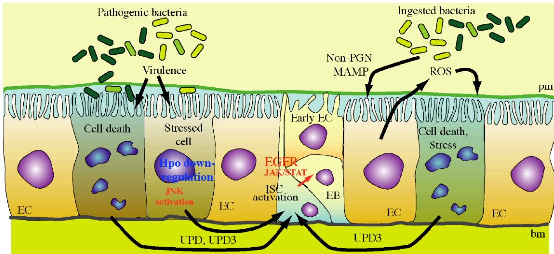
Figure 1.8: The Drosophila midgut homeostasis. The enterocytes (ECs) in the midgut epithelium are damaged either by the virulence factors of pathogenic bacteria or overactivated host immune response triggered against ingested microbes. The damages to ECs, as well as activation of JNK pathway and downregulation of Hippo (Hpo) pathway in the stressed ECs, lead to the secretion of cytokines, such as unpaired (UPD), and UPD3. After receiving a stress signal, the JAK/STAT and EGFR pathways are induced in ISCs (located in the vicinity of the basal membrane (bm)), thus leading to the compensatory proliferation of ISCs that maintains homeostasis. Modified from (Limmer et al., 2011).
