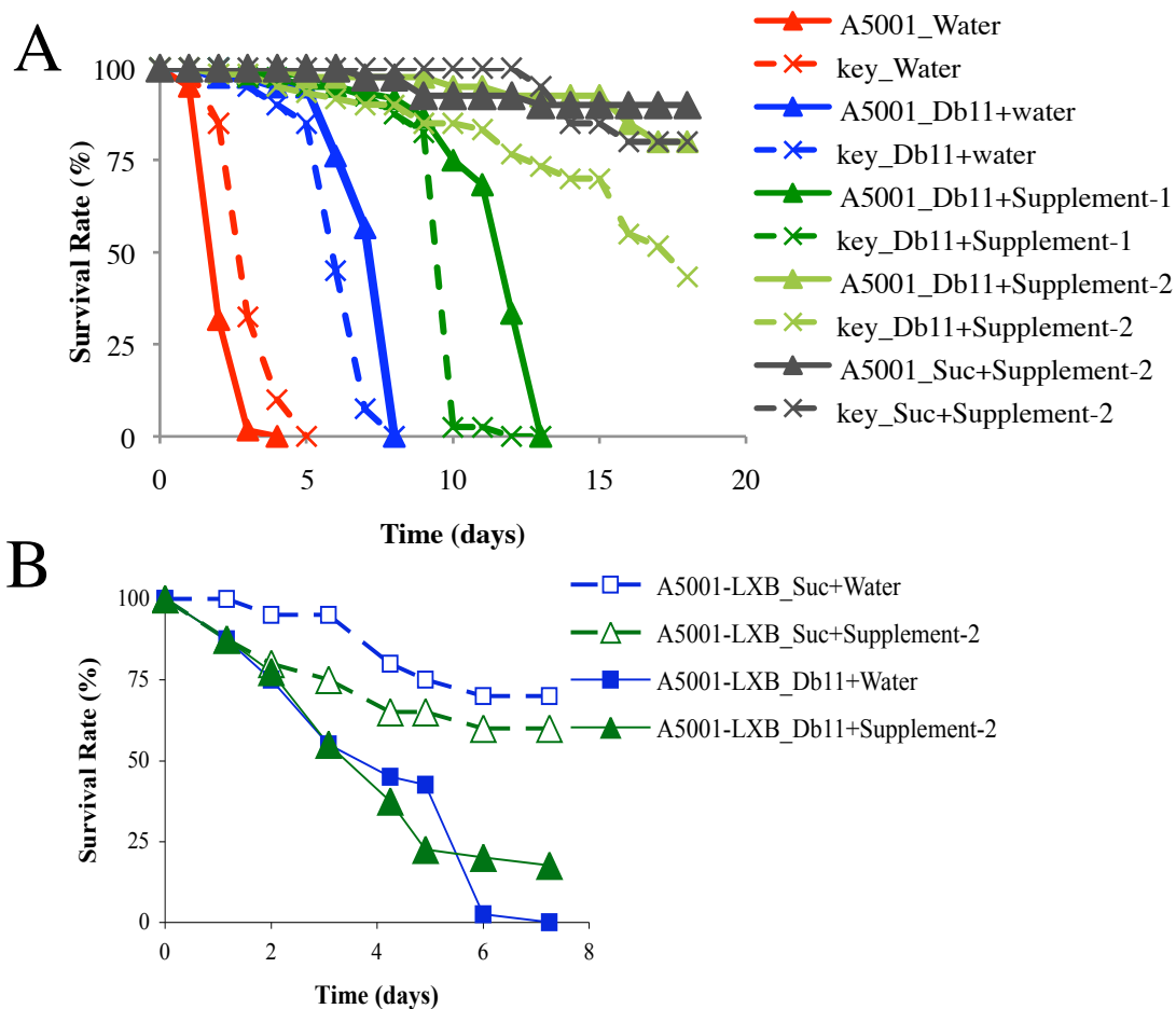
Figure 2.3: S. marcescens kills immunocompromised flies
