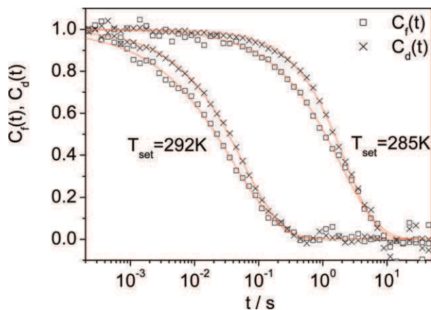
Fig. 2 Auto correlation functions C_f(t) , C_d(t) of fluorescence lifetime and linear dichroism fluctuations, respectively. Note that the binning free analysis 25 allows for correlation data even at very short times.
