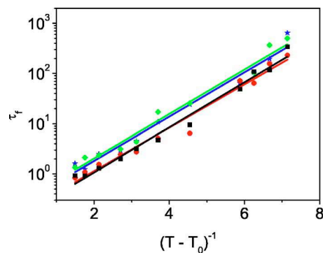
FIG. 10. (Color online) Vogel-Fulcher plots of the relaxation times \tau_l for a small ( M=1, \sigma=1 , squares; M=2.25, \sigma=1 , circles) or large ( M=1, \sigma=1.22 , diamonds; M=2.25, \sigma=1.22 , stars) dumbbell in the considered system. The values of the Vogel temperature T_0 and of the “fragility parameter” B/T_0 are presented in Table III.
