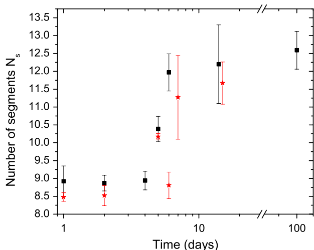
Fig. 2. Temporal evolution of the number of polymer segments N_s rearranging around DiD molecules embedded in a 70 nm thick polystyrene matrix. The values given correspond to the peaks of the distributions (Fig. 3), obtained on a daily basis after the spin coating (squares) or casting (stars) procedure has been initiated at room temperature 22 °C. The value pointed after break on the x scale corresponds to the peak value of the distribution of the number of segments obtained after annealing of the spin coated film.
