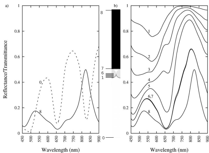
FIG. 3. (a) Simulated reflection (0, dashed) and transmission (8, solid) spectra of an array of hcp arranged monodisperse silica particles of diameter D=300 nm enclosed in between a front gold curved mirror and a gold-coated silicon wafer. (b) Simulated transmission spectra through flux planes situated at distances 5 (1), 30 (2), 50 (3), 70 (4), 90 nm (5) from the curved front mirror, in the center (6), at the back of the cavity (7) and at the outlet of the structure (8). Inset: geometry of the simulated structure with indication of the positions of the planes used for flux detection. The source originates from plane 0 and goes upwards. It is partially reflected/transmitted by the cavity. The reflected flux is detected back through plane 0. The transmitted flux goes through the cavity, entering at the front mirror, is detected successively through planes 1 (5 nm after the front mirror) to 7 (back mirror) prior to continue through the substrate to be finally detected through plane 8 (outlet of the structure).
