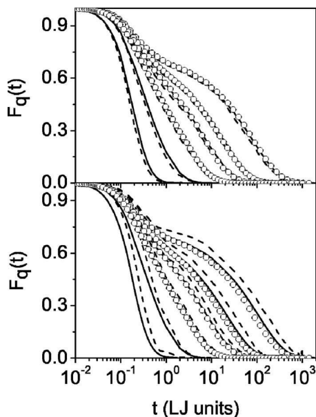
FIG. 1. Self-incoherent scattering functions of the dumbbell (dash), the polymer chains surrounding it (solid), and of the model system simulated in the absence of the probe (open circles). The probe is either a dimer of the surrounding mers ( M=1 , \sigma=1 , top) or a larger probe ( M=2.25 , \sigma=1.22 , bottom). T=0.5, 0.55, 0.55, 0.6, 0.7, 1.0 , and 2.0 from right to left, respectively.
