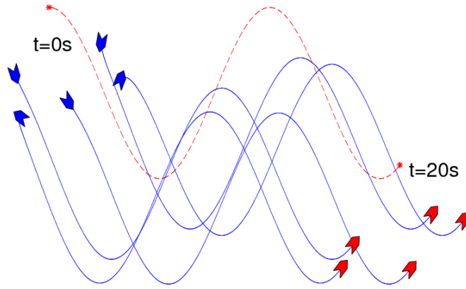
Figure 3.14: Simulation of five agents governed by (3.32). The blue lines represent the trajectories of the agents following a reference velocity given by the red dashed line \dot{\mathbf{r}}_{ref} = (1, -2 \sin \frac{t}{2}) . The figure shows two snapshots. The blue agents represent the initial conditions. The red ones represent the final state at t = 20s .
