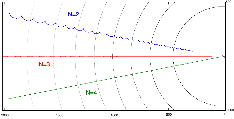
Figure 4.5: Trajectories of the formation center \mathbf{c} for different numbers of agents N when \sigma has circular level sets. Location of source is denoted by the \times . Image courtesy of Brandon J. Moore.
