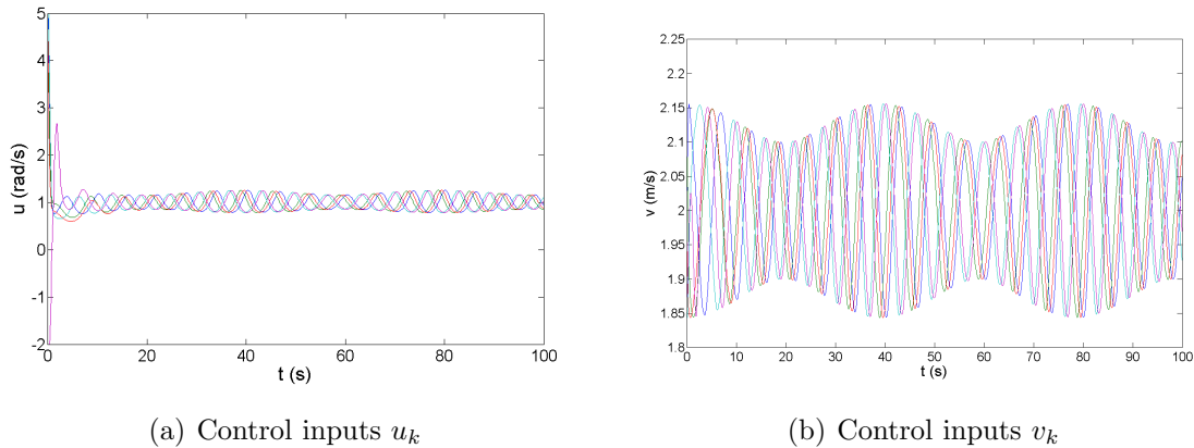
Figure 2.8: Evolution of the control inputs u_k (a) and v_k (b) corresponding to the previous simulation of five agents shown in Figure 2.7.
