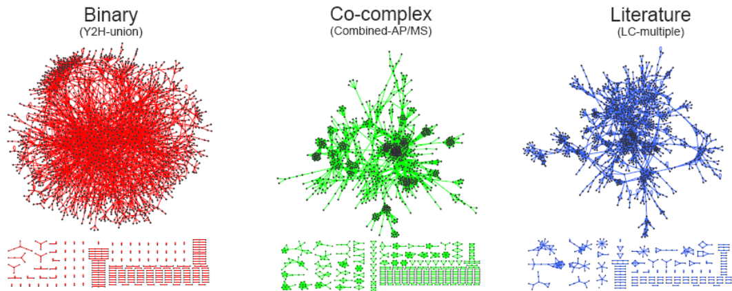
Figure 2.5: Graphical representation of three different types of yeast interactome datasets. (taken from High-Quality Binary Protein Interaction Map of the Yeast Interactome Network , Yu et al. , Science 2008.)
