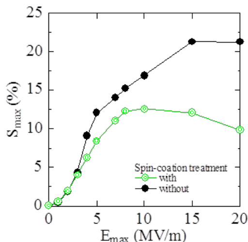
Figure 4.27 Experimental changes in maximum strain versus maximum electric field of 0.89 vol% composite with and without and spin-coating treatment films.
