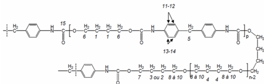
Figure 2.3 Structure of PU - Estane 58888.
