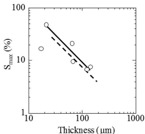
Figure 4.36 Linear logarithmic relationship between thickness of pure PU (broken line) and composite (open circle and line) films and maximum strain (20 MV/m), which is maximum strain at maximum electric field of 20 MV/m.
