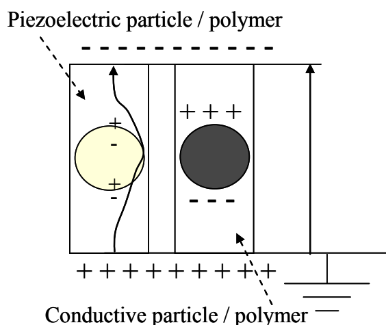
Figure 2.5 A schematic of electric induction for composite films filled with ferroelectric and conductive particles.
