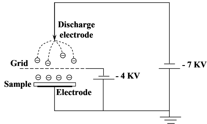
Figure 5.1 Corona discharge setup.
