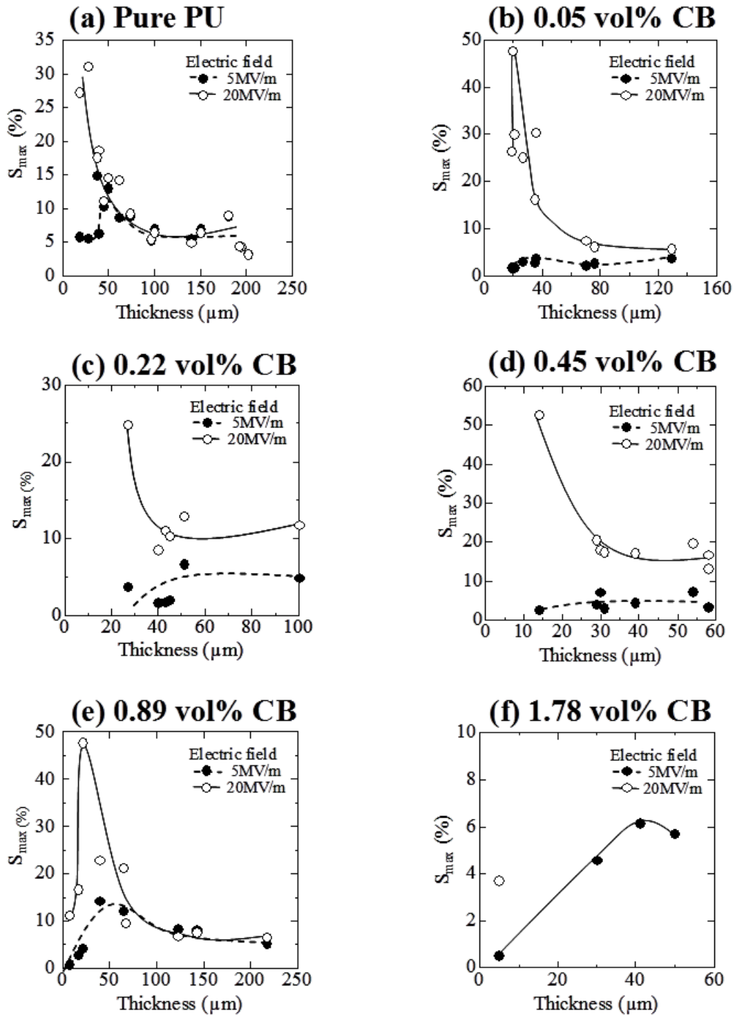
Figure 4.33 Thickness dependent maximum strain of pure PU and composites films as a function of the thickness at 5 and 20 MV/m.
