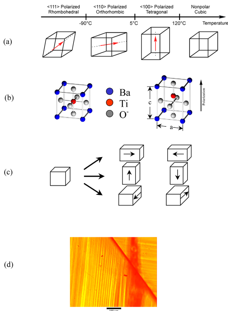
Figure 1.3 (a) Various crystalline phases of BaTiO 3 ; (b) crystal structures of BaTiO 3 in their cubic and tetragonal phase; (c) the six tetragonal variants; (d) domain pattern in single crystal BaTiO 3 visualized using polarized light microscopy. [9]
