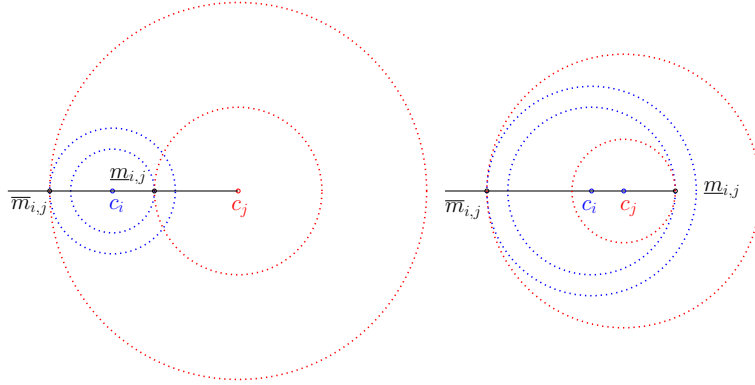
Figure 3.4: Relative position of minimal and maximal TT balls of two balls (Left) \overline{B}_j[\rho_{i,j}] and \overline{B}_i[\rho_{i,j}] are exterior tangent (Right) \overline{B}_j[\rho_{i,j}] is interior tangent to \overline{B}_i[\rho_{i,j}] .
