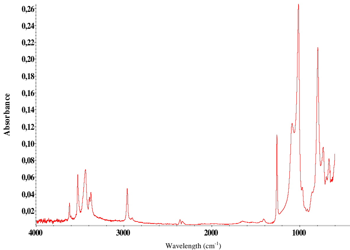
Figure 2.1 : ATR-IR spectra of filled silicone
