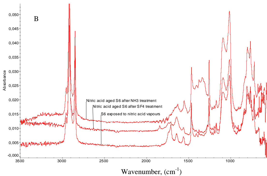
Figure 4: FTIR spectra A - SF 4 treatment on sample S6 (thermo-aged); B- SF 4 and NH 3 treatments on sample S6 (after nitric acid ageing).
