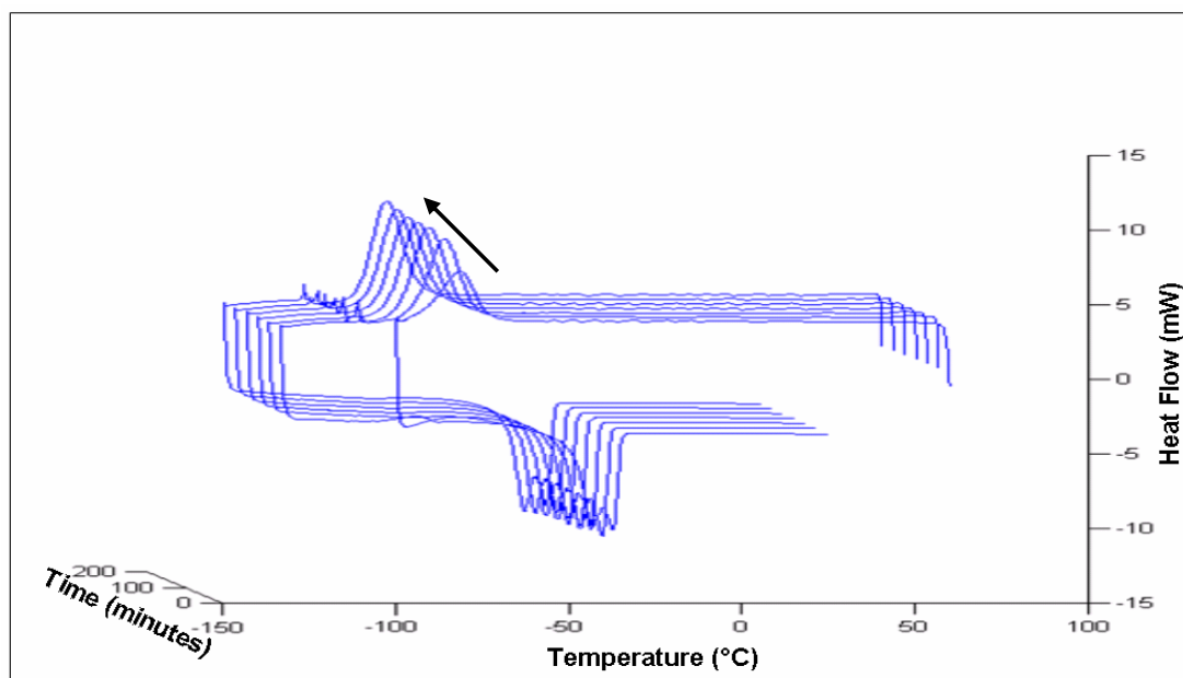
Figure 7 A: Photo-DSC thermograms after irradiation at 31 mW/cm 2 at 60°C ( \lambda > 300 nm) (initial, 30, 60, 90, 120, 150 and 180 min); for S2
