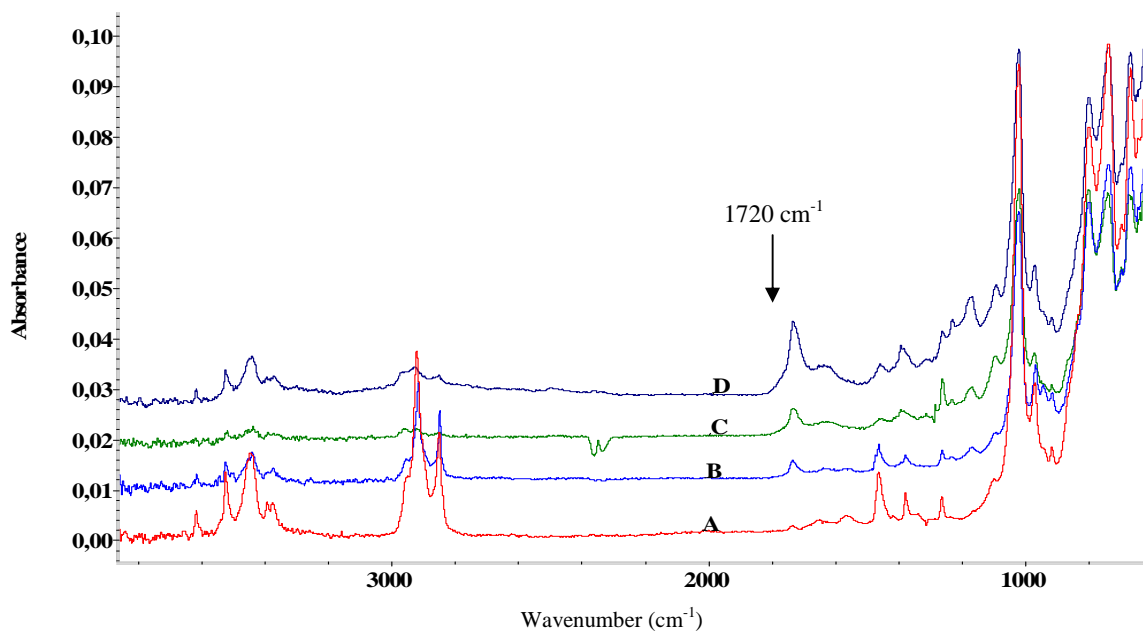
Figure 5: FTIR spectra of EPDM after photo-aging at 60°C (A=Initial, B = 24 hrs, C= 108 hrs, D= 600 hrs)
