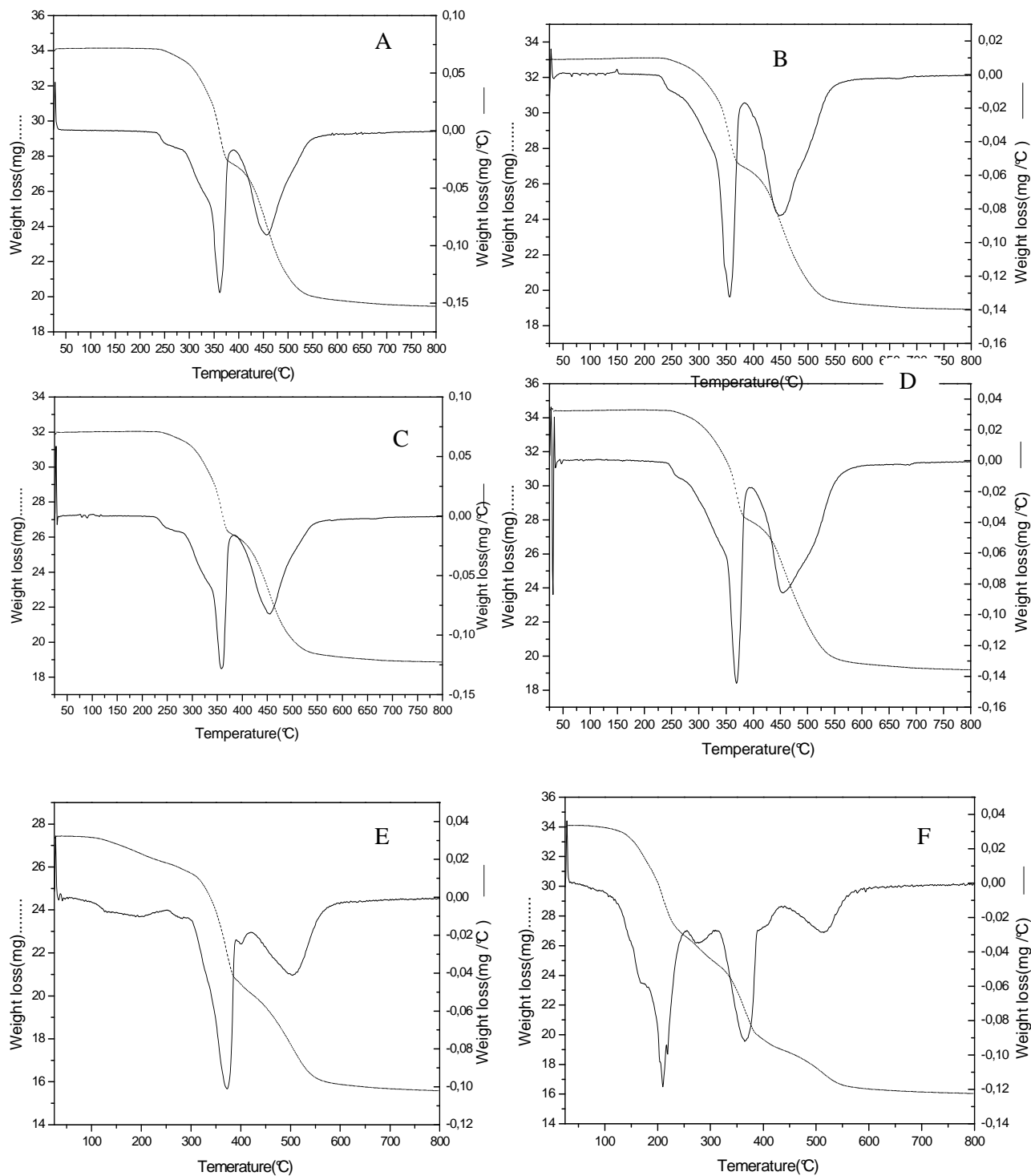
Fig. 7. TGA of silicone rubber before and after ageings (weight loss and derivate curves); A– Unaged sample; B– 10 000 hours in photochemical device; C– 10 000 hours in oven; D–260 hours under sulfuric acid treatment; E– 48 hours under nitric acid treatment; F– 2 months under nitric acid treatment.
