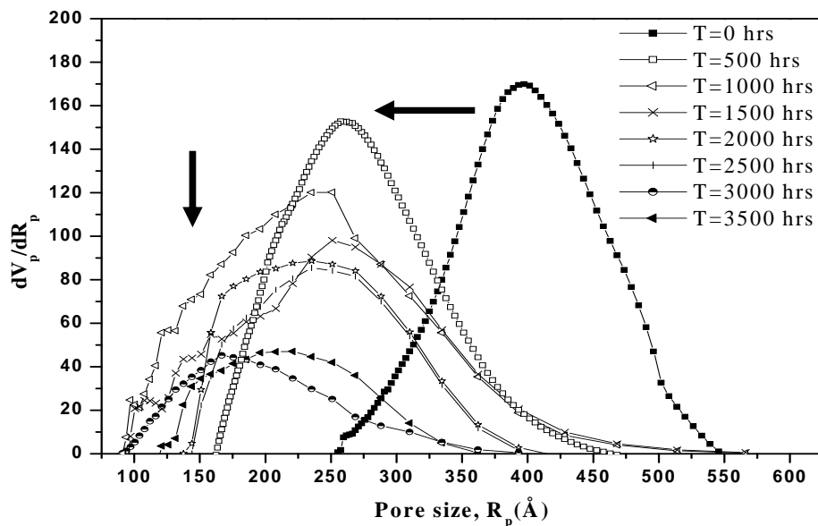
Figure 4: DSC-Thermoporosimetry results after thermal aging
