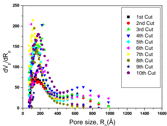
Fig. 5. Cross-linking profile obtained by DSC-thermoporosimetry on unaged sample surface (radius or pore size R_p , distribution dV/dR ).
