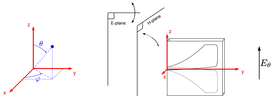
FIGURE 1.19: Axes and angles convention used for defining the radiation pattern of ETS antennas.
