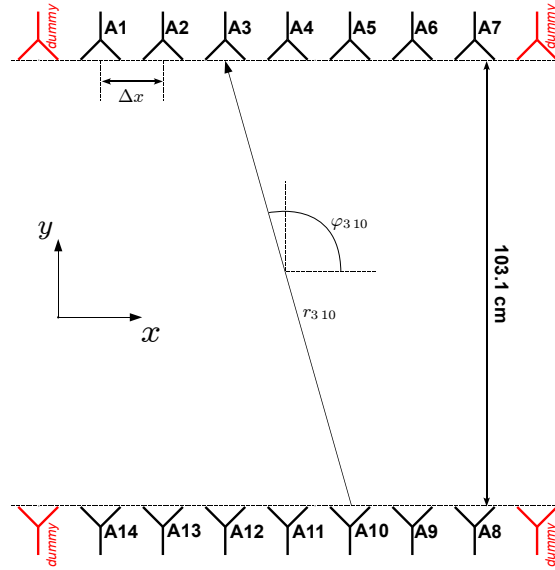
FIGURE 1.22: Measurement setup for the characterization of the antennas.
