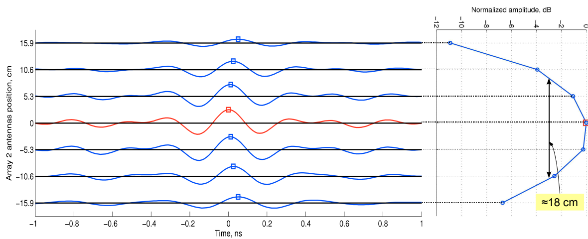
(b) W/ antenna coupling (FIG. 2.3)
