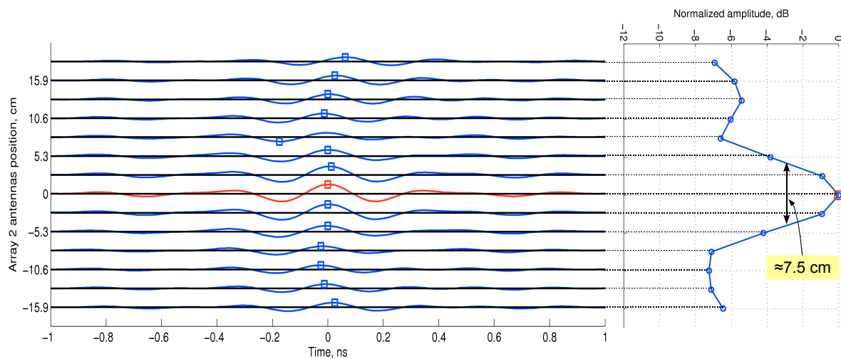
(c) W/ antenna coupling and “disorder” (FIG. 2.4)
