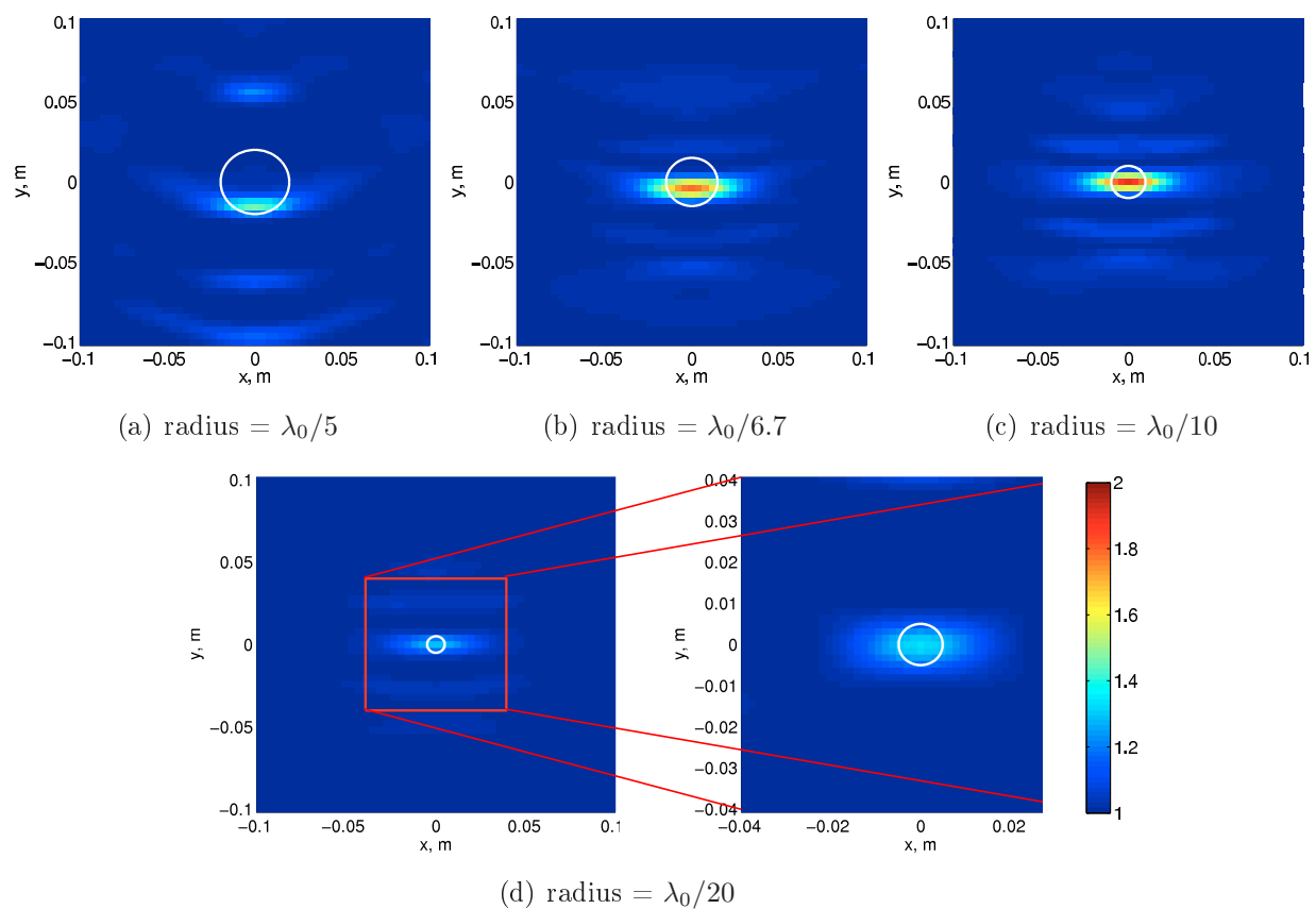
FIGURE 3.22: Synthetic data inversion of a dielectric cylinder with \varepsilon_r = 2 and four different radii. Only the \varepsilon_r profile is shown. The configuration is equivalent to the one in FIG. 3.13. In (d), two inversions have been run with two different \Omega sizes (hence different pixel sizes) to prove that the low \varepsilon_r values found with a large \Omega (left) are not due to the large pixel size-target dimensions ratio.
