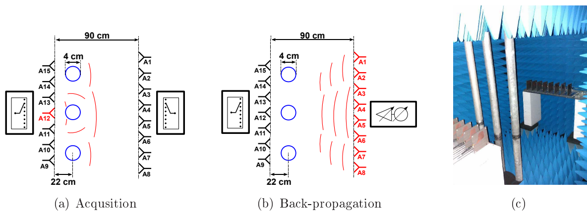
FIGURE 2.4: Time Reversal experiment setup. With respect to FIG. 2.3 three metallic cylinders are placed in front of the array-2.
