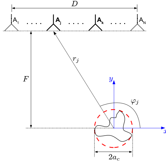
FIGURE 2.14: Configuration for deriving the properties of the DORT method.
