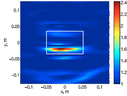
FIGURE 3.27: Same as FIG. 3.26, but the target is forced to be purely dielectric. Final result (\varepsilon_r; \infty) .
