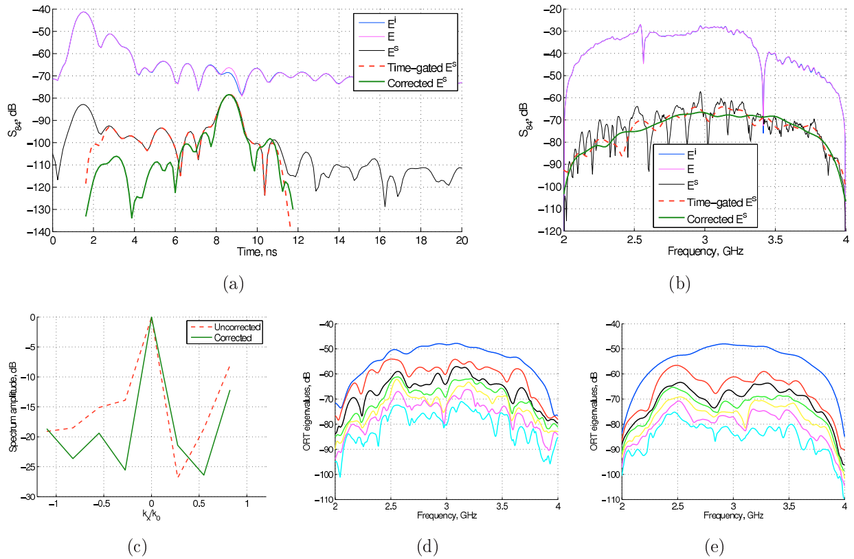
FIGURE 1.18: Impact of the drift correction algorithm for the setup in FIG. 1.17. (a) and (b) are the time- and frequency-domain S_{84} signals before and after the correction. In (c) the spatial spectrum bandwidth reduction at 3 GHz can be appreciated. In all these cases, A_4 is the transmitting antenna. (d) and (e) finally show the DORT eigenvalues distribution as a function of frequency without and with the drift correction, respectively.
