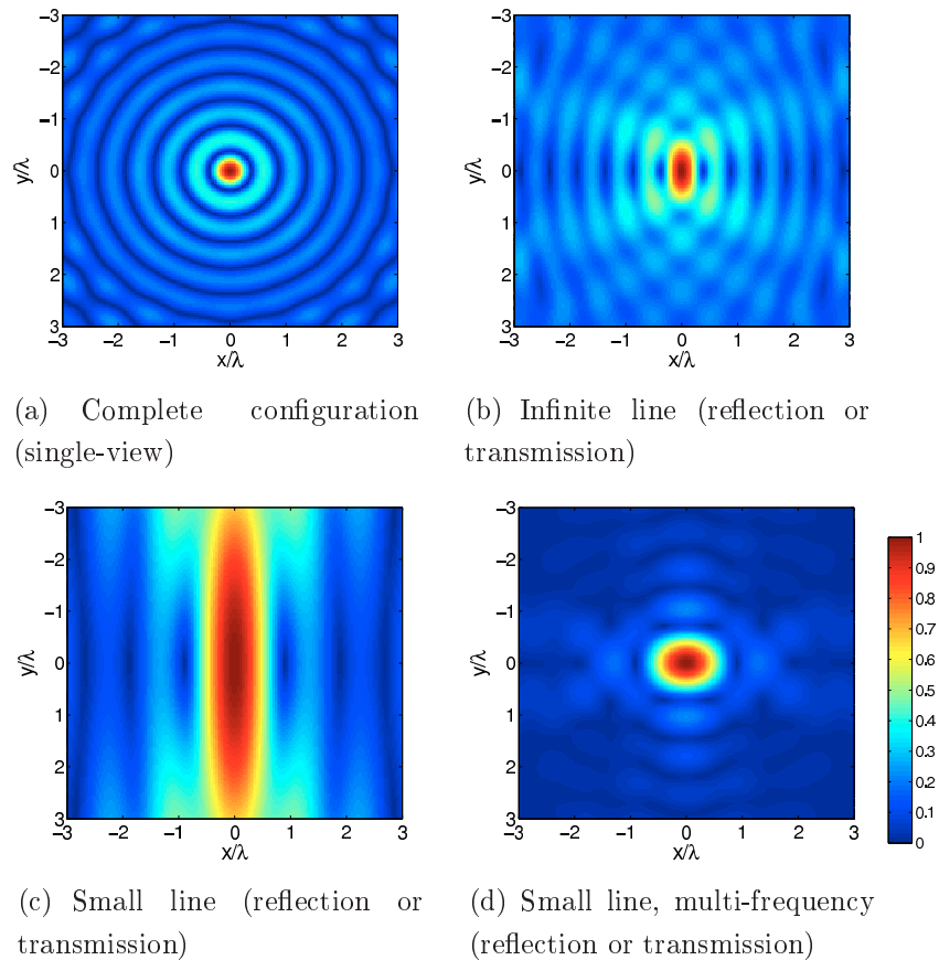
FIGURE 3.3: Resolution patterns issued from the Ewald's circle formalism. All the configurations are single view, and the amplitude scale is linear. x and y axes are normalized with respect to the wavelength (in (d) it is the one corresponding to the central frequency, \lambda_c ).
