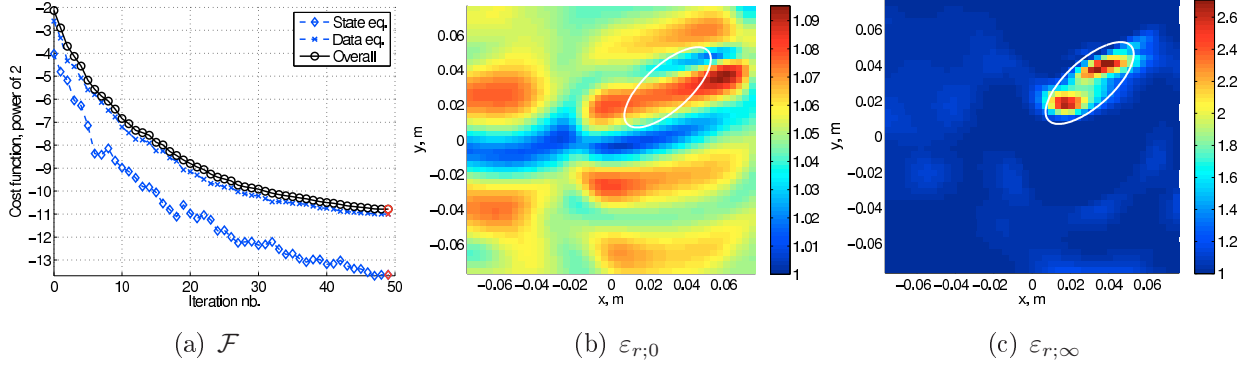
FIGURE 4.5: Noiseless data. Inversion results with \mathcal{F}^{\text{DORT}} and TX beamforming.
