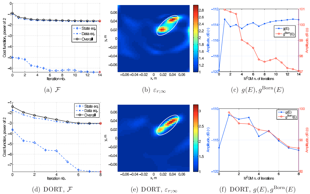
FIGURE 4.8: noise1 dataset. Inversion results with (top) the standard cost function \mathcal{F} and (bottom) \mathcal{F}^{\text{DORT}} .
