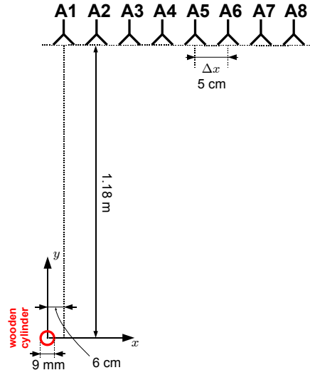
FIGURE 1.17: Reflection measurement setup used to test the drift correction algorithm.
