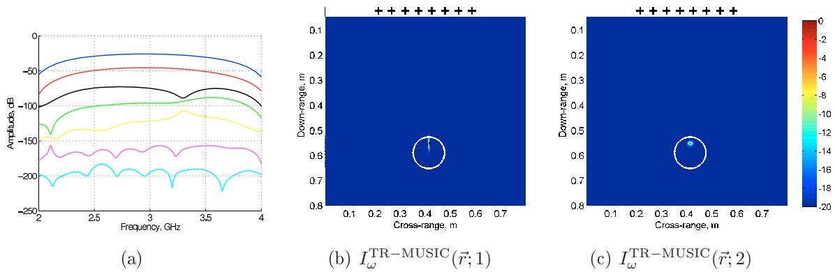
FIGURE 2.24: Synthetic data relative to the configuration in FIG. 2.18. (a) Singular values distribution, and (b-c) TR-MUSIC images at 3 GHz with signal subspace dimension M = 1 and M = 2 , respectively.
