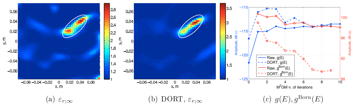
FIGURE 4.10: noise2 dataset. Inversion results with \mathcal{F} and \mathcal{F}^{\text{DORT}} .
