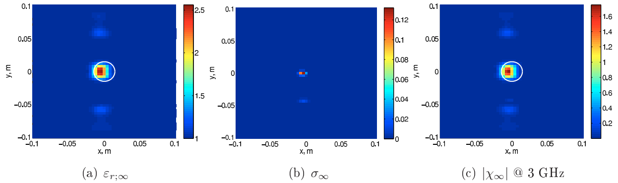
FIGURE 3.42: Inversion of the configuration in FIG. 3.31(c). Full data. Synthetic results ( \varepsilon_r=2 ).
