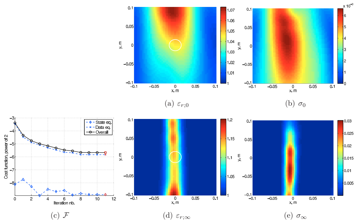
FIGURE 3.33: Inversion of the transmission configuration in FIG. 3.31(c). Experimental results.
