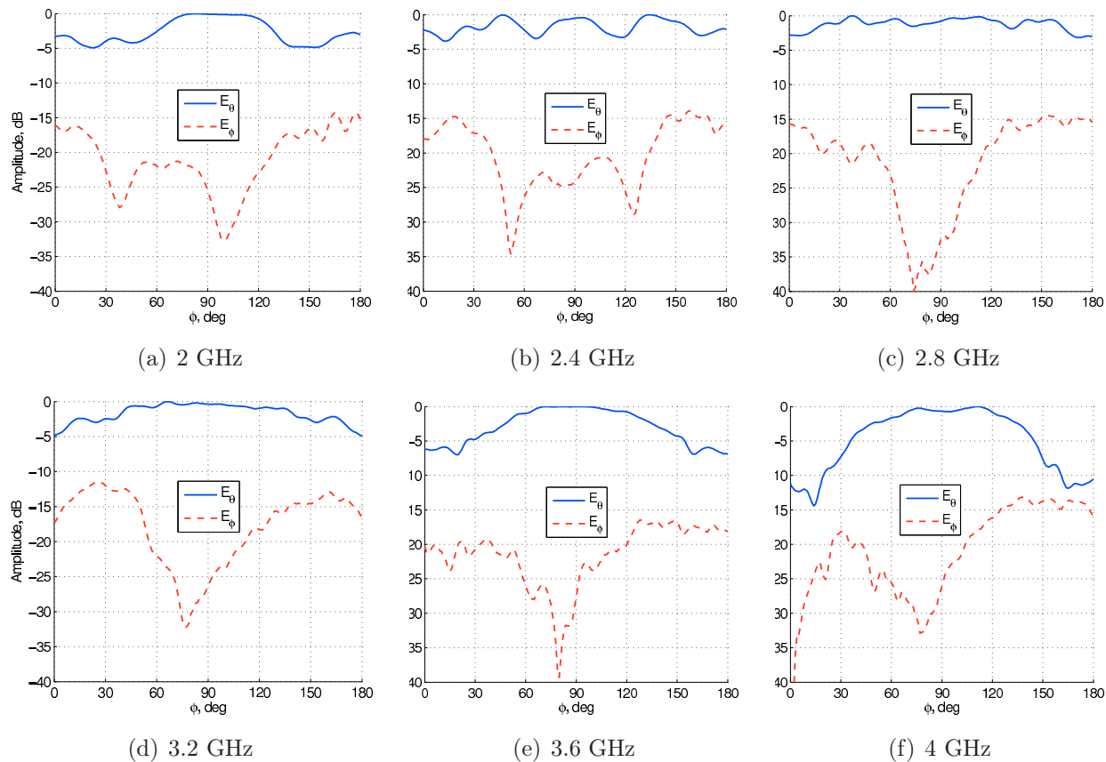
FIGURE 1.20: H -plane far-field radiation patterns of the ETS antennas measured at LEAT in Sophia Antipolis.
