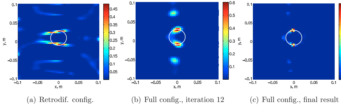
FIGURE 3.36: Inversion results with synthetic data. d_{\text{pix}}/\delta_\infty @ 3 \text{ GHz} .
