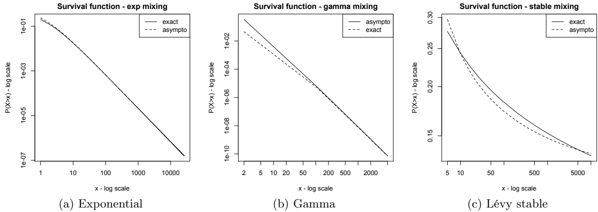
Figure 4.1: Survival functions
