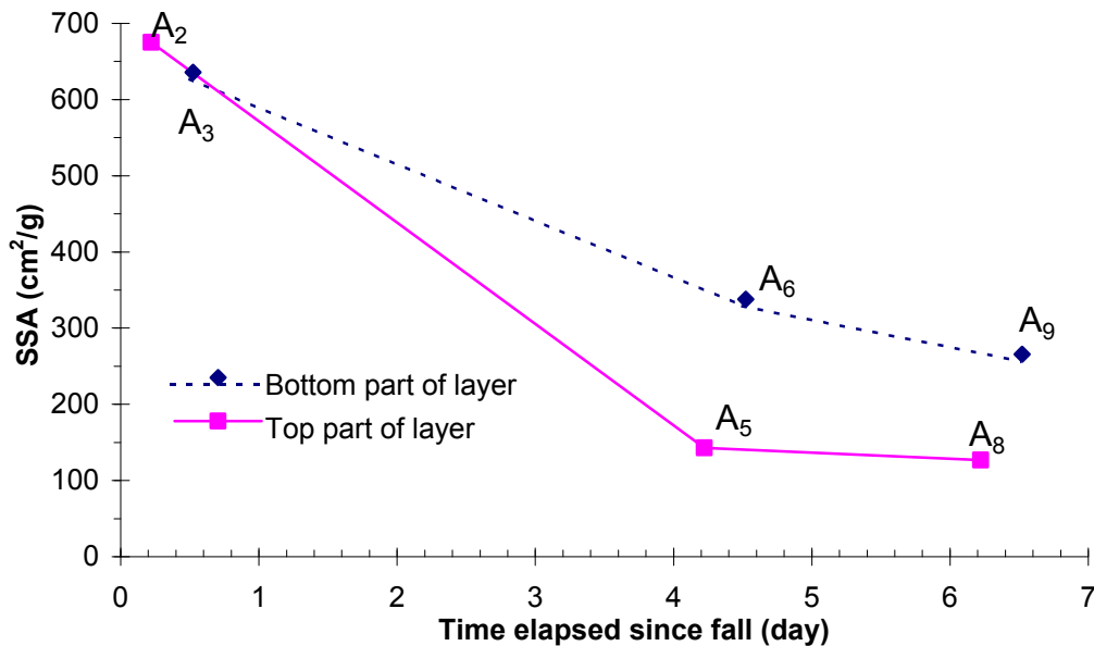
Figure 6: Time-evolution of the SSA of the top part (sequence A 2 , A 5 , A 8 ) and bottom part (sequence A 3 , A 6 , A 9 ) of layer A.
