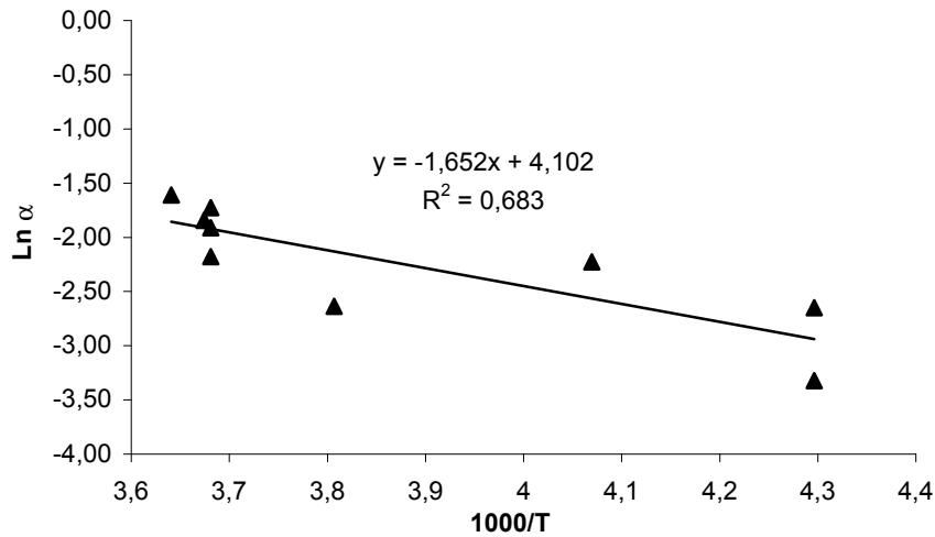
Figure 13: Evolution of the parameter \alpha_{exp} as a function of 1/T . Values of \alpha_{exp} are summed up in table 5. The 25-28 April 00 snow layer affected by wind has not been included in the data.
