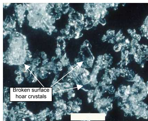
Figure 3: Photomicrograph of snow collected on 22 February during the wind storm. Scale bar: 1 mm.
