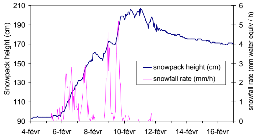
Figure 2: Snowpack height and snowfall rate at col de Porte in early February 1999. Time is GMT.
