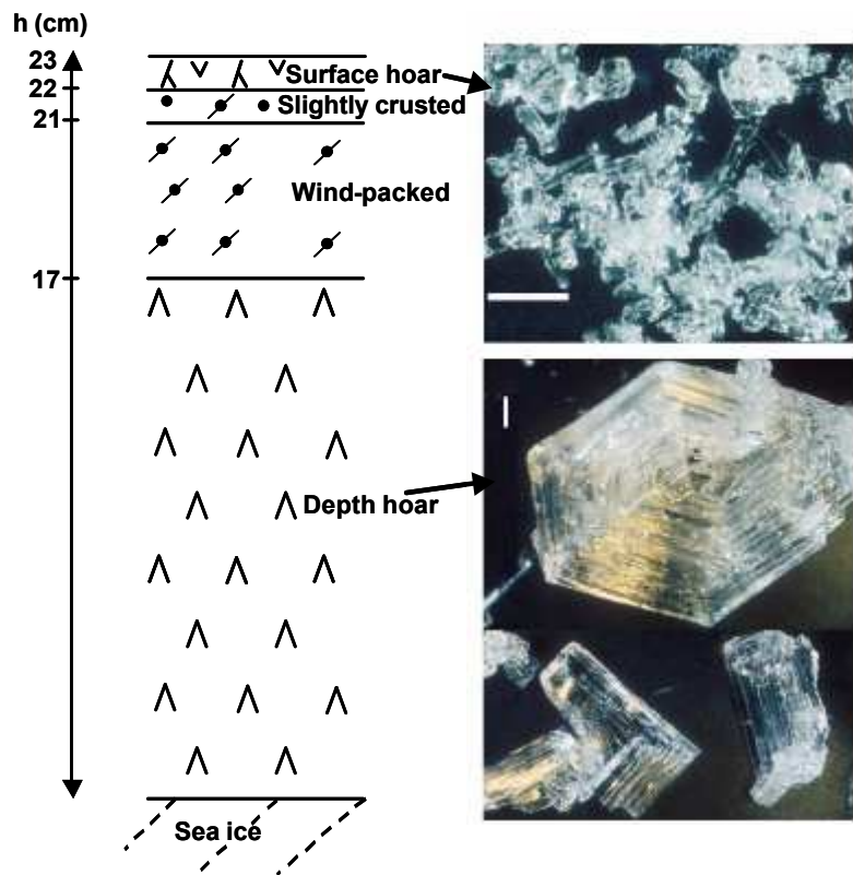
Figure 6: . Example of snowpack stratigraphy on the Arctic ocean (85°N) on 25 April 2000, with macrophotographs of snow crystals. All scale bars : 1 mm.
