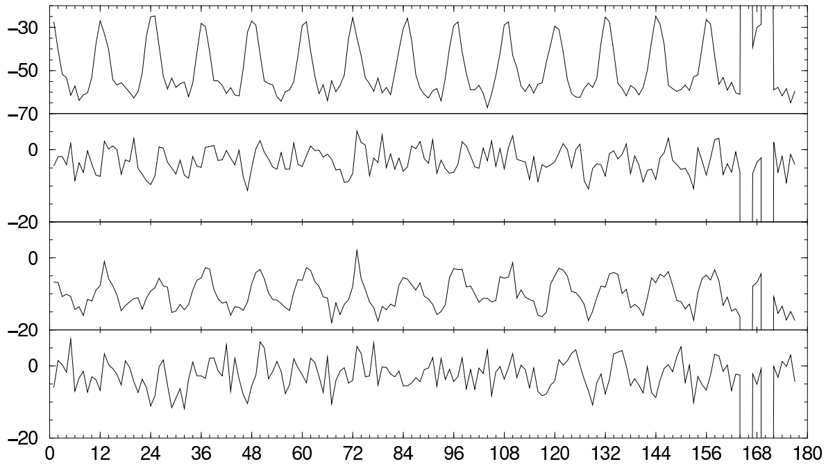
FIG. 3.10 – Time series of surface temperature at South Pole, in °C. From top to bottom : MWS (Amundsen Scott, SP) observations ; Nudged model minus MWS ; Reanalyses minus MWS ; Free model minus MWS. Values outside scale reveal missing observations.
