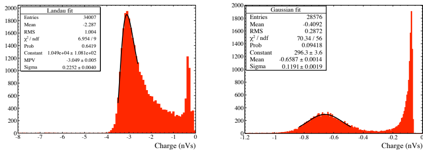
FIGURE 7.6: Example of two measured charge spectra for alphas emitted by an ^{241}\text{Am} with two different distances of air : (left) 0.9 mm of air ; (right) 25 mm of air.
