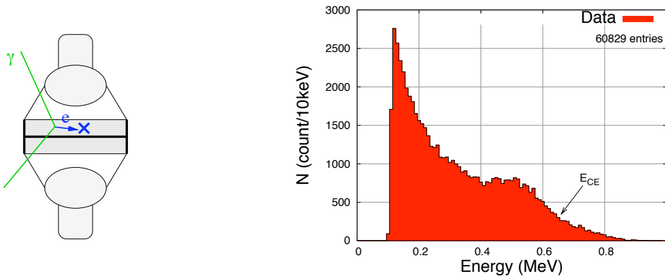
FIGURE 8.7: Energy calibration with a ^{54}\text{Mn} source : (left) showing the principle of the method and (right) an example of the energy spectrum obtained with a scintillator.
