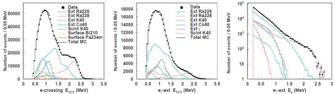
FIGURE 2.14: Result of the fit of the external background model to the observed data (black dots) of the Phase 2 data, for the whole detector : (left) energy sum of crossing electrons, (center) energy sum of the electron and \gamma for external ( e^- , \gamma ) events and (right) detected energy of the electron for external ( e^- , \gamma ) events.
