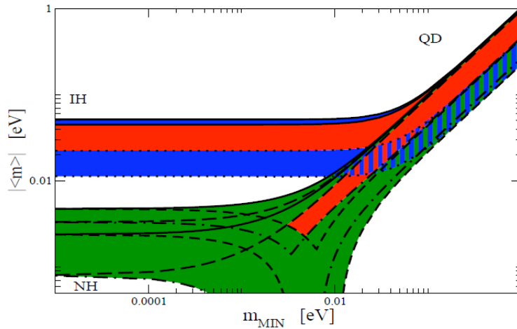
FIGURE 1.5: The predicted value of \langle m_{ee} \rangle as a function of m_{\text{min}} , obtained using the 2\sigma allowed ranges of \Delta m_{\text{atm}}^2 , \Delta m_{\odot}^2 , \sin^2 \theta_{\odot}^2 and \sin^2 \theta_{13}^2 . The regions shown in red correspond to violation of CP-symmetry while the rest of the regions correspond to the four different sets of CP-conserving values of the two Majorana phases with the green region for normal hierarchy and blue region for inverted hierarchy.
