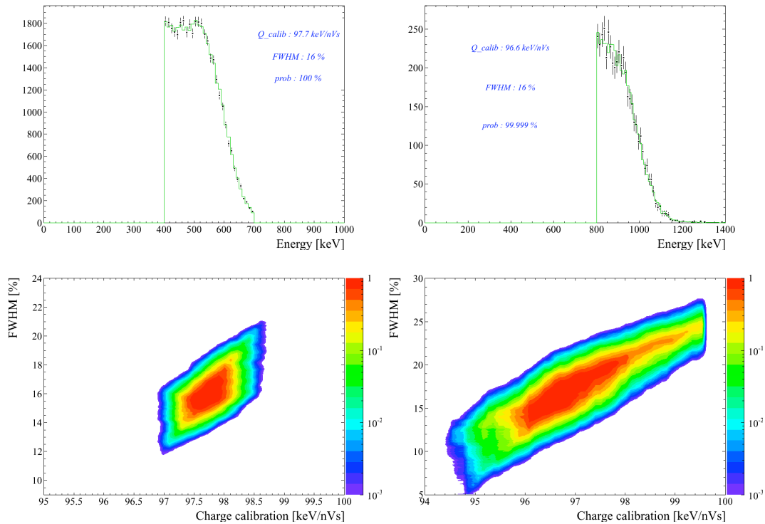
FIGURE 11.14: Energy spectrum of the Compton edge measured with ^{54}\text{Mn} (upper left) and ^{22}\text{Na} (upper right) and result of the Monte-Carlo fit; (Lower plots) Allowed region for the most probable values of the energy calibration and energy resolutions obtained with ^{54}\text{Mn} (left) and ^{22}\text{Na} (right).
