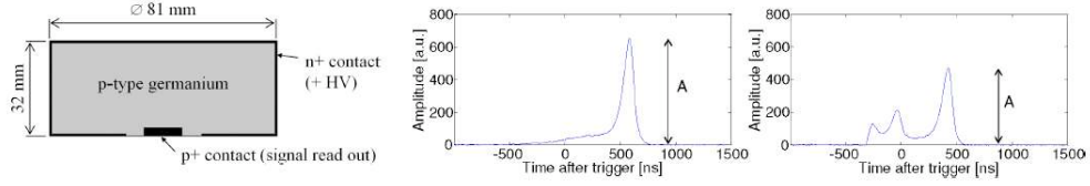
FIGURE 3.6: (Left) Schematic view of a point-contact Broad Energy Germanium (BEGe); (Center) Single Site Event ( \beta\beta\nu topology); (Right) Multi Site Event (Multi Compton background topology)
