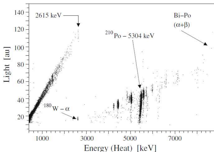
FIGURE 4.8: Result of a background measurement performed with a 3\times 3\times 6 cm 3 CdWO 4 crystal (426 g) during 1066 hours. No \beta/\gamma events have been observed above the 2615 keV ^{208}\text{Tl} line.
