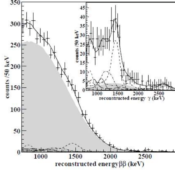
FIGURE 5.5: Energy distributions from 752.66 hrs of EXO-200 single-cluster events (main panel) and multi-cluster events (inset). The result of the fit (solid line) contains \beta\beta 2\nu -decay (shaded region) and prominent background components of the TPC vessel.
