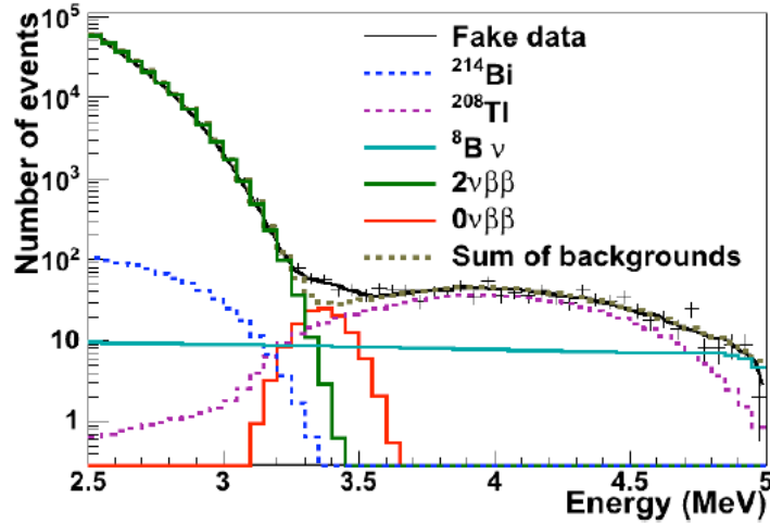
FIGURE 5.3: Simulated event energy spectrum showing the expected backgrounds and \beta\beta\nu signal (assuming T_{1/2}^{0\nu} = 10^{24} yrs) for a 3 years run with 0.1% Nd-loading.
