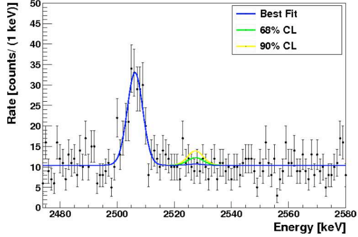
FIGURE 4.2: Energy spectrum in the \beta\beta\nu region [65]
