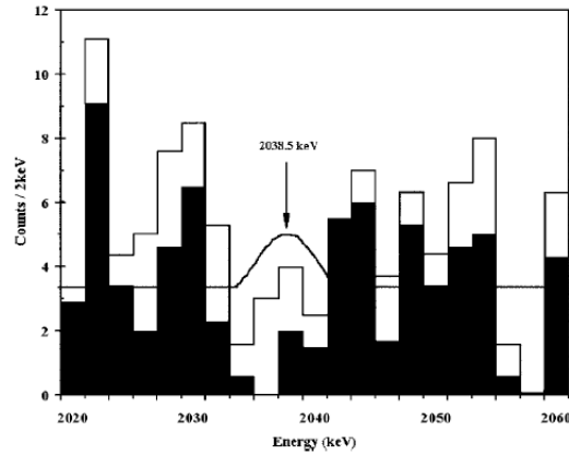
FIGURE 3.2: Energy spectrum measured by the IGEX experiment with 8.87 kg.y of ^{76}\text{Ge} exposure. The darkened spectrum results from the application of PSD to \approx 45\% of the total data set. The Gaussian curve represents the 90% C.L. excluded \beta\beta 0\nu signal [50].
