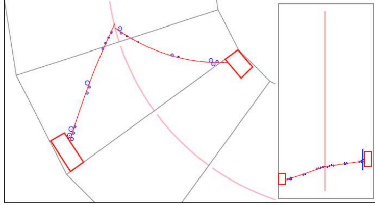
FIGURE 2.4: Transverse (left) and longitudinal (right) view of a reconstructed \beta\beta\nu candidate event selected from the data with a two-electron energy sum of 2812 keV.
