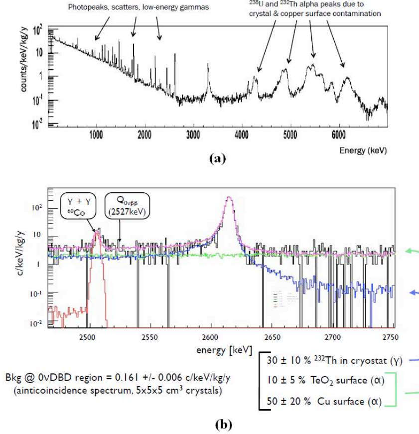
FIGURE 4.3: (a) Energy spectrum in the full energy range; (b) Energy spectrum in the \beta\beta\nu region and fitted Monte-Carlo background model.
