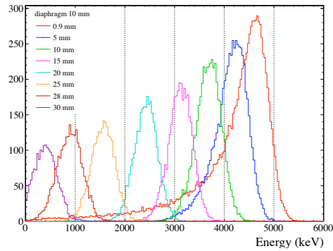
FIGURE 7.5: Expected charge spectrum deposited in the polystyren scintillator by \alpha particles emitted by ^{241}\text{Am} , and crossing different distances of air, calculated by GEANT4 simulation.
