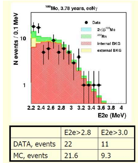
FIGURE 2.20: Sum energy spectrum of the two electrons using (e^-e^-, N\gamma) channel from ^{100}\text{Mo} , with 3.78 years of collected data in Phase 2 and expected background from Monte-Carlo simulation.
