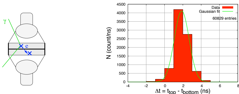
FIGURE 8.8: Time calibration with a ^{54}\text{Mn} source : (left) showing the principle of the method and (right) an example of the time distribution obtained with one module.
