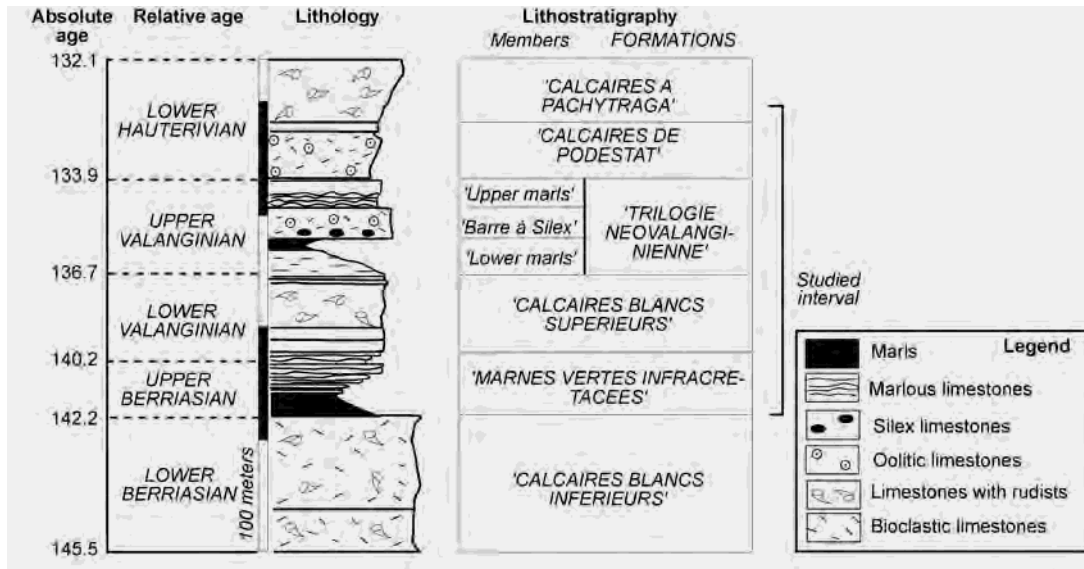
Figure 3. Lithostratigraphy and chronostratigraphy proposed for the Berriasian-Hauterivian interval and its relative datation (modified from Virgone, 1997). Absolute ages are from the Ogg et al. (2008) timescale.
