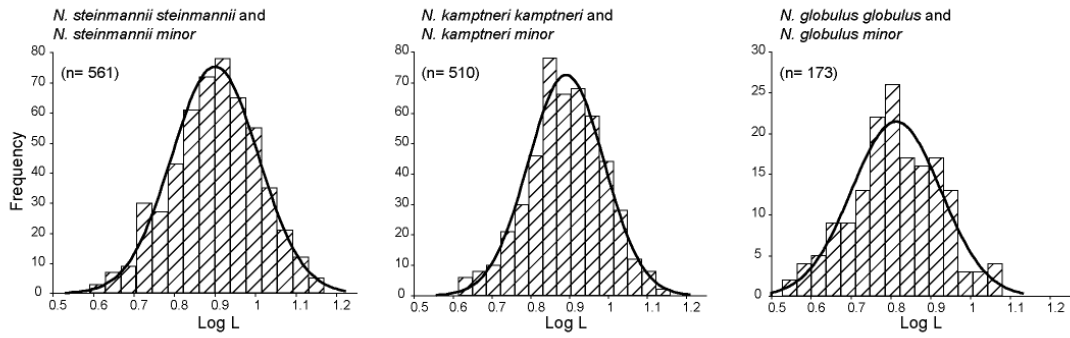
Figure 6. Frequency distribution of the length values (Log L) for N. steinmannii , N. kamptneri and N. globulus . Mixture analysis indicates a single normal distribution (black curves).
