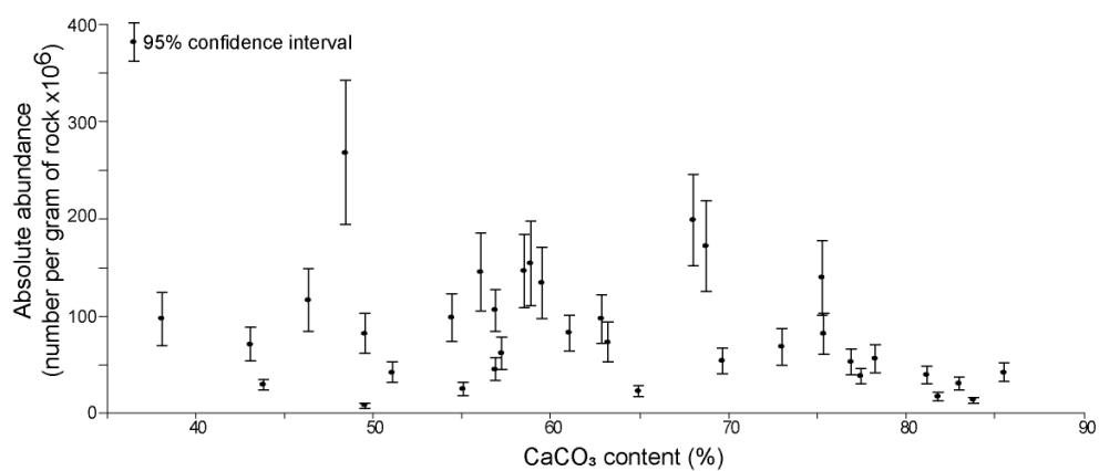
Figure 5. Absolute abundance of nannoconid plotted against the calcium carbonate percentage.
