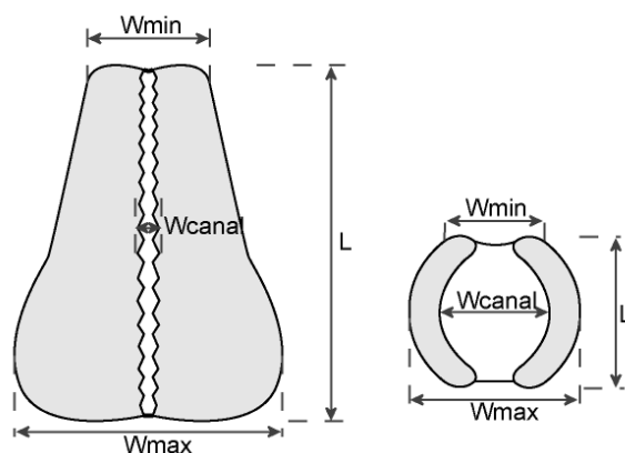
Figure 2. Descriptive variables of Nannoconus . Here N. steinmannii (left) and N. globulus (right) are shown as examples. Abbreviations: Wmin = minimal width, Wmax = maximal width, Wcanal = width of the central canal and L = length.
