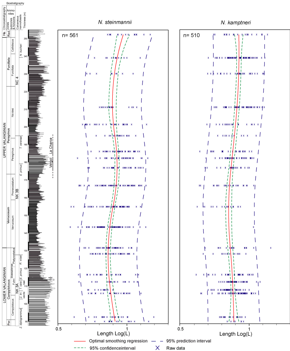
Figure 7. Stratigraphic distribution of the Length (L) of N. steinmannii and N. kamptneri . The penalized-spline regression shows significant stratigraphic trends for both species.
