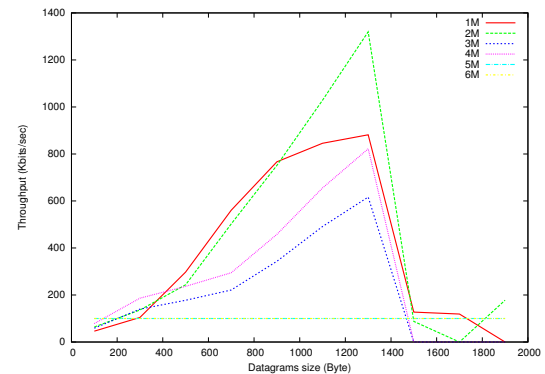
Figure 12.12: Throughput - multi-hop
