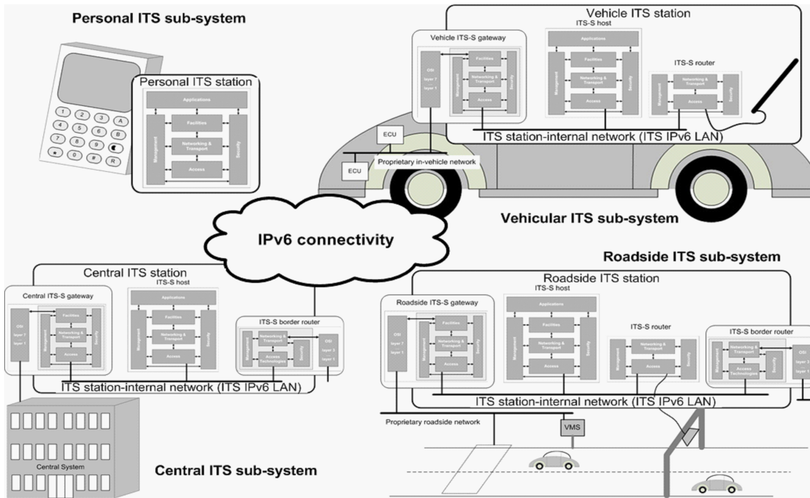
Figure 2.7: ITS sub-systems
