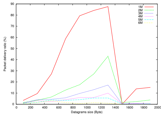
Figure 12.11: Packet delivery ratio - multi-hop
