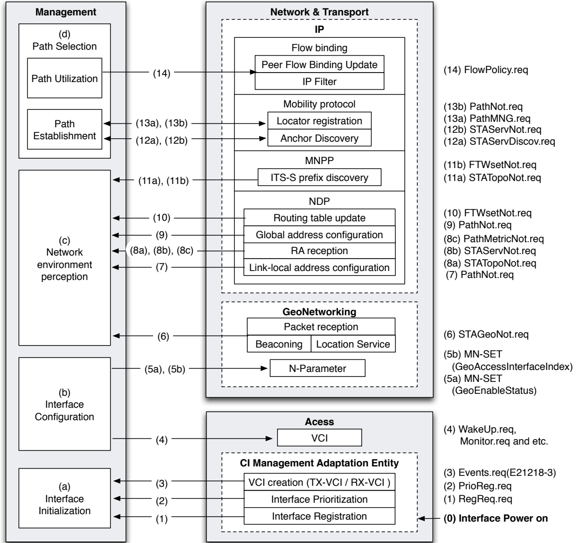
Figure 7.4: Procedure of Path Management
