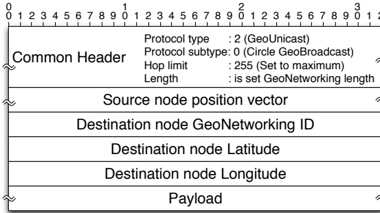
Figure 3.4: GeoUnicast packet
