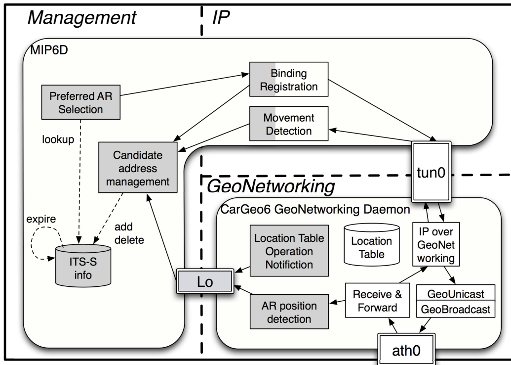
Figure 9.7: Overview of MIP6D implementation with MN-SAP
