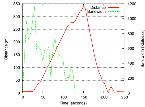
Figure 12.18: Throughput on TCP with distance
