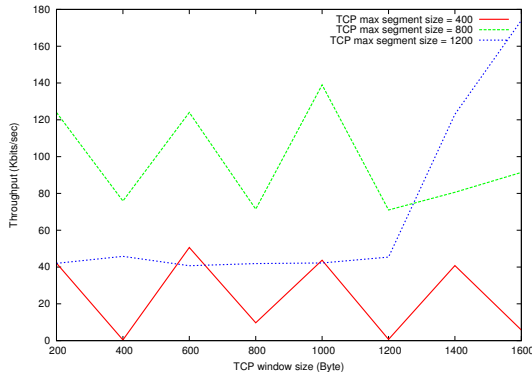
Figure 12.13: Single Hop Throughput with HITACHI
