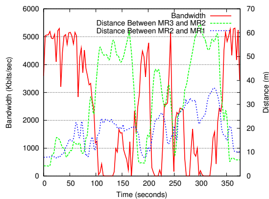
Figure 11.11: TCP highway test with 3 dynamic cars (bandwidth/distance)
