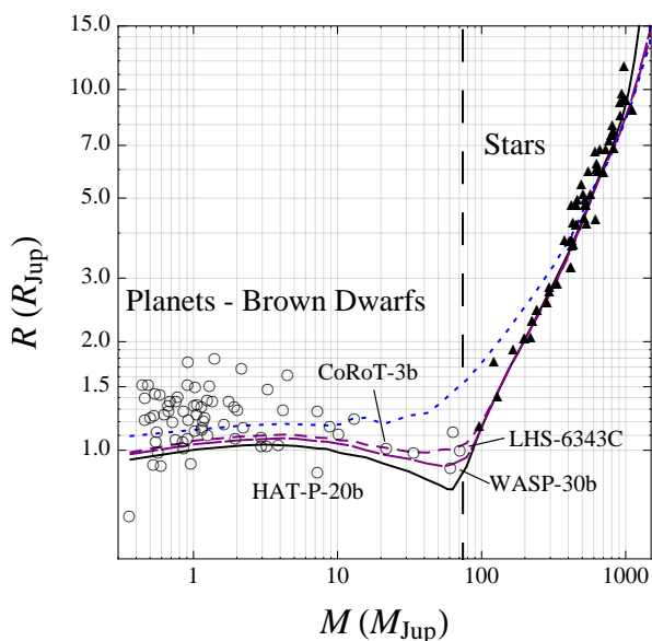
Figure 2.5: Mass-radius relationship of gaseous objects at 5 (solid), 1 (long dashed), 0.5 (dashed) and 0.1 Gyr (dotted). Observational data points are also shown.
