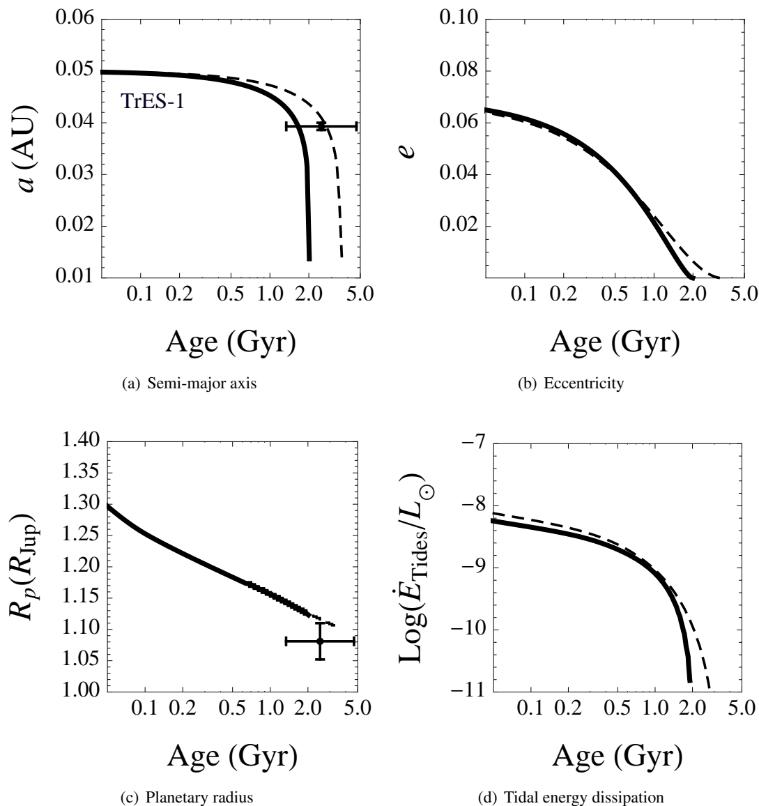
Figure 5.11: Consistent tidal/thermal evolution of TrES-1 b computed with our constant time-lag model ( solid line ) and with the " e^2 model" ( dashed line ). This is a 0.76 M_{\text{Jup}} planet orbiting a 0.89 M_{\odot} star (Winn et al. 2007a). The error bars are the measured parameters with the 1\sigma uncertainty. The dashed curve is comparable to Fig. 7 of Miller et al. (2009) and was computed with the same parameters ( Q'_p = 10^{6.5} , Q'_* = 10^5 ). As expected, in the low e limit the tidal dissipation rate is well approximated by Eq. (5.32) and the two models yield similar evolutions, although the merging time depends on the rheology used. Figure from Leconte et al. (2010a).
