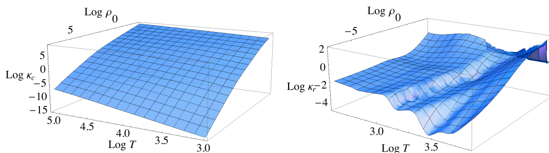
Figure 1.1: Left: Conductive opacities ( \kappa_c in \text{m}^2.\text{kg}^{-1} ) from Potekhin et al. (1999) as a function of density (in \text{kg}.\text{m}^{-3} ) and temperature (in K). Right: Decimal logarithm of the COND Rosseland radiative opacities ( \kappa_r in \text{m}^2.\text{kg}^{-1} ) from Ferguson et al. (2005) as a function of density (in \text{kg}.\text{m}^{-3} ) and temperature (in K).
