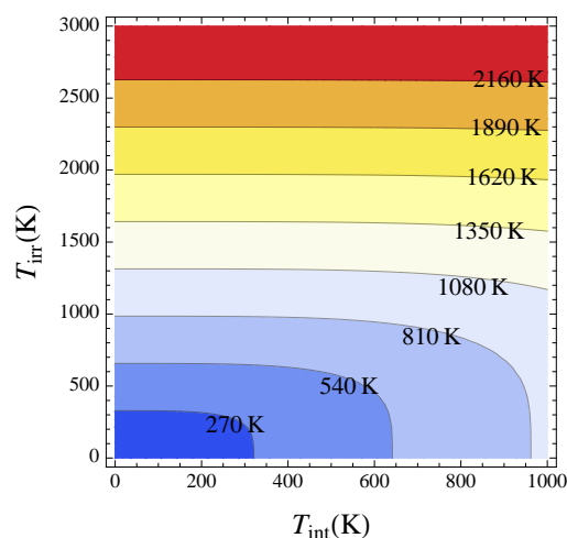
Figure 1.4: Atmospheric boundary temperature ( T_{\text{atm}} ; Eq. (1.97)) at the 10 bar level ( P_{\text{atm}} = 10 bar) as a function of the internal flux (parametrized by T_{\text{int}} ) and incoming stellar flux (parametrized by T_{\text{irr}} ) for a redistribution factor \bar{f} = (2\sqrt{3})^{-1} (see text).
