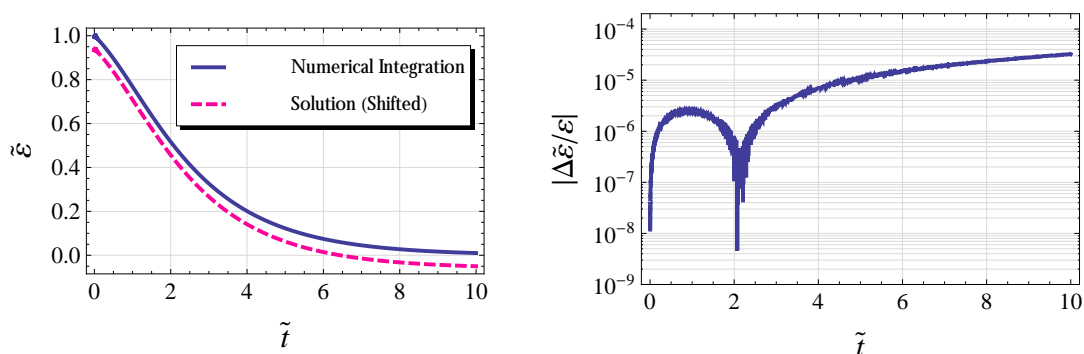
Figure 5.4: Left: Comparison between the exact solution given by Eq. (5.28) for the obliquity of the planet and the numerical integration of the full set of equations. The exact solution has been shifted to be visible. As predicted the planet pseudo synchronizes and its obliquity is damped to 0. Right: Relative error between the exact solution and the numerical integration. The numerical integration yields correct results down to 10^{-5} . The peculiar behavior of the error is due to the fact that the solution is not convex: the sign of the error changes.
