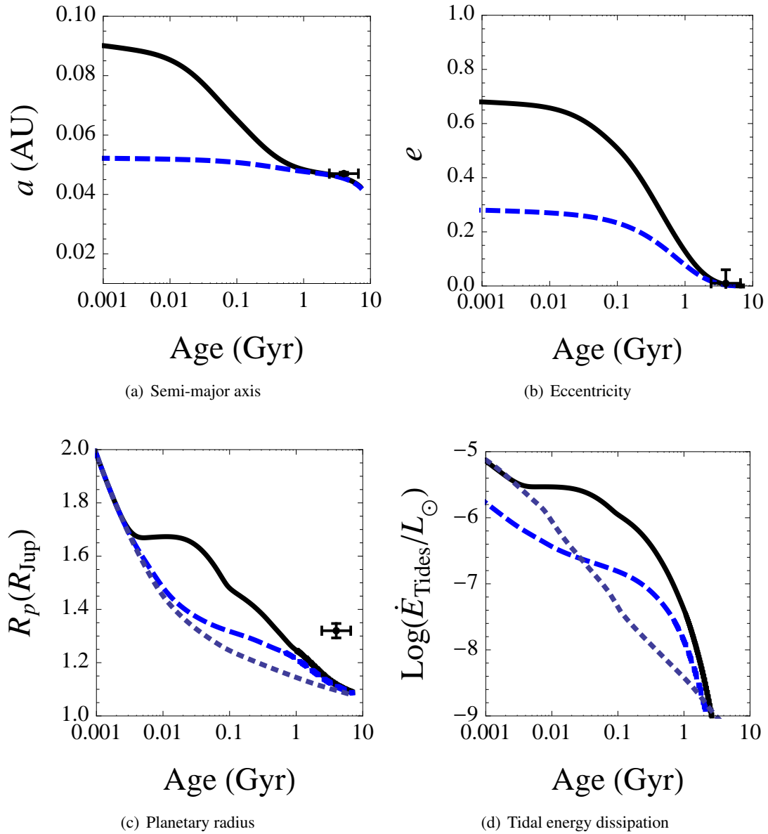
Figure 5.13: Consistent tidal/thermal evolution of HD 209 458 b with different initial conditions (solid and dashed) computed with our constant time-lag model. HD 209 458 b is a 0.657 M_{\text{Jup}} planet orbiting a 1.01 M_{\odot} star (Knutson et al. 2007). These runs assume Q'_{0,p} = 10^6 and Q'_{0,*} = 10^6 . For comparison, the radius and luminosity of an isolated planet (no tidal heating) is shown on the lower panels (dotted curves). Even though these evolutions recover the presently observed orbital parameters for the system, the eccentricity damping arises too early during the evolution, leading to insufficient tidal dissipation at present epoch to explain the inflated radius. Figure from Leconte et al. (2010a).
