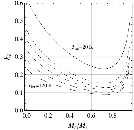
Figure 3.3: Love number as a function of the core mass for a 11 M_{\oplus} planet, for various effective temperature ( T_{\text{int}} from 20 to 120 K by steps of 20 K ; more and more spaced dashing).
