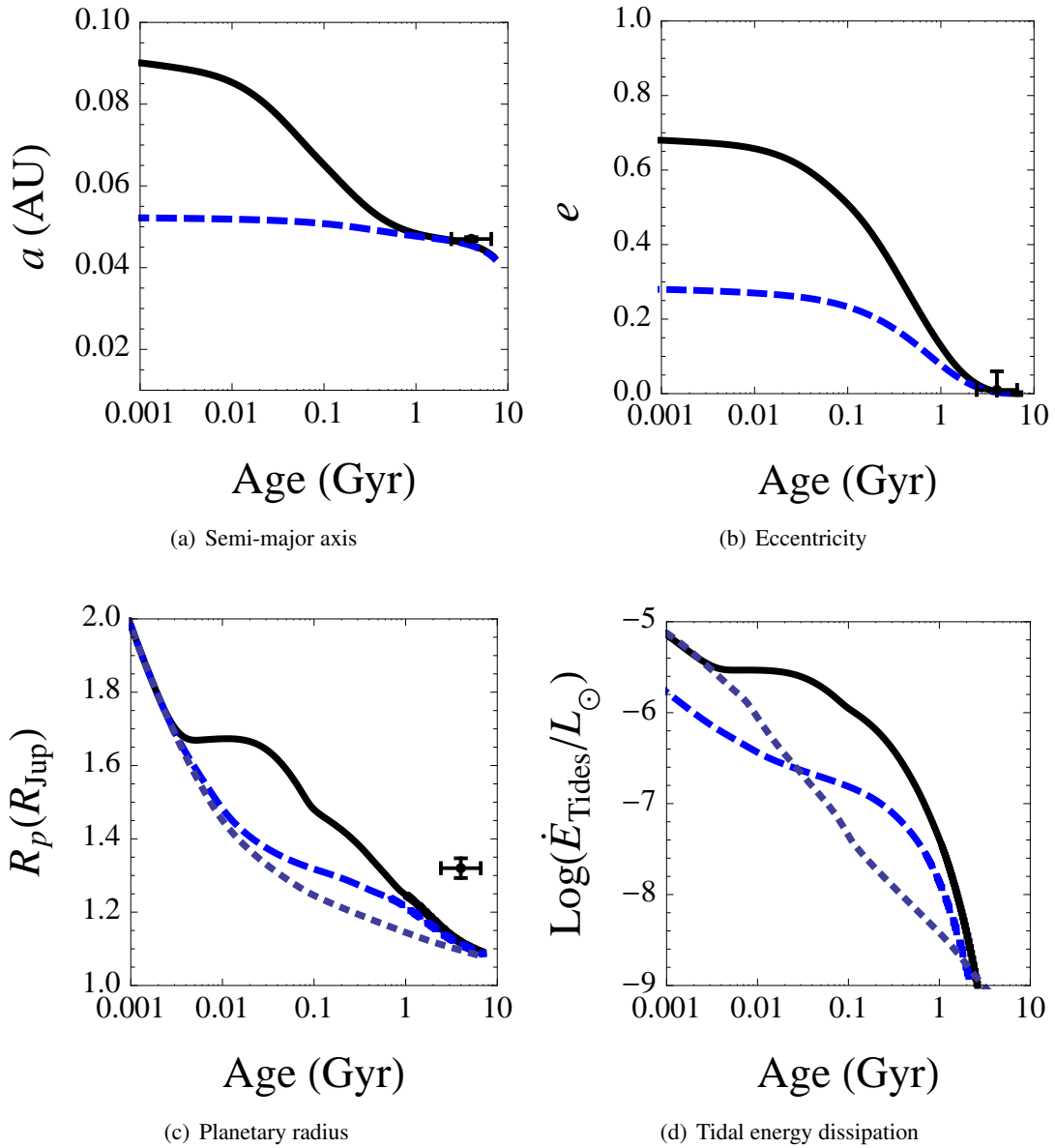
Figure 5.13: Consistent tidal/thermal evolution of HD 209 458 b with different initial conditions (solid and dashed) computed with our constant time-lag model. HD 209 458 b is a 0.657 M_{Jup} planet orbiting a 1.01 M_{\odot} star (Knutson et al. 2007). These runs assume Q'_{0,p} = 10^6 and Q'_{0,*} = 10^6 . For comparison, the radius and luminosity of an isolated planet (no tidal heating) is shown on the lower panels (dotted curves). Even though these evolutions recover the presently observed orbital parameters for the system, the eccentricity damping arises too early during the evolution, leading to insufficient tidal dissipation at present epoch to explain the inflated radius. Figure from Leconte et al. (2010a).
