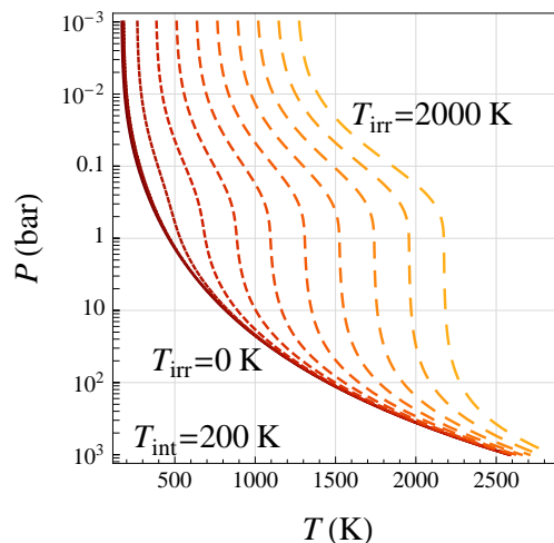
Figure 2.8: Atmospheric T - P profile computed with Eq. (1.96) for a Jupiter analog with T_{\text{int}} = 200 K and T_{\text{irr}} varying between 0 K (black solid) and 2000 K (yellow dashed) by steps of 200 K. For this example, \kappa_{\text{vis}} = 10^{-3} \text{m}^2 \cdot \text{kg}^{-1} and \kappa_{\text{th}} = 10^{-2} \text{m}^2 \cdot \text{kg}^{-1} (see § 1.5.2).
