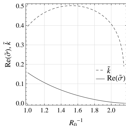
Figure 4.2: Dimensionless wavenumber ( \tilde{k} ; dashed) and growth rate ( \text{Re}(\tilde{\sigma}) ; solid) of the fastest growing overstable mode with respect to the inverse density ratio ( R_0^{-1} ). The length scale of the fastest growing mode is about 12d .
