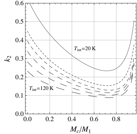
Figure 3.3: Love number as a function of the core mass for a 11 M_{\oplus} planet, for various effective temperature ( T_{\text{int}} from 20 to 120 K by steps of 20 K ; more and more spaced dashing).
